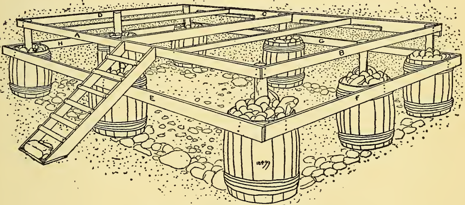
FIG. 88.—A Finished Foundation.
