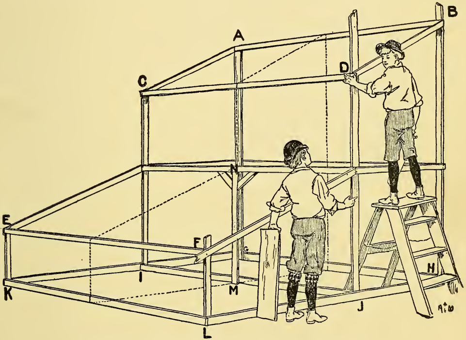
FIG. 31.—Frame of Bantam-Coop and Pigeon-Loft.
