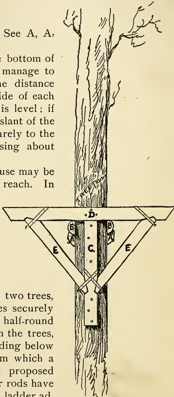
FIG. 3.—End View of Corbel Resting on B Sticks.
