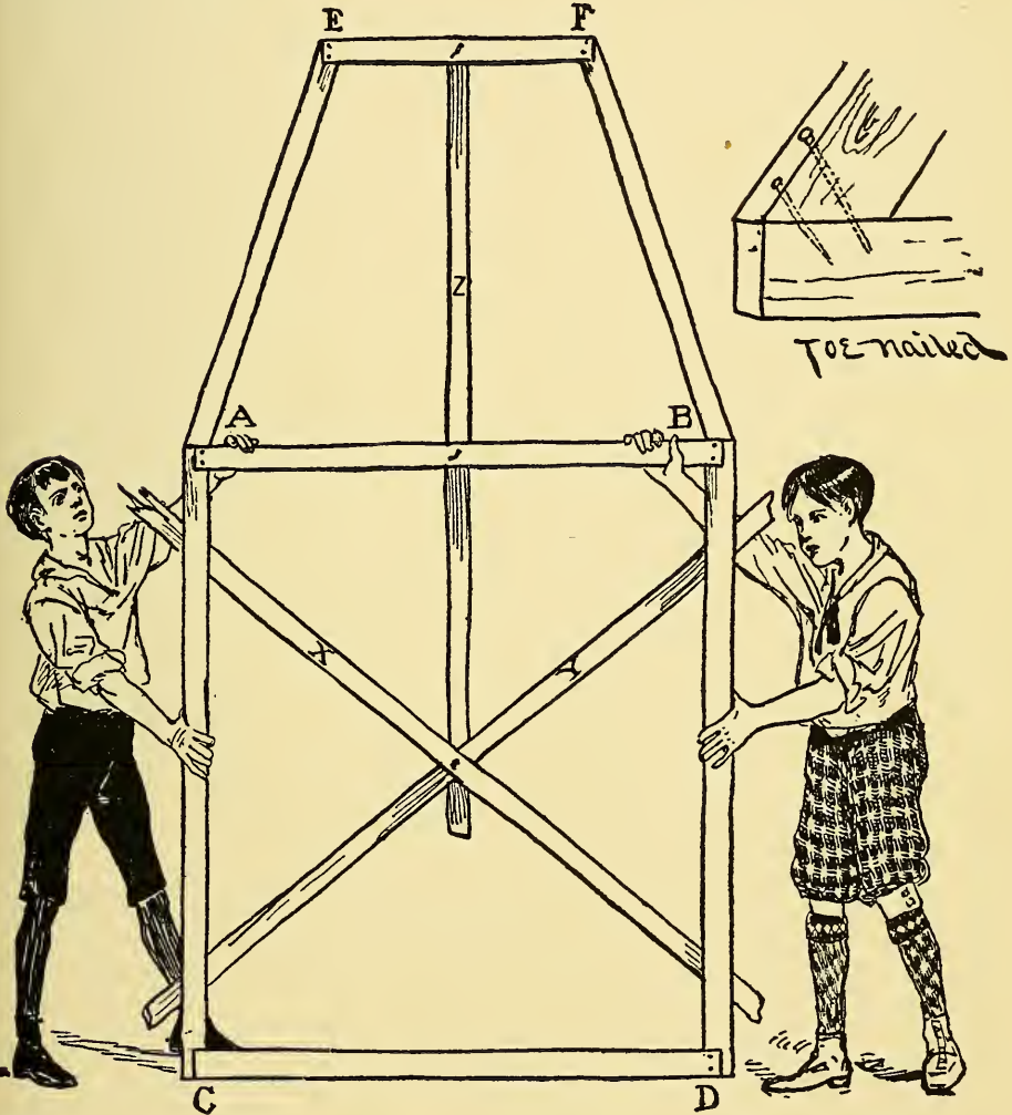
FIG. 254.—The Back of the Chimney.
