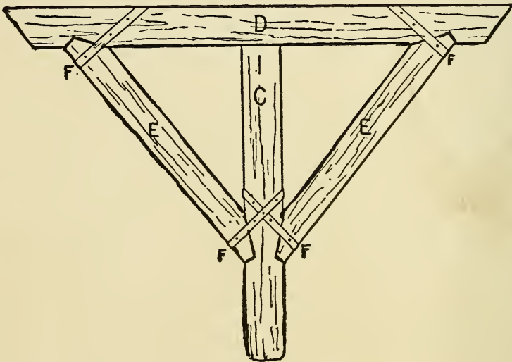
FIG. 2.—King Posts and Corbel.
