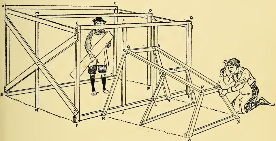
FIG. 77.—The Frame.
