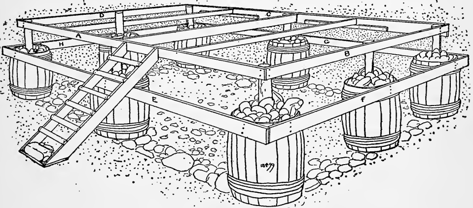
FIG. 88.—A Finished Foundation.
