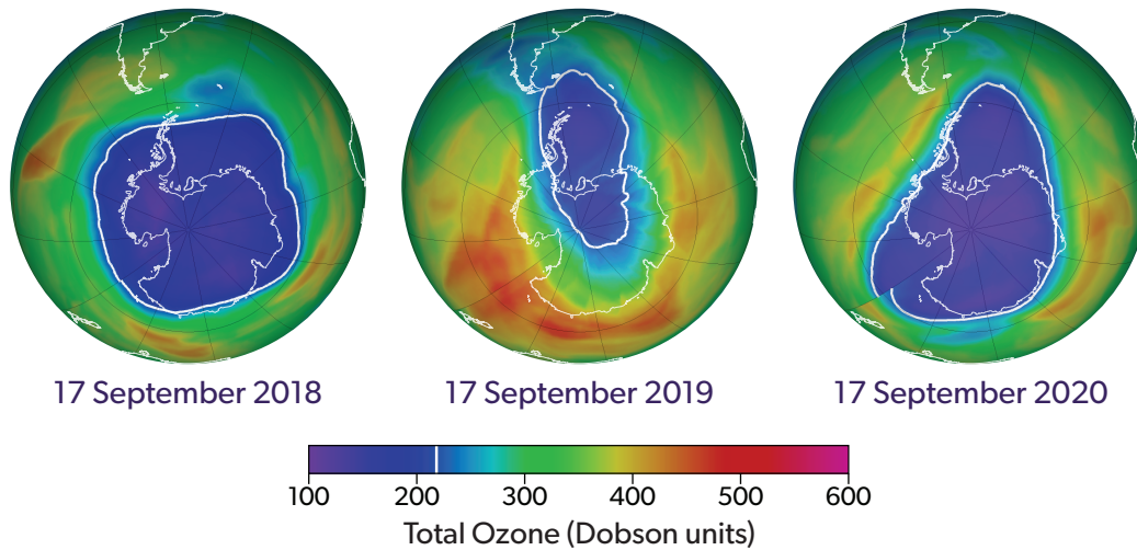
Figure Q10-4. Unusual 2019 ozone hole. Views from space of the Antarctic ozone hole are shown for 17 September for three consecutive years: 2018, 2019, and 2020. The ozone holes in 2018 and 2020 are considered typical of those observed since the late 1990s. An initially circular hole in 2019 was transformed by the significant transport of air from midlatitudes into the region of the ozone hole starting in late August. This unusual event, initiated by meteorological disturbances in the midlatitude troposphere, transported high amounts of ozone from midlatitudes into the region of the ozone hole and led to higher temperatures that reduced the rate of ozone depletion in 2019 compared to most other years. Consequently, the region of low total ozone in 2019 was displaced from the normal circumpolar position, and the amount of ozone depletion in 2019 as measured by the area of the ozone hole or minimum total ozone amounts was much less than in either 2018 or 2020 (see Figure Q10-2).
