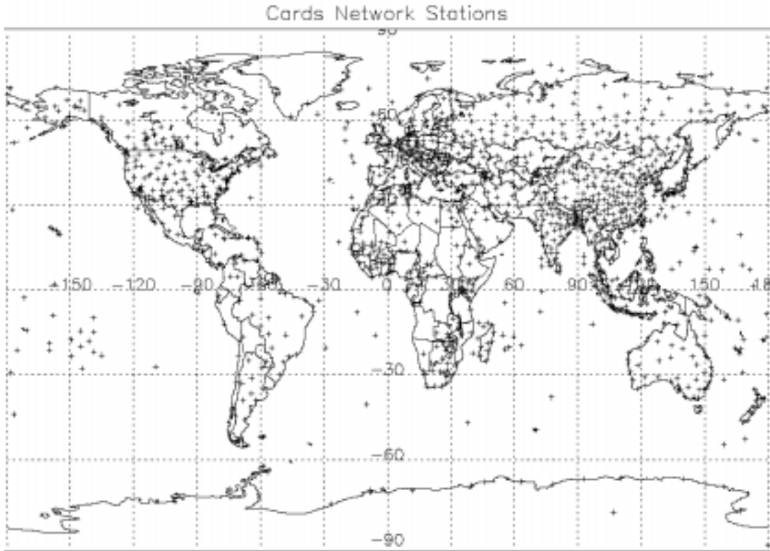
Fig. 5.2. CARDS Network of meteorological sonde sites.
