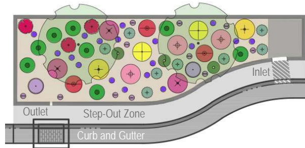
FIGURE 20. Western Prairie Planting Plan (Source: Stream Design, 2015.) Scale: 1" = 10'
