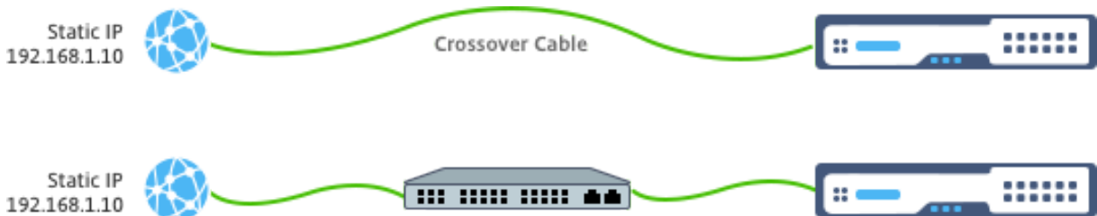
Figure. Initial Configuration of LOM Module
