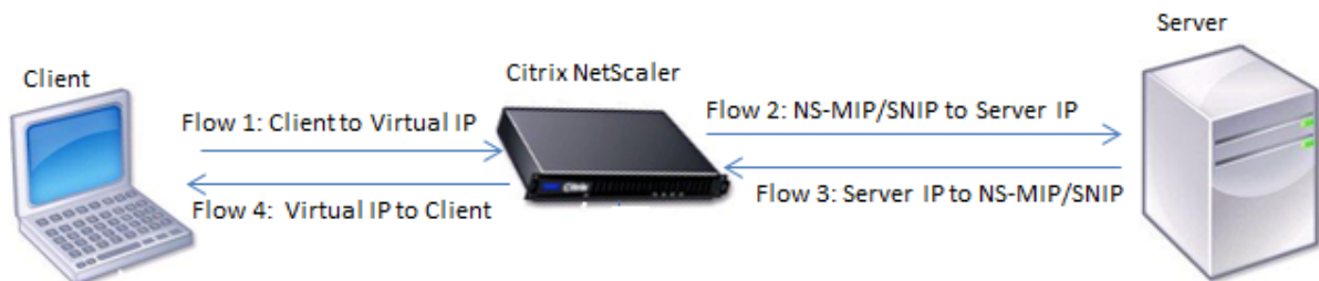
Figure 1. Citrix ADC Flow Sequence
