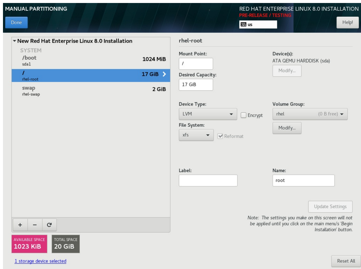
Figure 16.1. Customizing Partitions
