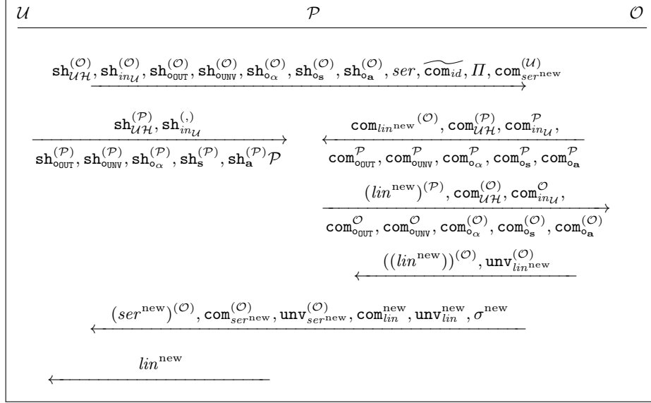
Fig. 32: Message overview for \pi -Outsource.
