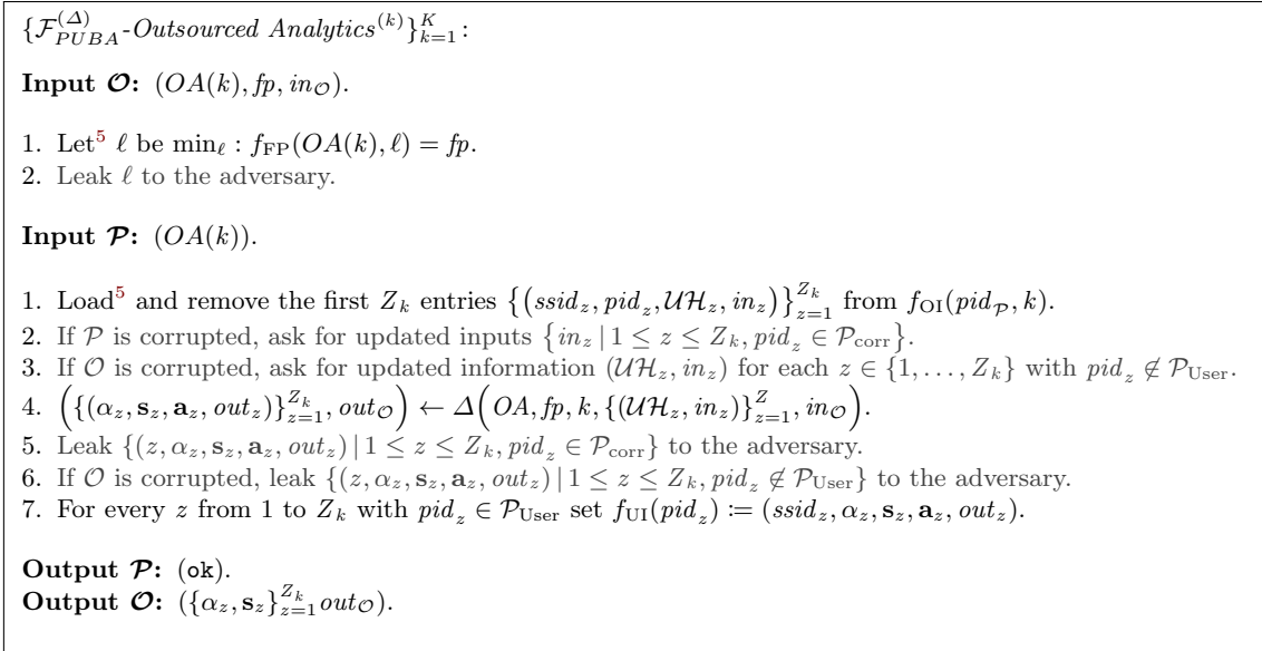
Fig. 12: Task \mathcal{F}_{PUBA}^{(\Delta)}\text{-Outsourced Analytics}^{(k)} for outsourced computation between the operator and the proxy of the task defined by k \in \{1, \dots, K\} .
