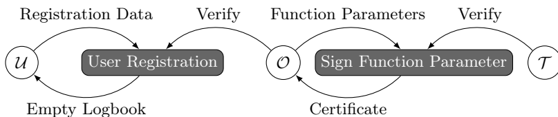
Fig. 1: Overview of the preparatory tasks.
