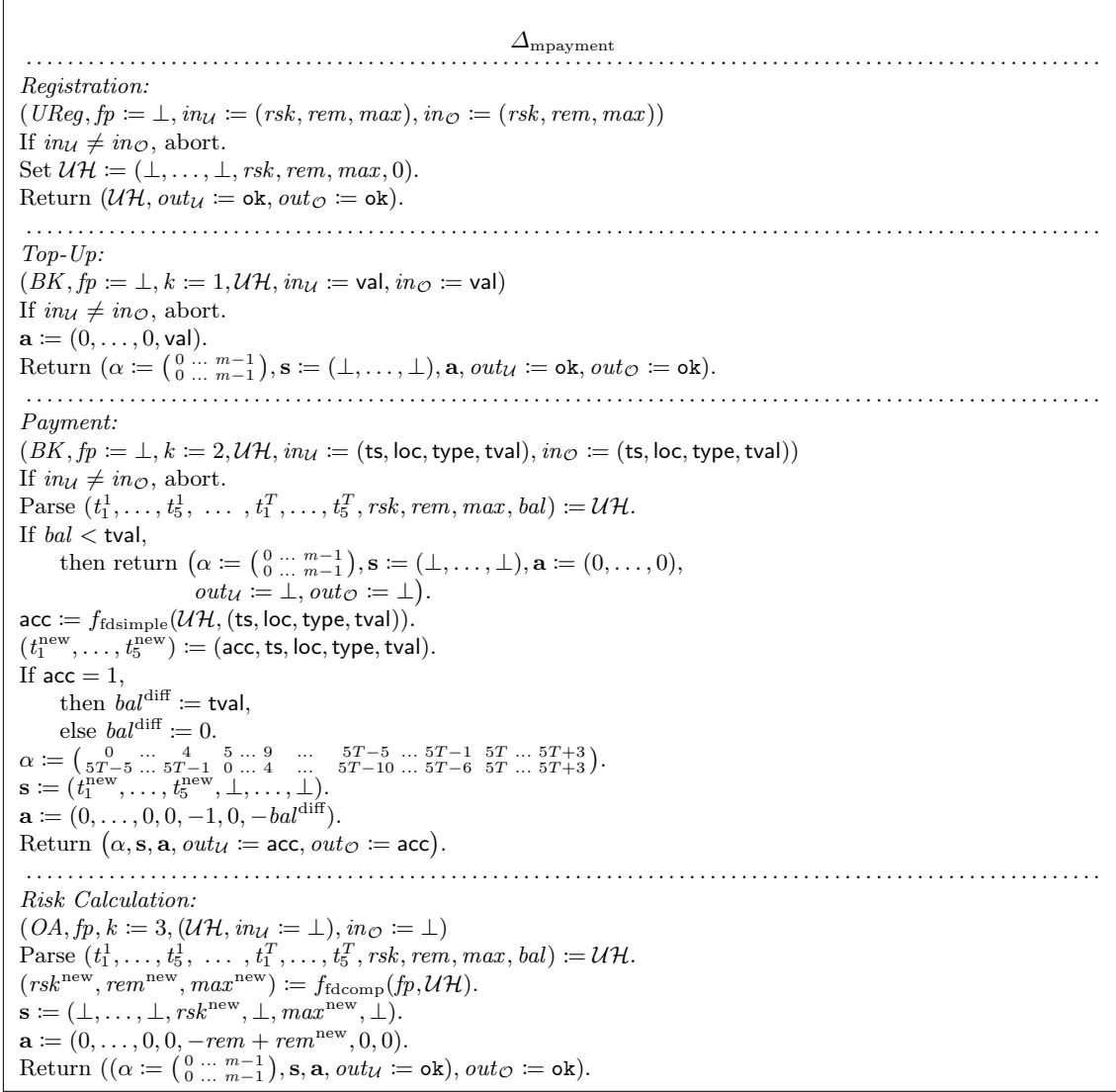
Fig. 39: Instantiation of \Delta for privacy-preserving mobile payments with fraud detection.
