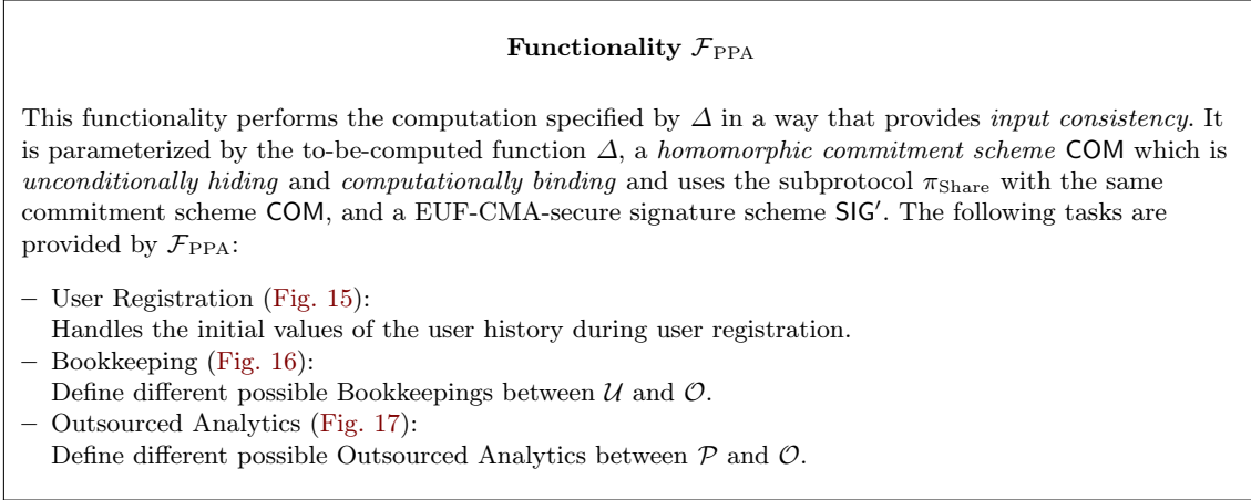
Fig. 14: The functionality \mathcal{F}_{\text{PPA}} we use to perform the computations.
