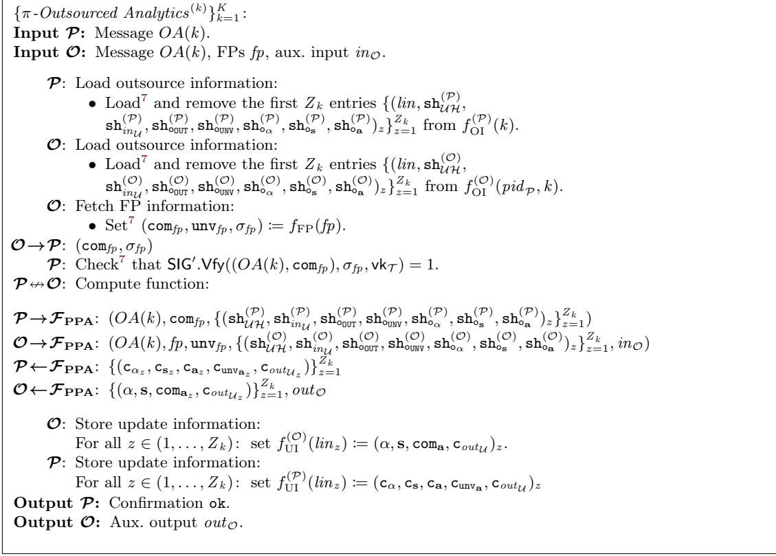
Fig. 34: The protocol \pi\text{-Outsourced Analytics} for the Outsourced Analytics-task (Fig. 12).
