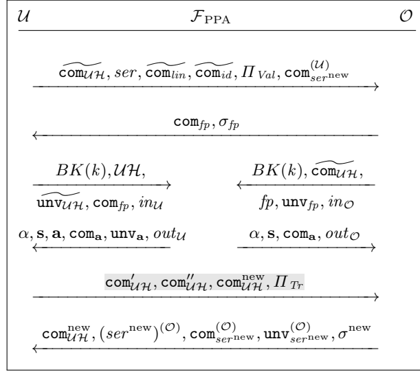
Fig. 28: Message overview for \pi -Bookkeeping (k) . The highlighted message is not always sent.
