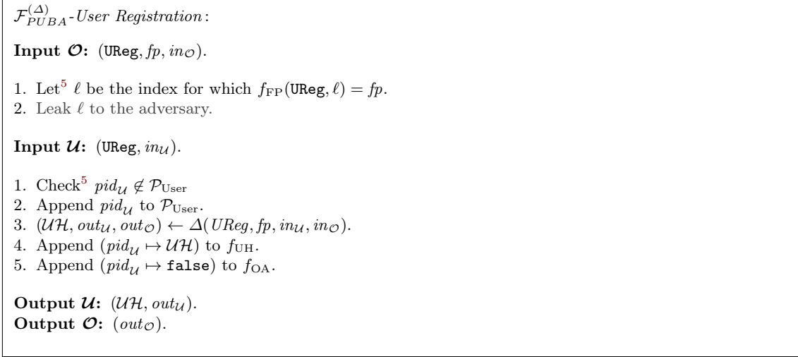
Fig. 9: Task \mathcal{F}_{PUBA}^{(\Delta)} -User Registration for registering a user.
