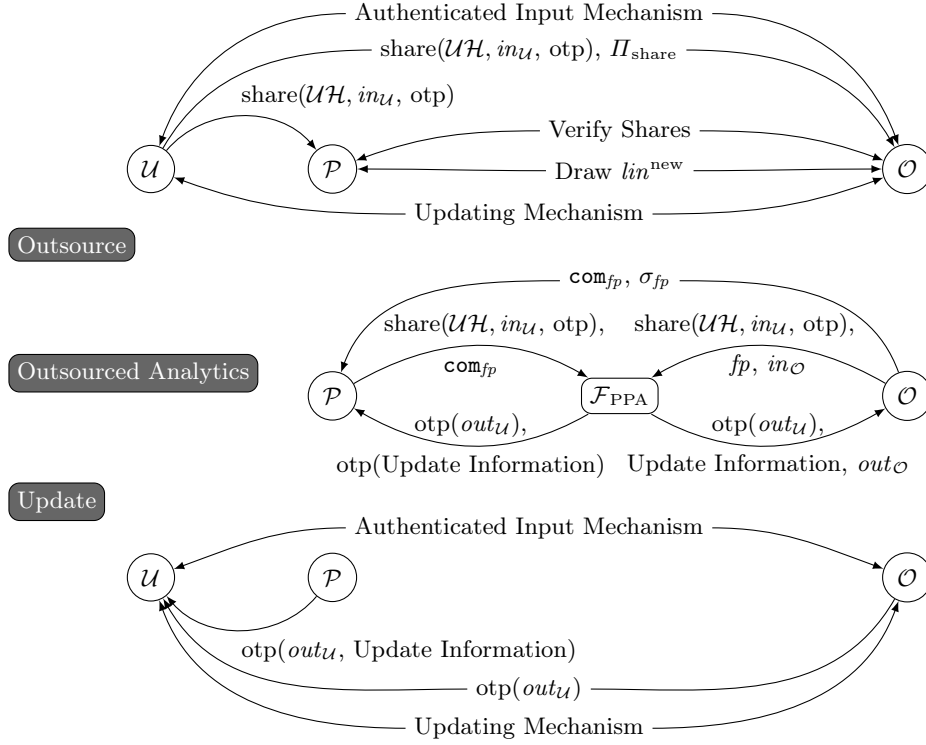
Fig. 5: Simplified depiction of \pi_{PUBA} for outsourcing computations.
