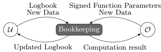
Fig. 2: Overview of the Bookkeeping task.
