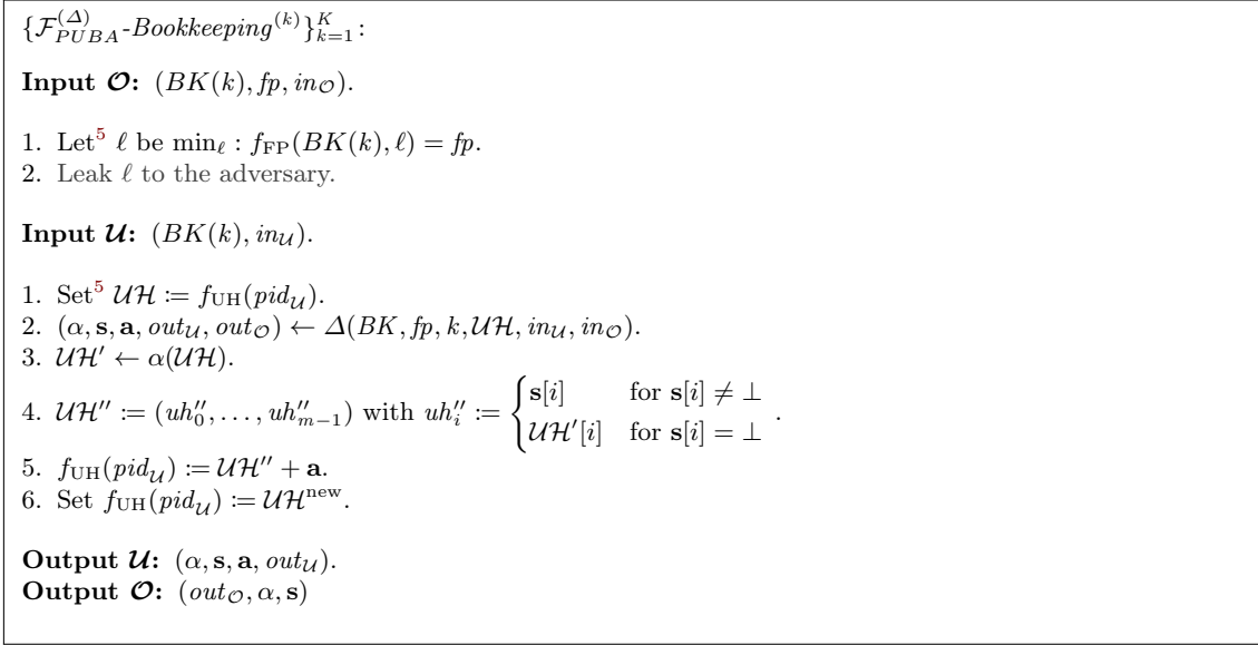
Fig. 10: Task \mathcal{F}_{PUBA}^{(\Delta)}\text{-Bookkeeping}^{(k)} for direct computation between user and operator of the task defined by k \in \{1, \dots, K\} .
