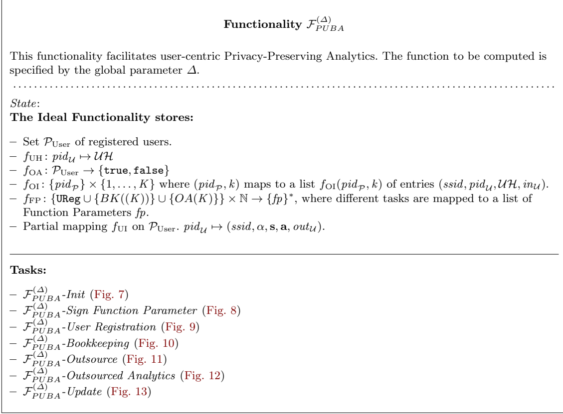
Fig. 6: The basic functionality \mathcal{F}_{PUBA}^{(\Delta)} for user-centric Privacy-Preserving Analytics. The remaining tasks are described in Figs. 7 to 13.
