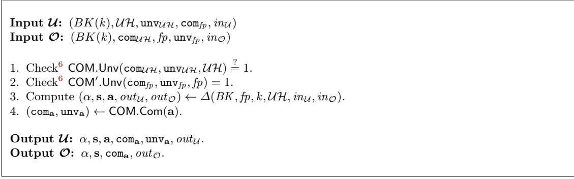
Fig. 16: The subfunctionality-task of \mathcal{F}_{\text{PPA}} for performing direct computations.
