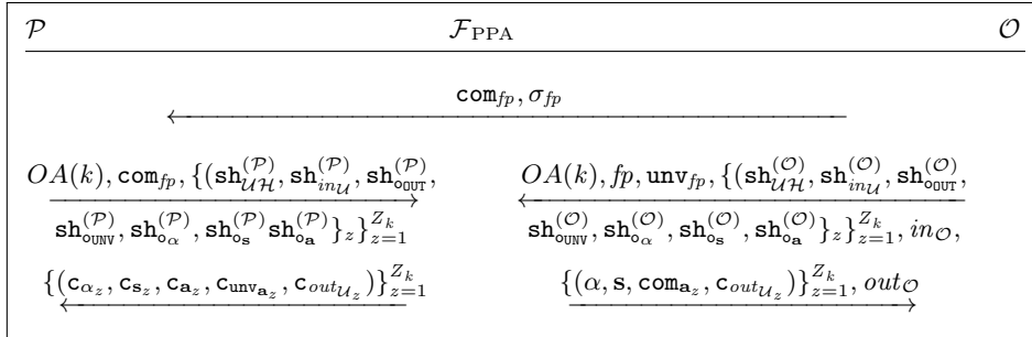
Fig. 35: Message overview for \pi\text{-Outsourced Analytics}^{(k)} .
