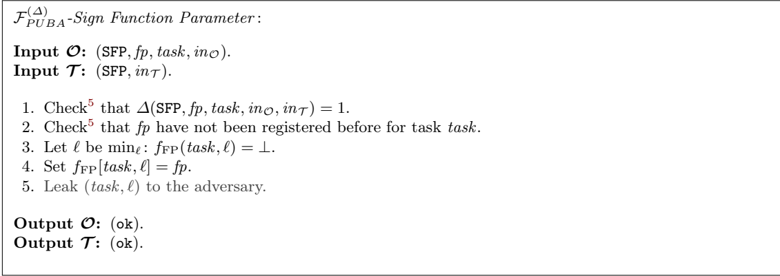
Fig. 8: Task \mathcal{F}_{PUBA}^{(\Delta)}\text{-Sign Function Parameter} for signing Function Parameters.
