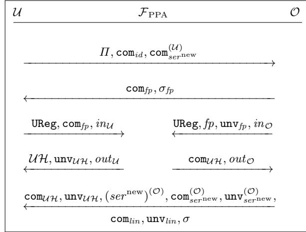
Fig. 25: Message overview for \pi -User Registration.
