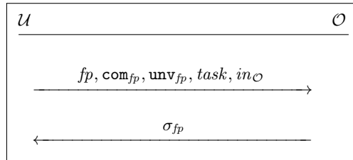
Fig. 23: Message overview for \pi -Sign Function Parameter.
