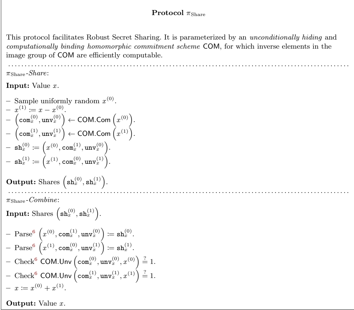
Fig. 18: Protocol for Robust Secret Sharing (RSS).
