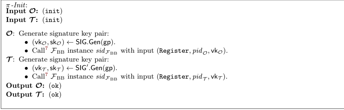
Fig. 21: The protocol \pi -Init for the Init-task (Fig. 7).
