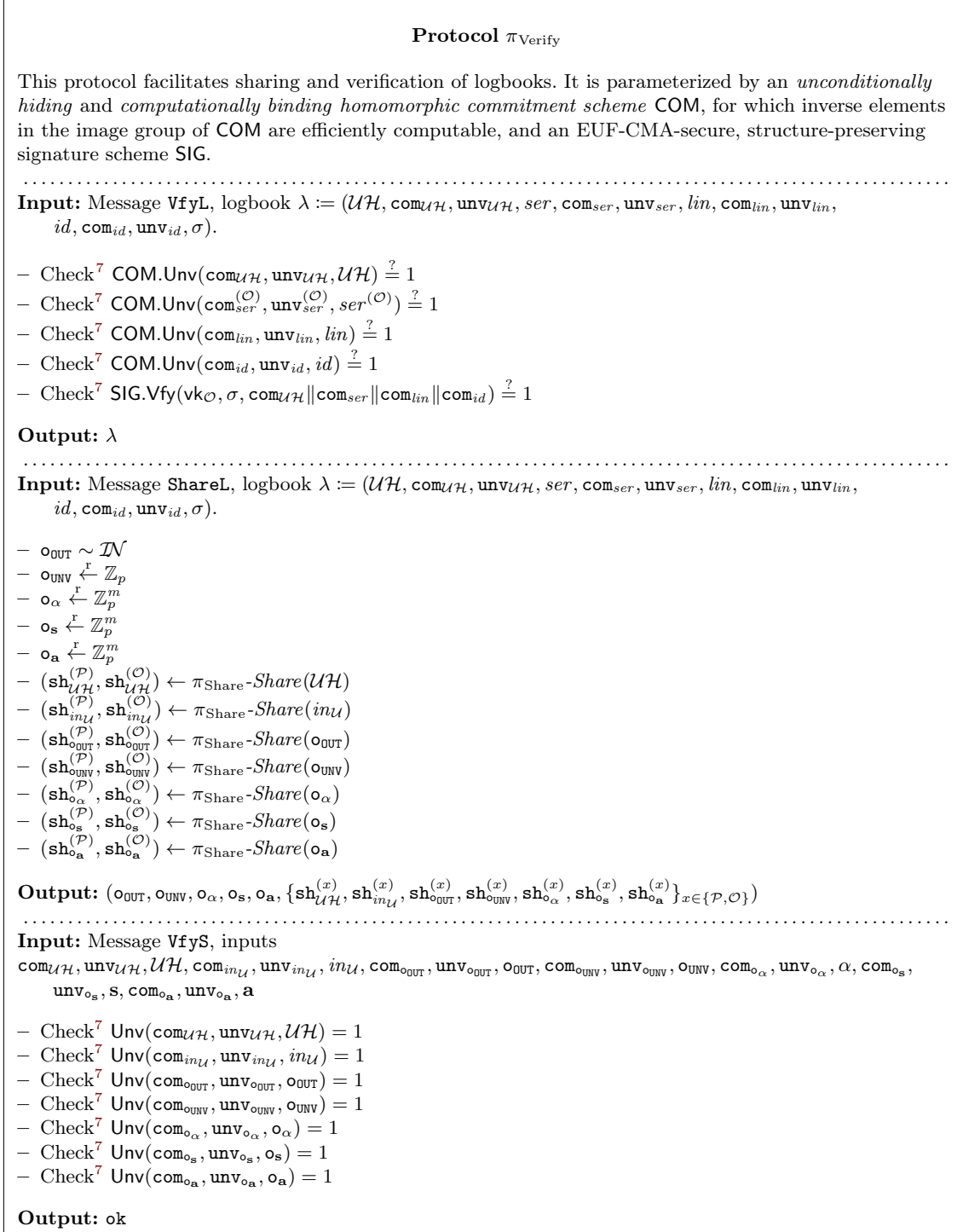
Fig. 19: Protocol for User logbook verification.
