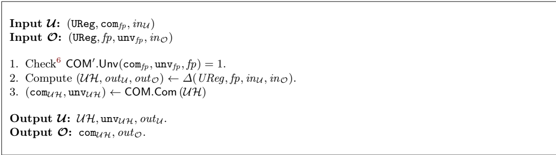
Fig. 15: The subfunctionality-task of \mathcal{F}_{\text{PPA}} for performing user registration.
