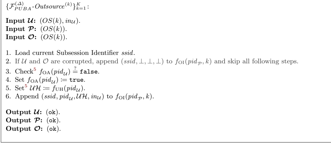
Fig. 11: Task \mathcal{F}_{PUBA}^{(\Delta)}\text{-Outsource}^{(k)} for outsourcing user data required for outsourced computation of the task defined by k \in \{1, \dots, K\} .
