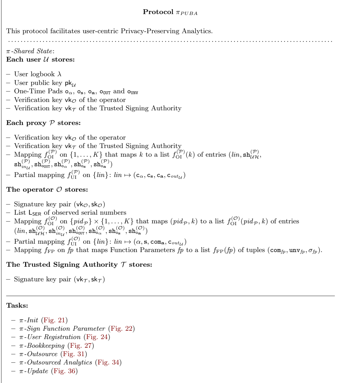
Fig. 20: Shared state of the protocol \pi_{PUBA} .
