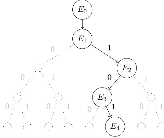
Figure 1: The path followed by the CGL function within the graph \mathcal{G}_2(\overline{\mathbb{F}_{p^2}}) for the bitstring 101.
