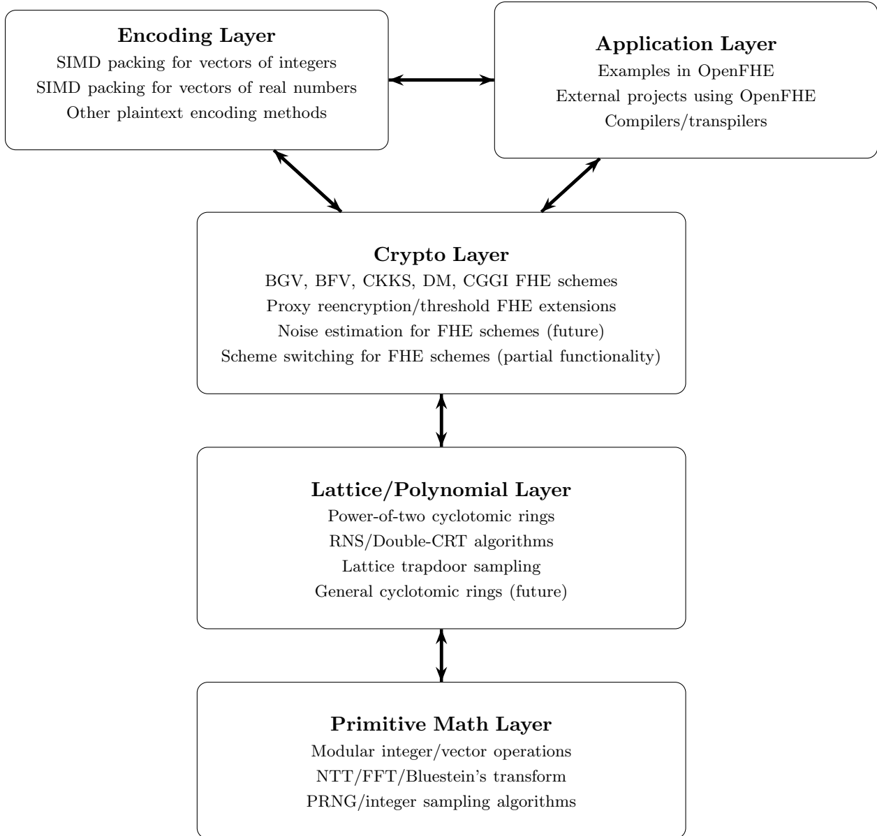
Figure 1: Layers in OpenFHE
