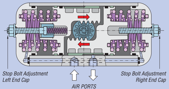
TRAVEL ADJUSTMENTS TOP VIEW
