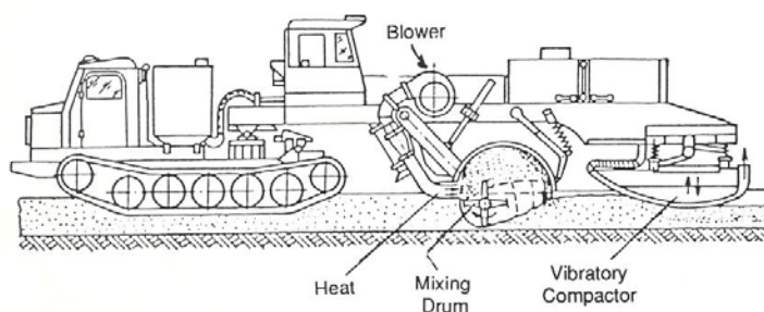
Figure A17. Soviet thermo-vibrating snow compactor (Volkova 1979).
