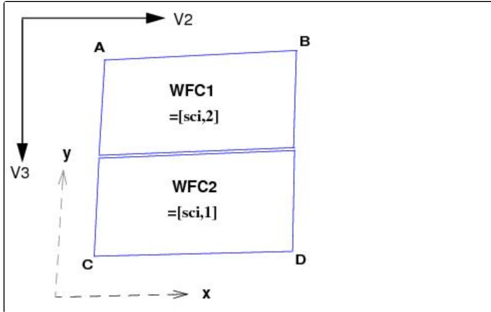
Figure 2.2: WFC apertures Compared with the V2/V3 Reference Frame
