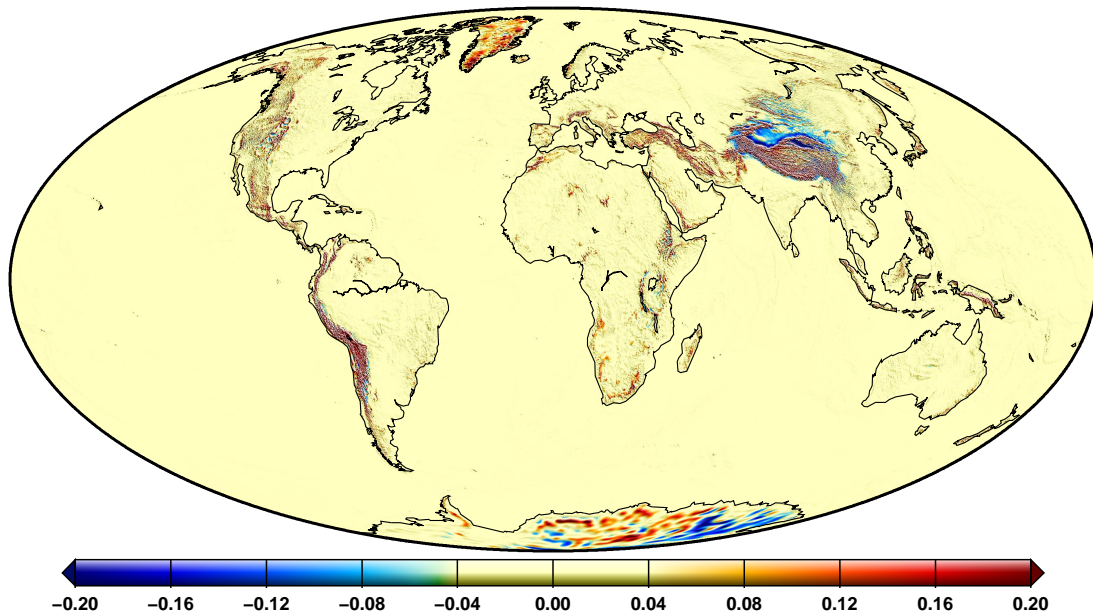
Figure 9: The difference between the pseudo height anomalies on the ellipsoid and the height anomalies on the Earth's surface: (\zeta_{e1} - \zeta) ; wrms = 0.052 m, min = -0.78 m, max = 3.4 m
