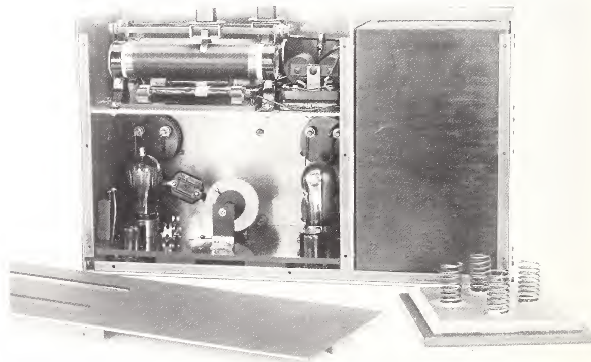
Portable, temperature-controlled, piezo-oscillator, frequency standard designed by Vincent E. Heaton and Walter H. Brattain in 1929. Spring mounting (right) provided vibration isolation to temperature-controlled chamber housing the quartz crystal. Brattain joined Bell Telephone Laboratories in 1929; in 1956 he shared the Nobel Prize in Physics with Shockley and Bardeen for discovery of the transistor effect.
