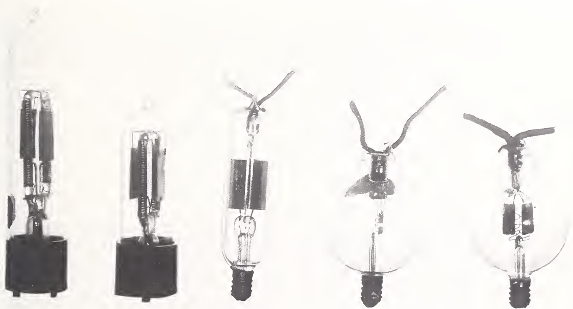
Electron tubes of the de Forest type that were available to the Radio Section during the period of World War I.
