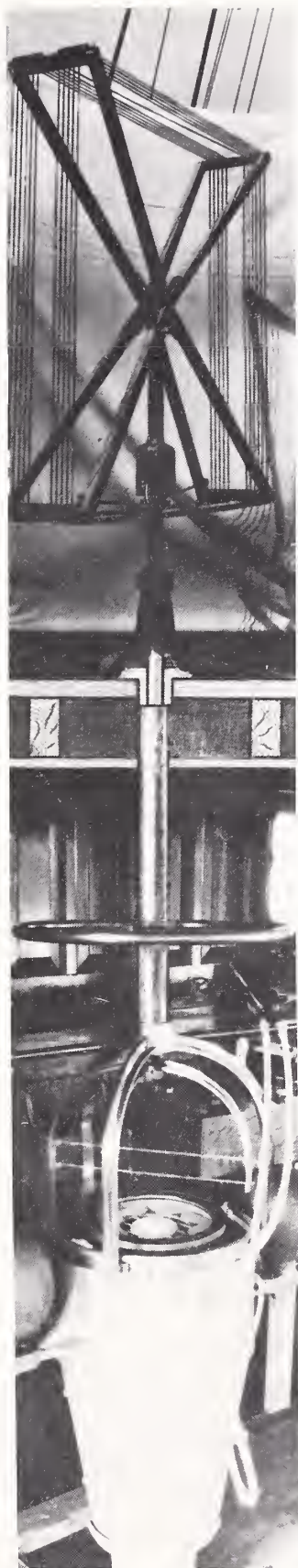
Composite photograph of radio compass installation on board the Bureau of Lighthouses tender Tulip during the summer of 1920. The directional loop antenna was mounted above deck, with rotational control and directional bearing indication and the compass below deck.
