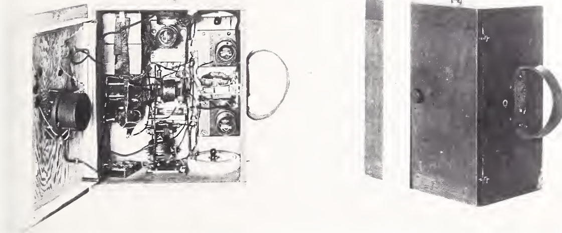
The "Portaphone," a portable radio receiver constructed by the Radio Section in 1921. Included within the wood case (12×12×6 in) was a loop antenna with tuning capacitor, electron-tube detector, two-stage amplifier, and dry batteries. A loudspeaker driver unit fitted with a small "morning glory" horn provided sufficient volume to entertain the passerby with music from local broadcasting stations. A later model completely enclosed a wood horn.
