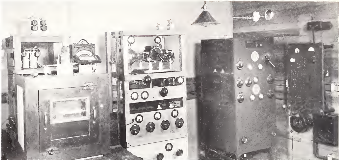
Transmitting equipment of station WWV, College Park, Md. Left front, temperature-controlled cabinet housing 200-kHz control piezo oscillator. Left rear, 150-watt, 5000-kHz transmitter Center, 1-kW 5000-kHz transmitter Right, 1/2-kW multifrequency transmitter Far right, switchboard
