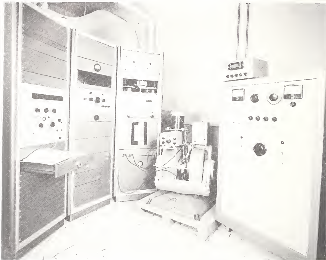
Equipment used in early 1960's for measurement of tensor permeability properties of ferrites at 3100 MHz by the Radio and Microwave Materials Section. The ferrite material was placed in cavity between pole pieces of strong electromagnet (center). Signal generators, detectors, and other electronic equipment are at left. Ferrites have found many uses in RF equipment.
