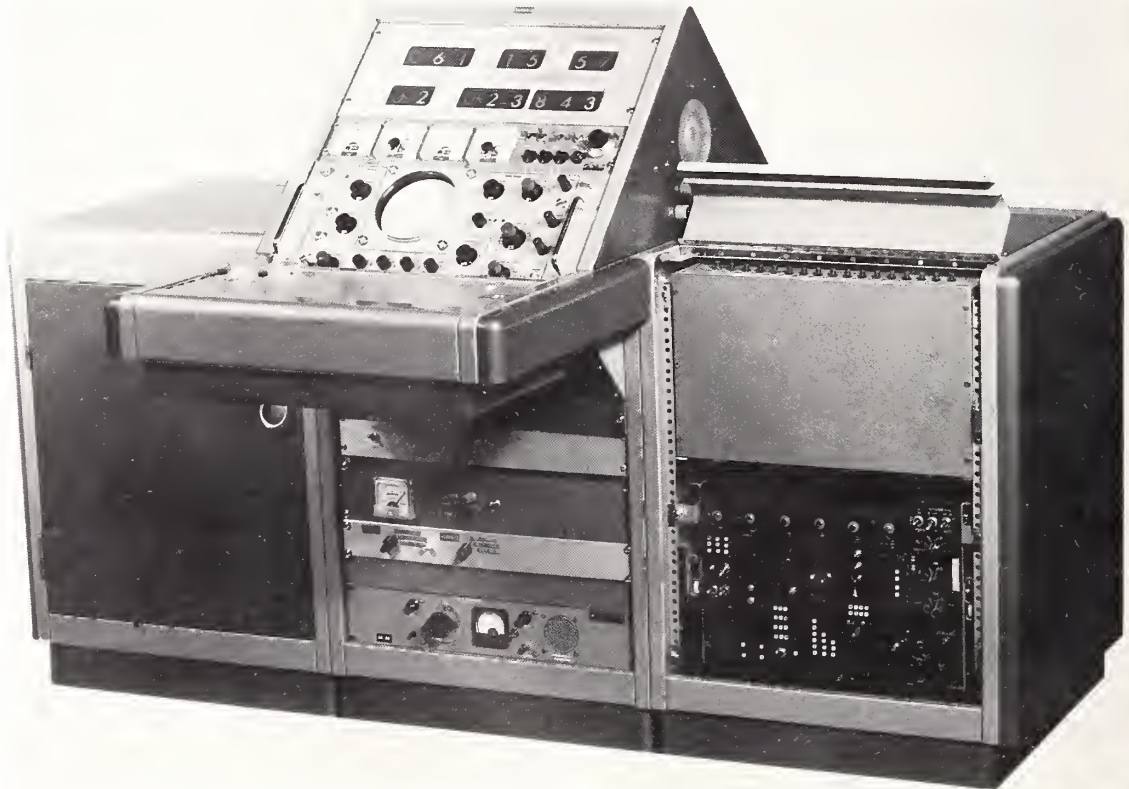
Console of an advanced development model (1961) of the Loran-C clock used to synchronize time (to within 1 microsecond) and frequency at widely separated locations. Receiver equipment in cabinet at right. Electronic circuitry of the Loran-C clock housed in cabinet at left. Above the monitor oscilloscope in center section is the readout that contains a 15-digit visual display covering 1 microsecond to 1000 days.
