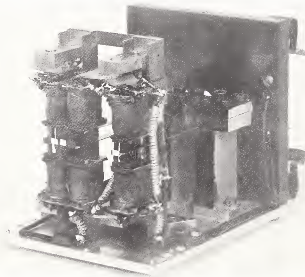
Earliest vibrating-reed-type visual indicator (type A) designed by Dunmore in 1926 for the radio beacon installed at the College Park, Md. Airfield. The two white-tipped ends of permanently magnetized steel reeds can be seen at middle left. Electromagnets from headphone receivers drove the reeds. One reed vibrated at a 60-Hz modulation frequency in response to deviation of plane to one side of course, the other at 85 Hz for opposite side of course. The third reed (right) was used to indicate marker beacons spaced at different distances from airfield. Dunmore brought out a series of reed indicators, each successive stage an improvement in design and performance, and with minor changes in the reed frequencies.
