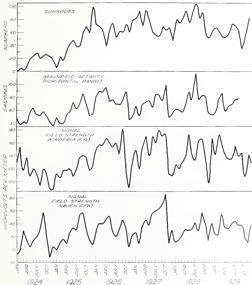
The relation of solar and magnetic activity to long distance radio transmission is indicated by these 1924-1930 observations of Austin and colleagues (of the Laboratory for Special Radio Transmission Research, associated with the Radio Section (see ch. II, pp. 36-37). Monthly averages of signal levels from two low-frequency transmitters (Bordeaux, France, 15.9 kHz; Nauen, Germany, 23.4 kHz) show fairly close correlation with magnetic activity and less correlation with solar activity. Austin stated in a publication that, "The deep drop of both magnetic and signal curves in November (more rarely in December) is especially striking." The effect of early winter North Atlantic transmissions had often been noticed by others.
