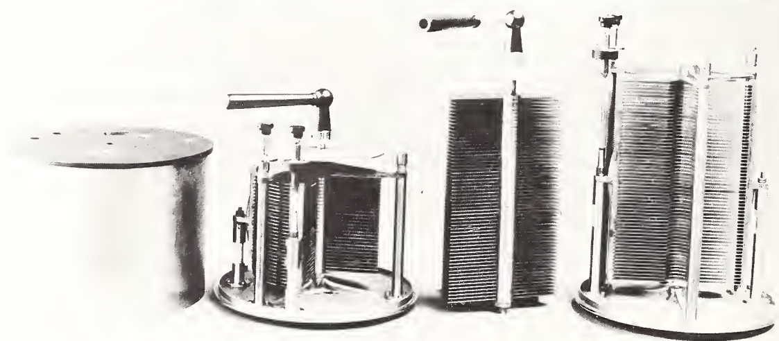
Variable condensers (capacitors) of "Bureau of Standards Type," with quartz insulation, designed in 1915 for laboratory standards. One at left includes the housing. One at right contains 59 fixed and 60 movable plates, with a capacity of 0.007 microfarad.
