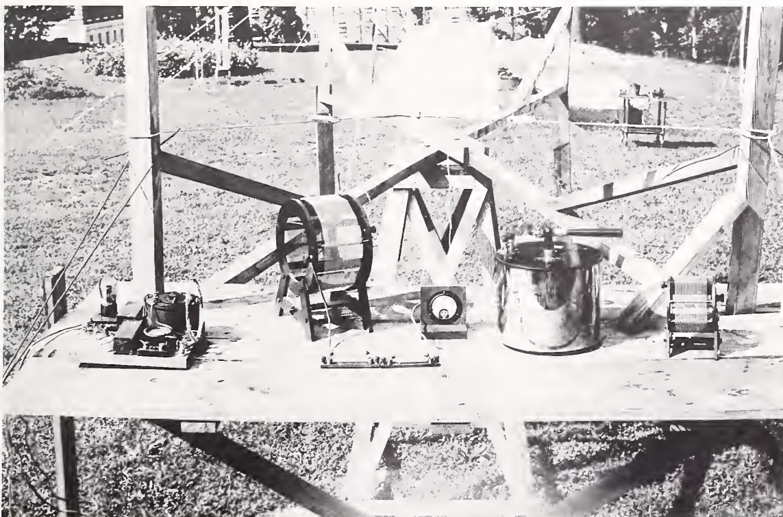
Apparatus, including standard inductor and standard capacitor, used to measure constants of a condenser antenna. Lower plate of antenna is seen beyond measurement equipment. Location is on lawn of Radio Building in the summer of 1920. (East Building at left, recently constructed Industrial Building in far background to the north.)
