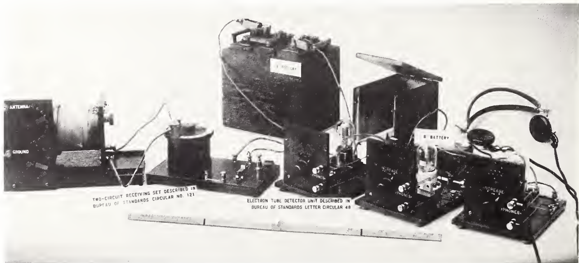
Radio broadcast receiver with two-circuit tuning unit, electron-tube detector, and two-stage amplifier, constructed from directions given in three NBS Circulars published in 1922. Complete with batteries and headphone, this assembly of heavy equipment occupied considerable space, judging by the 2-ft ruler. Today, the equivalent in a transistor radio with enclosed loudspeaker could be held on palm of the hand.
