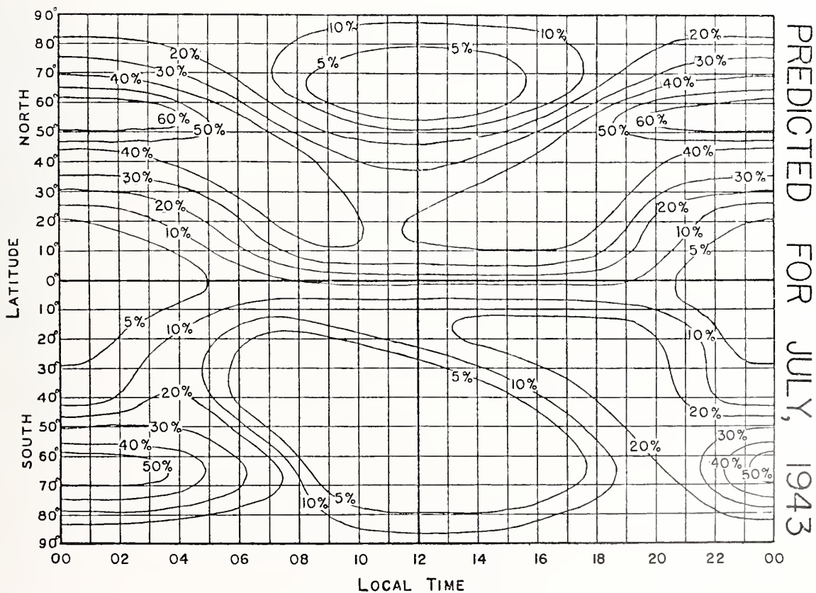
Sporadic-E distribution predicted for July. Numbers on curves are percentage of total time for sporadic-E maximum usable frequency in excess of 15 Mc.
