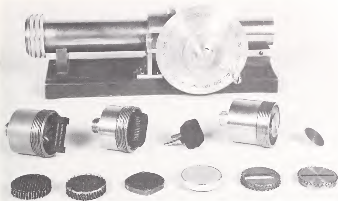
First waveguide below-cutoff or piston-type attenuator designed by Microwave Standards Section and constructed in Bureau shops in 1946. It was used at an intermediate frequency of 20 MHz in the heterodyne method of calibrating attenuators at microwave frequencies. Shown here with experimental components used to determine best operation. In lower row are various types of filters used to suppress unwanted modes of the wave that progressively decays through the piston. In upper row are several means of "launching" the wave and the pickup or receiving coil. This instrument was the progenitor of a lineage of waveguide below-cutoff attenuators that now reach a high state of development at NBS, and is preserved as an historic item.
