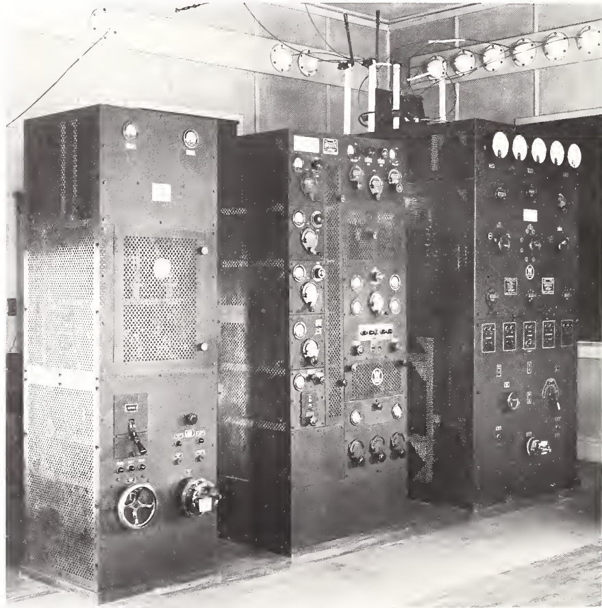
Thirty-kW transmitter of station WWV, Beltsville, Md., 1932-1940.
