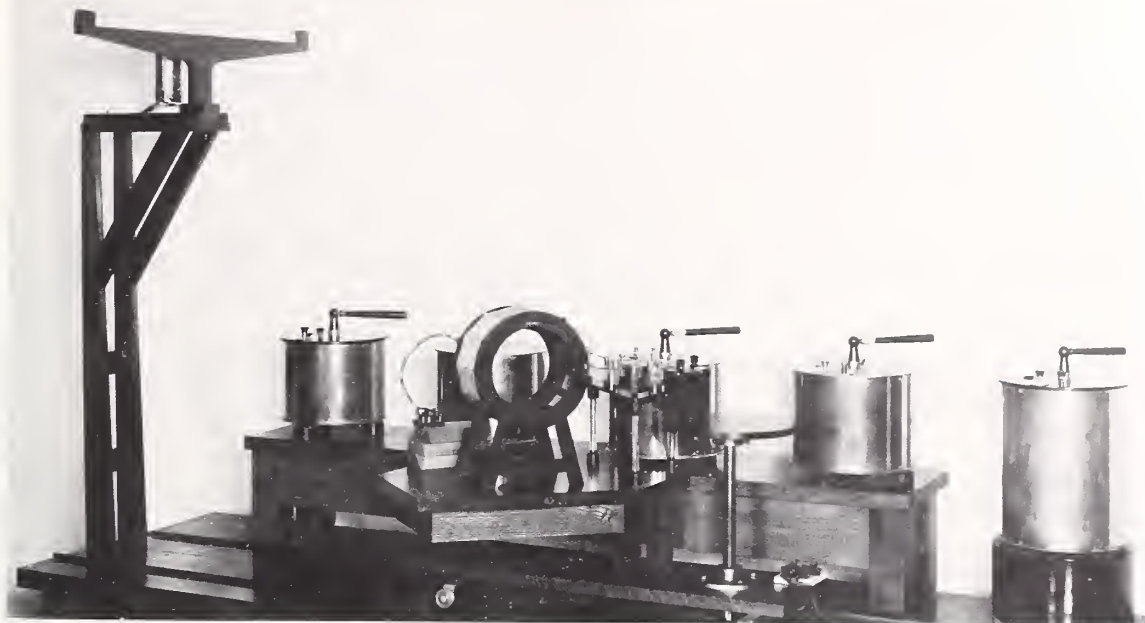
Equipment used for calibration of standard capacitors. The several variable capacitors are of Bureau of Standards design and construction and were very useful for various types of measurements during the early years of the Radio Section.
