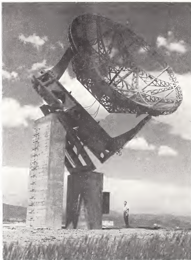
During 1952 the three Würzburg (Giant) antennas were moved from Sterling, Va., to Colorado and installed on Gunbarrel Hill, northeast of Boulder. They served for many years as "collectors" for the study of solar radio noise. Such an antenna is geared to track the Sun in its daily path across the sky.
