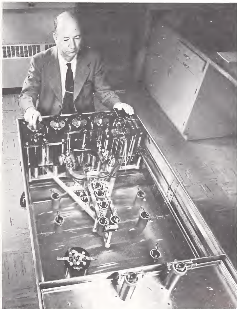
Photograph (1958) of Frank Weaver, head of Low Frequency Unit, Electronic Calibration Center, operating precision bridge used to calibrate standard resistors with uncertainty of less than one part per million. The bridge was a development in 1918 by Dr. Frank Wenner of the Electricity Division, and a small number have been manufactured through the years. Originally called the NBS Precision Bridge, it became better known as the Wenner Bridge. All parts of bridge, except control knobs, are submerged in oil at constant temperature of 25 °C.
