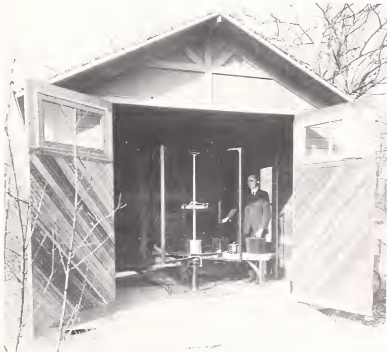
Direction finder at Kensington, Md. field station in 1919, being operated by L. E. Whittemore. A cooperative program (engaged in by L. E. Voorhees) with the Navy revealed large errors in directional bearings caused by the ionosphere. The received signals were from transmissions of long wavelengths (e.g., 13,600 meters, or 22 kHz).
