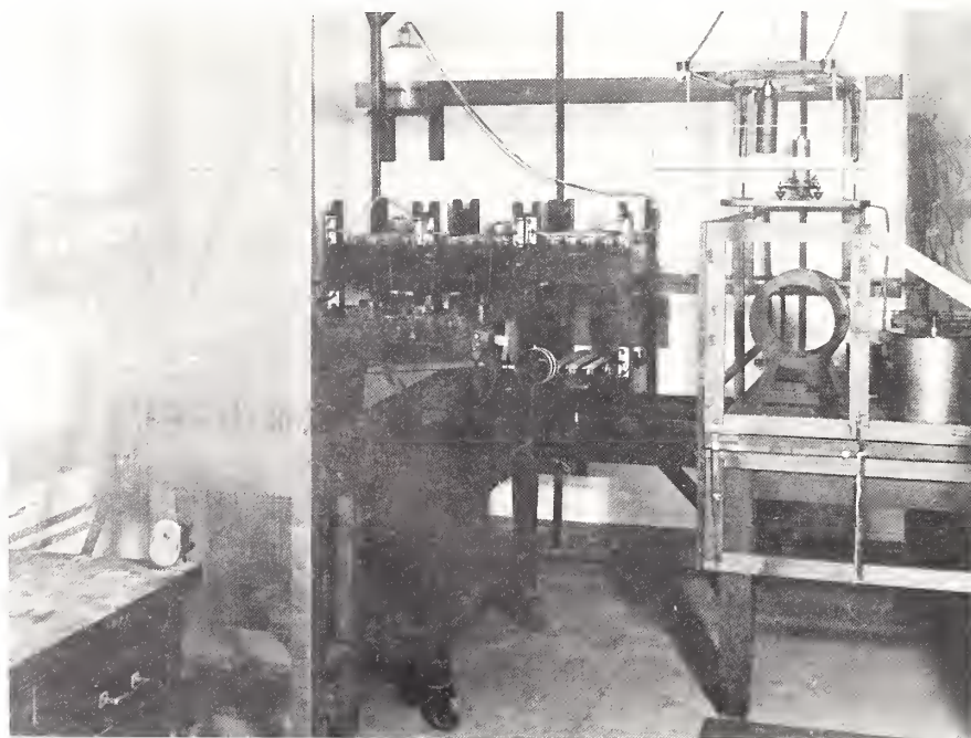
Apparatus used in 1921 to measure the phase difference (or power factor) and dielectric constant of insulating materials from 7.5 to 3000 kHz. Measurements were performed in a shielded room of window screening. Dellinger was the principal investigator on the project for several years.
