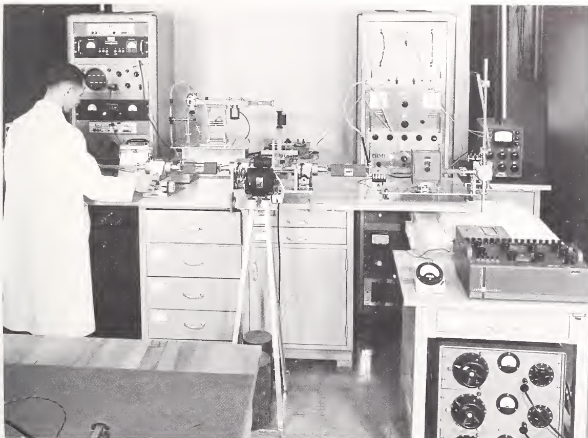
Microwave radiometer in X-band (8.2-10.4 GHz) developed by 1962 to measure the noise temperature of gas-discharge noise sources for use as interlaboratory standards.
