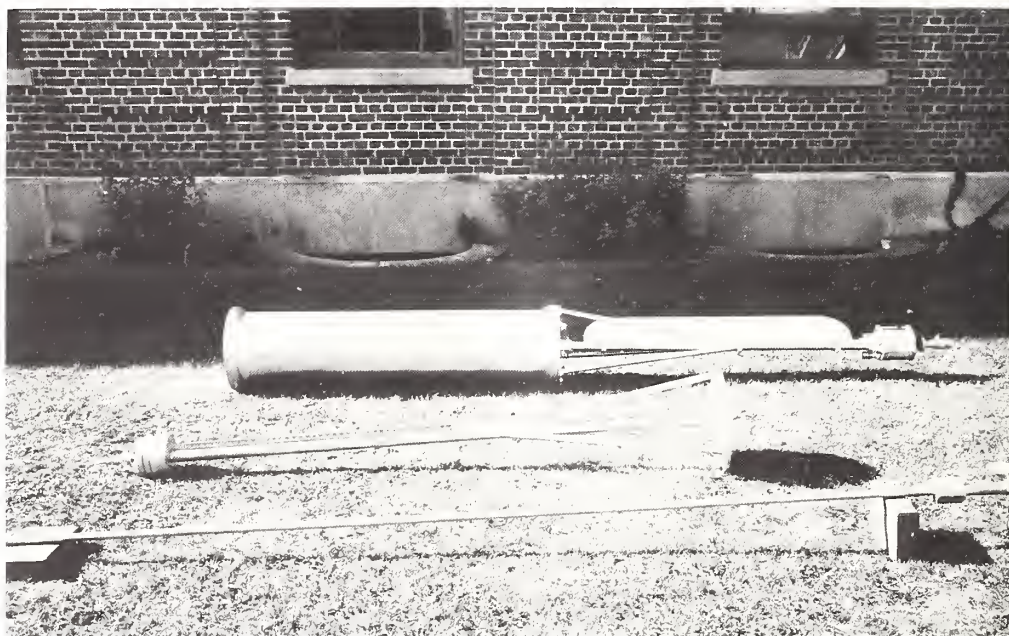
Buoy-type automatic weather station developed for the Navy, shown here disassembled in three sections for transportation. Copied in principle after "Grasshopper," this remote weather station was the first of a series of the buoy-type developed by NBS for the Navy since World War II. Observation of wind speed and direction was an added feature. Today, these stations operate for many months at a time without servicing.
