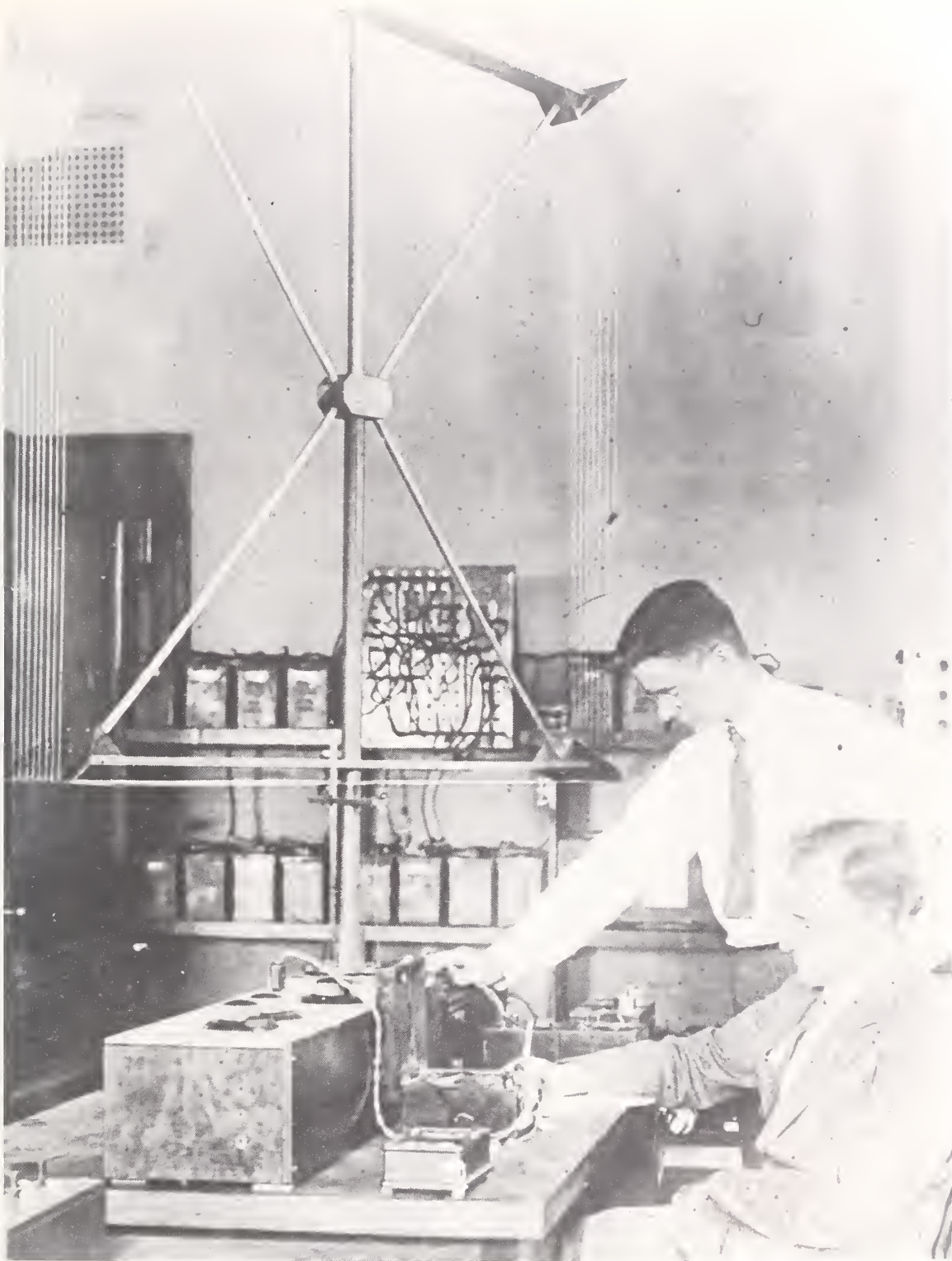
Dellinger (seated) and Taintor Parkinson measure the field strength of a distant high-power radio station with early-type equipment. Use of a loop antenna was considered "standard" procedure for making such measurements. Photo taken September 4, 1925. A year later the Radio Section developed its first field-intensity (strength) meter (see ch. V, p. 111).
