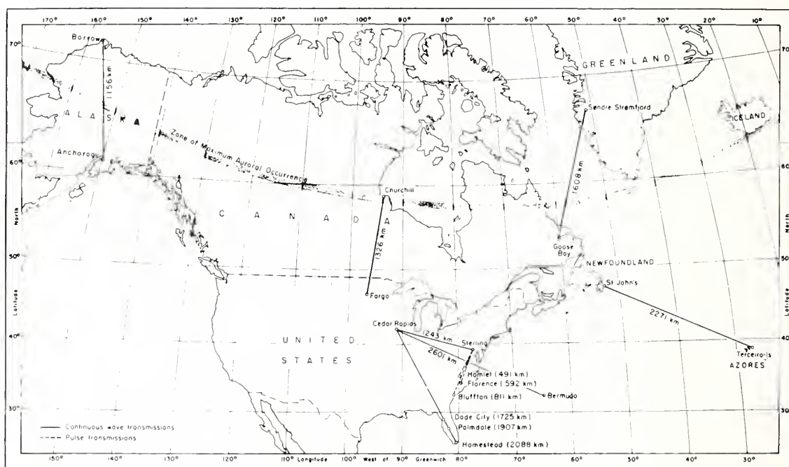
Experimental paths used by NBS in the study of radio transmission by ionospheric forward scatter. Two paths crossed the zone of maximum auroral occurrence, another path (Fargo to Churchill) terminated at the zone. These two paths were used in special studies of ionospheric forward scatter at high latitudes. Signals were observed for the first time on January 23, 1951, at Sterling, Va., over a 1243-km path from Cedar Rapids, Iowa.
