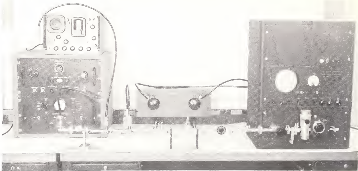
Measurement of X-band attenuator in 1946, using a heterodyne system operating at 20-MHz intermediate frequency. A carbon resistor coaxial-type attenuator covering a range of 40 dB was used as the standard attenuator. Microwave power came from the klystron oscillators.
