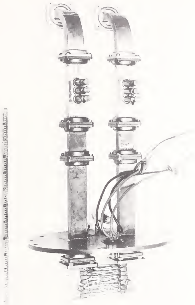
Waveguide section of the first of a series of microwave microcalorimeters (Joule twin type) developed by NBS, this one by Macpherson and Kerns, beginning in 1948. Earliest model used polyiron as the absorbing load at about 1 milliwatt of RF power; replaced in later models with a bolometer unit. A dummy load served as the temperature reference for the multi-junction thermopile (lowest portion of photograph). Tuning stubs (upper portion) provided impedance matching of X-band assembly at 9315 MHz. Entire unit was temperature controlled in a 45-gallon oil bath.
