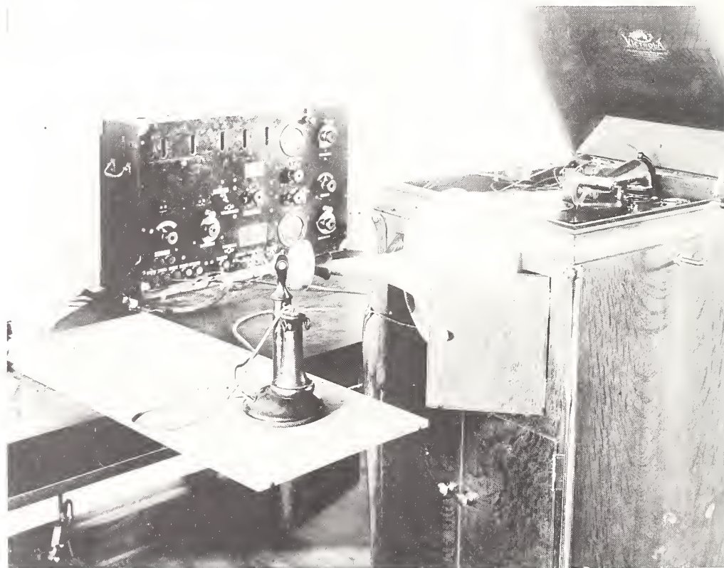
During the spring of 1920 the Radio Section broadcasted music over station WWV in advance of the scheduled commercial broadcasts later in the year. A Victrola phonograph was the source of music, with pickup by a "microphone" using a telephone transmitter fitted with a "morning glory" horn. U.S. Army Signal Corps radio equipment served as the transmitter.
