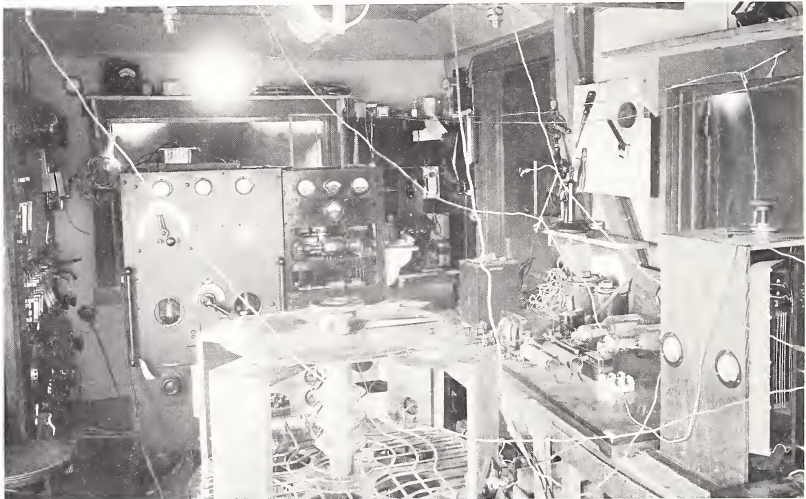
Experimental transmitting equipment at base of radio beacon tower, College Park, Md. Goniometer (mutual inductor in antenna feed to control direction of transmitted signals) in foreground. Another type of goniometer at right.
