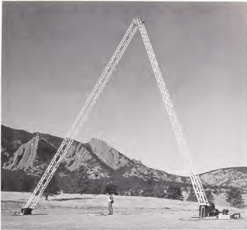
Model antenna range located on Green Mountain Mesa at base of the Flatirons, Boulder. The inverted V-frame of improved design replaced the one brought from the flatlands of Sterling, Va. Being measured for antenna patterns, as shown in this photo of 1962, is a model of the National Science Foundation's Antarctic research ship USNS Eltanin fitted with several types of model antennas, located on ground plane in front of observer.
