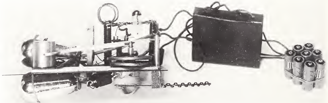
Earliest form of the radio meteorograph (later called radiosonde) developed by the Radio Section in 1935. An aneroid barometer indicated air pressure (hence altitude); the rotation of a spiralled bimetallic strip indicated temperature; each movement modulated the transmitter oscillator. Observation of humidity was to come later.
