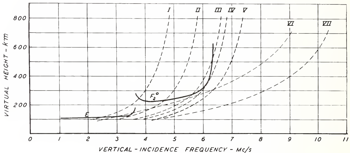
Earliest published (July 1937) transmission curves by NBS for determination of frequency for selected distances of transmission (assuming flat Earth and flat ionosphere). In a generalized form, this whole procedure by Newbern Smith shows the various relationships. The solid curve is a typical normal-incidence observation of virtual height vs. frequency, showing the E and F_2 layers of the ionosphere. The dotted curves depict conditions of transmission for various frequencies and several distances. For example, curve IV depicts maximum possible frequency for a given distance. Adoption of this method became valuable for predicting median values of maximum usable frequency for propagation over any path at any time of day for several months ahead, and provided for world charts during World War II for predictions.
