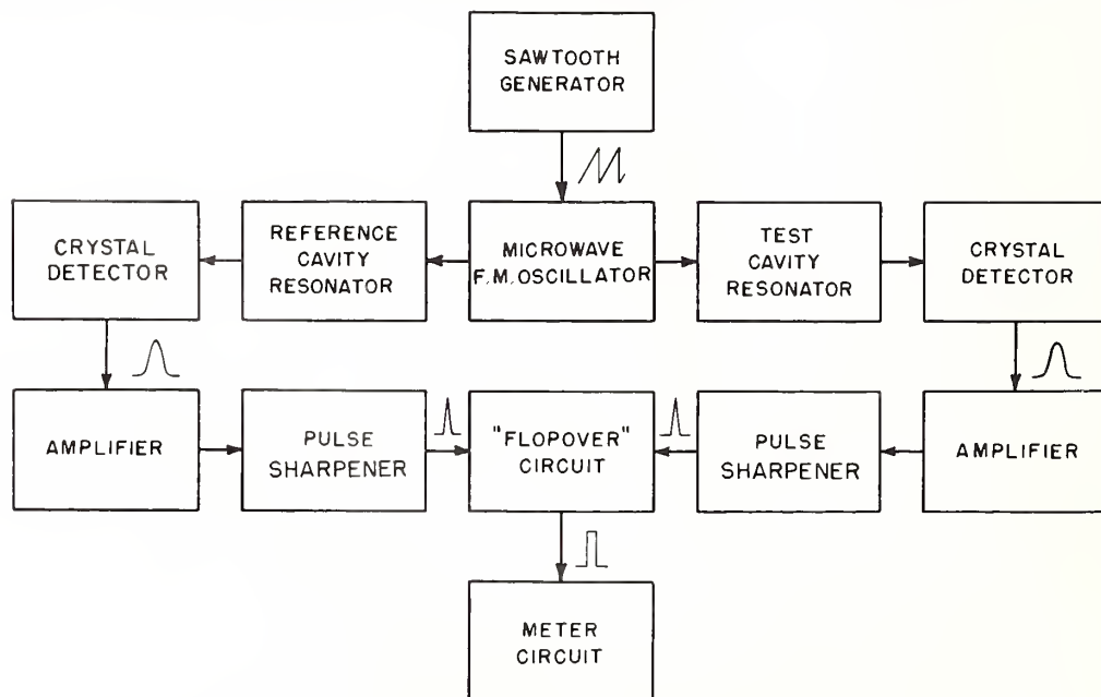
Early form of the recording microwave refractometer developed by George Birnbaum of the Microwave Standards Section during latter 1940's. Initiated by a defense project, this instrument became useful for dielectric studies and particularly for continuous measurement of refractive index of the atmosphere for propagation studies.
