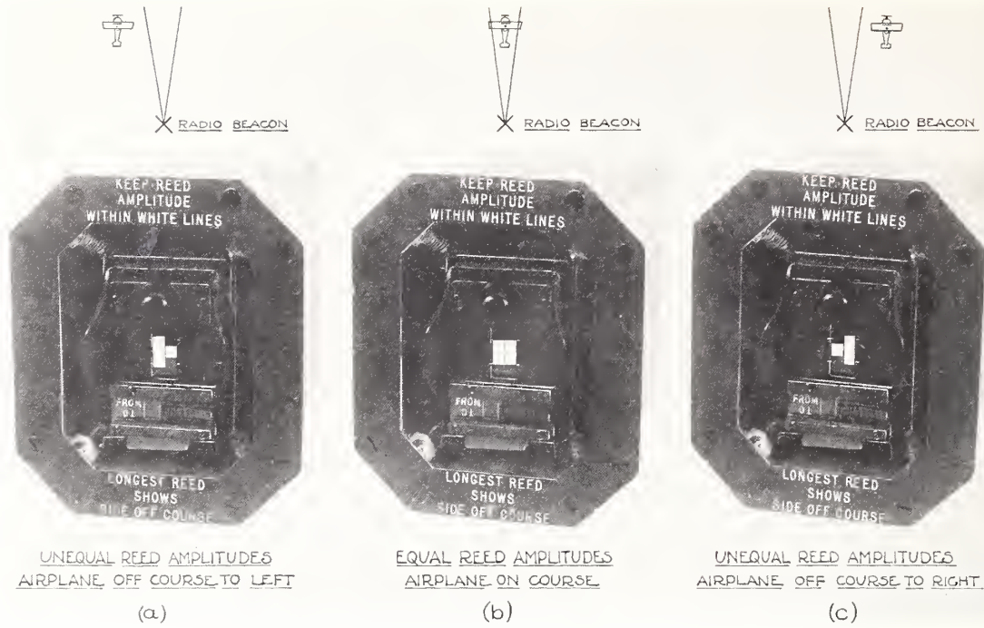
Much improved design of vibrating-reed course indicator—showing the three conditions of travel along beacon course.
