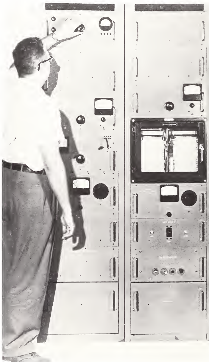
Robert T. Disney at controls of the NBS Model ARN-2 Atmospheric Radio Noise Recorder. This equipment covers a frequency range of 15 kHz to 20 MHz, operating on eight fixed-frequency channels. A number of these recorders were manufactured on contract for use in the IGY noise measurement program of 1957-1958 that was supervised by NBS personnel.
