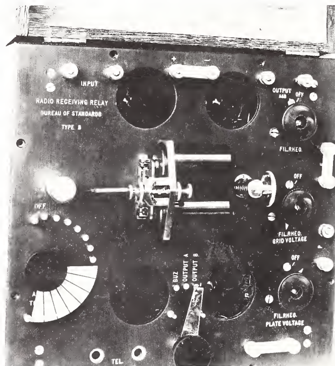
Remote control by a radio signal was achieved in 1922 by Dunmore with his design of this "radio receiving relay." One model was energized by batteries, another operated from 60-Hz alternating current—a new achievement. Remote control by radio signals became a common mode of operation in later years—eventually to distances of interplanetary space.
