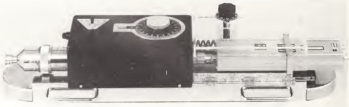
One of the more recent progenies of the lineage of waveguide below-cutoff attenuators developed at NBS. Many refinements are featured in this model, including the added 30-dB amplifier unit (right). The precision attenuator operates at 30 MHz over a range of 60 dB. Position of the receiving coil by a motor-driven precision-screw movement is observed with a revolution counter and dial readout.
