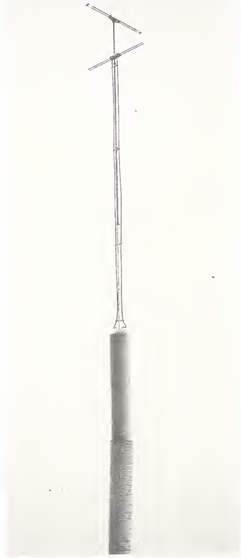
As a component of the Navy's Project CXJX of simulating a false fleet of ships was this buoy-supported jammer of radio signals. The turnstile antenna gave an omnidirectional pattern to the radiated signals. Small boats could be used to launch these jammers along an enemy shoreline in preparation for an amphibious landing. A water-soluble plug allowed the device to sink after several hours of operation.
