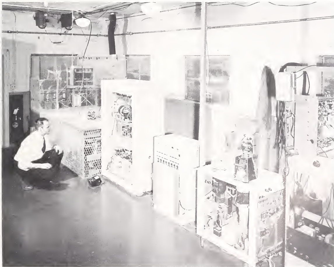
Beginning in 1956, this "one-of-a-kind" ionosonde with a sweep-frequency range of 50 kHz to 2 MHz was used for a number of years for studying the ionosphere at low frequencies. Located at the Sunset field station northwest of Boulder, RF power was radiated efficiently by a very long antenna stretched across Four-mile Canyon and anchored at each end to a mountain top. William S. Hough is shown ready to push a button that started the cycle of operation.
