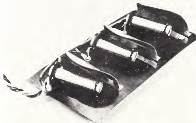
Glass tube (upper component) encloses electrolyte used as a resistance thermometer. On opposite side of panel a group of electric hygrometers in three sensing ranges indicated a wide range of relative humidity.
