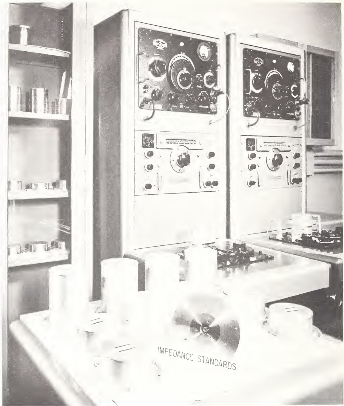
This photograph of 1958 shows 2 of 18 consoles that were being developed in an ambitious project in the Electronic Calibration Center for the calibration of impedance bridges in the frequency range of 30 kHz to 300 MHz. In foreground is assortment of impedance standards of resistance, inductance, and capacitance, shielded in "top hat" enclosures. A specially designed connector made contact with the standard bridge. Passage of time and experience led to a simpler method of calibrating bridges.
