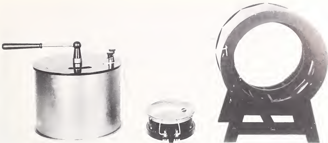
Very early wavemeter developed by Radio Section. This photograph was published in NBS Circular 74, "Radio Instruments and Measurements" (issued March 23, 1918), with the title "Standard wave meter circuit." Wavelengths over the range of 100 to 13,000 meters were calculated from low frequency calibrations of several capacitors and inductors, taking into account the high frequency effects of leads, distributed capacity of inductors, and losses in capacitors. Resonance was indicated by current flow in loosely-coupled, single-turn loop and thermal ammeter.
