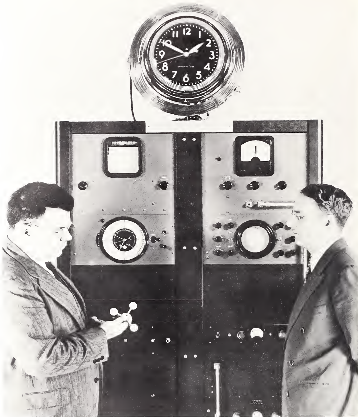
Dr. Harold Lyons (right), inventor of the ammonia absorption cell atomic clock, observes, while Dr. Edward U. Condon, director of NBS, examines model of ammonia molecule. Frequency control, and thus time-rate control of clock, came from the inversion or absorption frequency of ammonia at 23,870.1 MHz.
