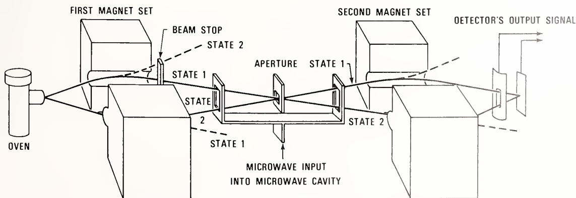
SCHEMATIC ILLUSTRATION OF MAJOR COMPONENTS AND BEAM PATHS OF NBS-5
