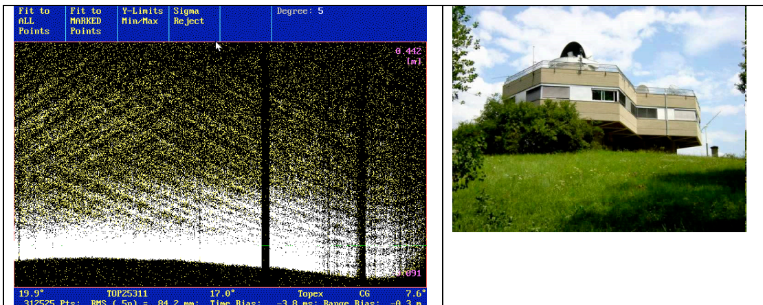
Figure 1 2 KHz returns from Graz Station with a 35 ps pulse width on the TOPEX Satellite (provided by Georg Kirchner)
