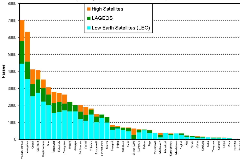
Figure 5 Tracking record in pass numbers for each station during 1998 (ILRS web)
