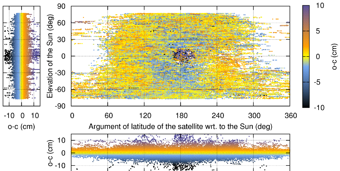
Figure 3: SLR residuals vs. Microwave-based orbits, as a function of Sun projection in orbit plane ( u ) and Sun angle with orbit plane ( \beta ). \beta < 14 and u = [170, 190] corresponds to eclipse. The lack of data in the regions u \sim 0 and u \sim 360 indicates no daylight tracking. The plot is based on the residuals of the SLR observations from the GPS satellites over the time frame of 1995 to 2008 using the ESOC reprocessed orbits.
