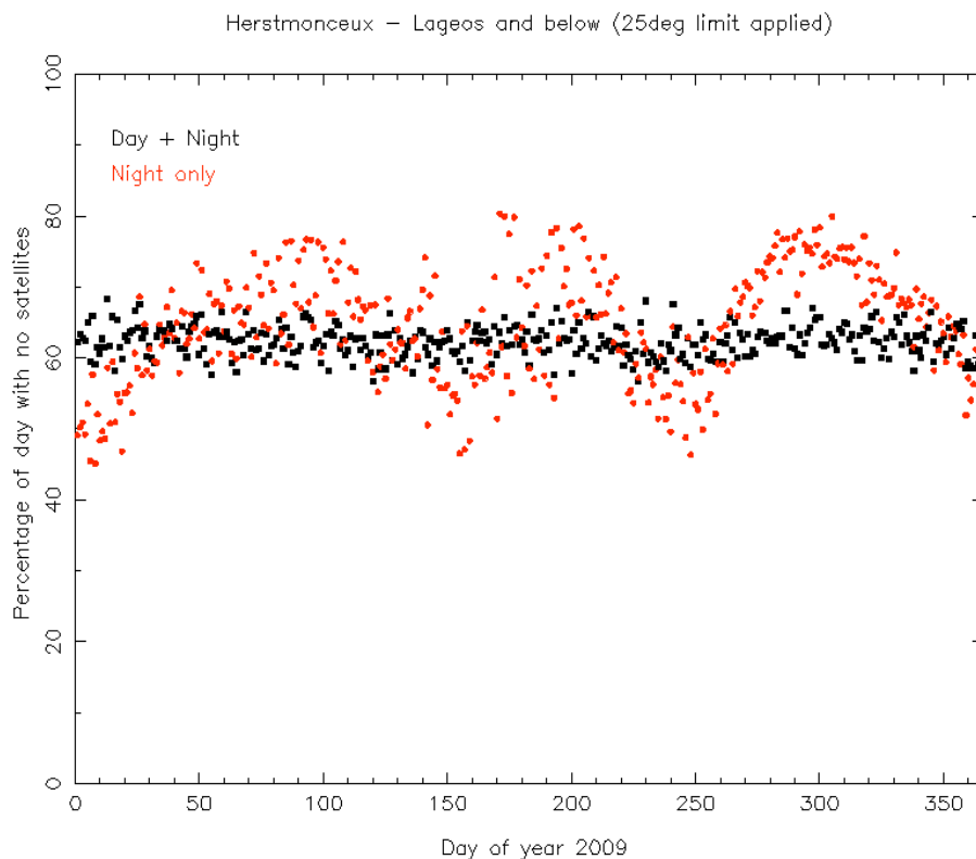
Figure 3 (a) Percentage of time per day when no LEO->LAGEOS satellites are available
