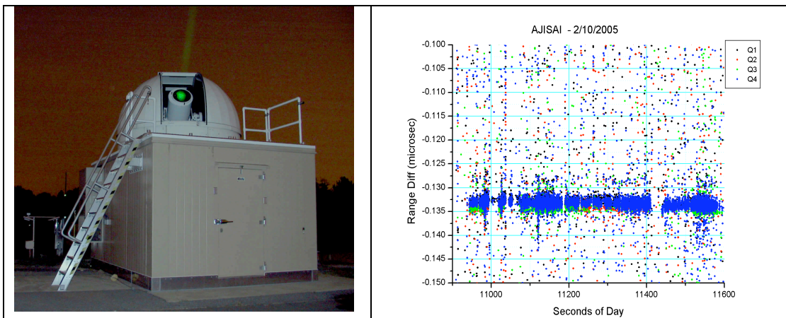
Figure 2 2 KHz returns from the NGSLR Station with a 300 ps pulse width on the Ajisai Satellite (provided by Jan McGarry).
