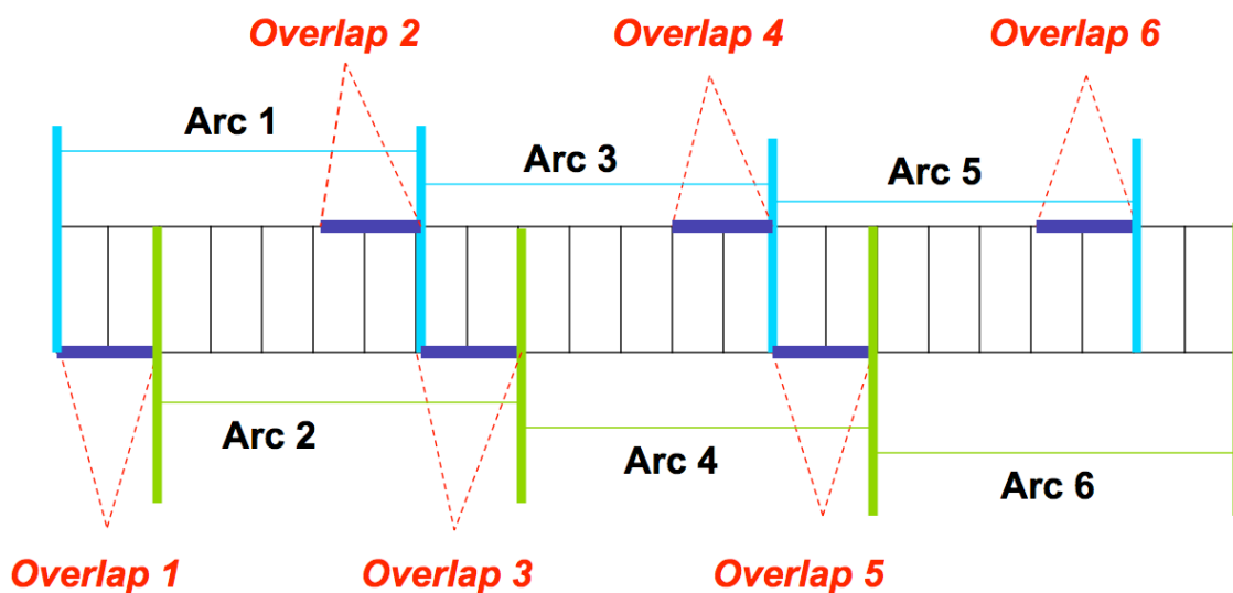
Figure 1. Definition of the adopted 7-day arcs, with a sliding 2-day offset.
