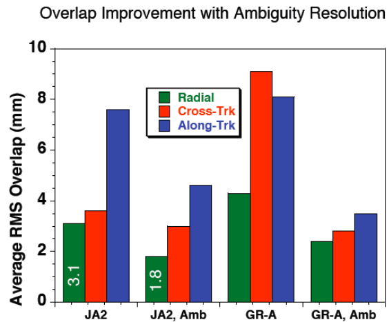
Figure 2. Orbit overlap RMS for Jason-2, based on improved ambiguity resolution [Bertiger et al., 2009].
