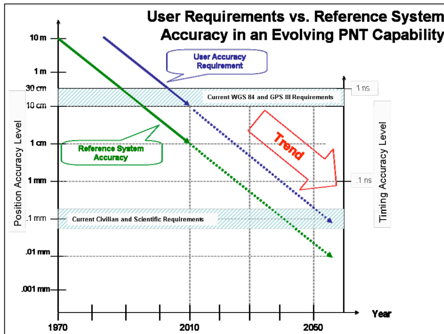
Figure 5. The figure illustrates the evolution of user accuracy requirements versus positioning system accuracy capability using an extrapolation of the historical trends of the past four decades.
