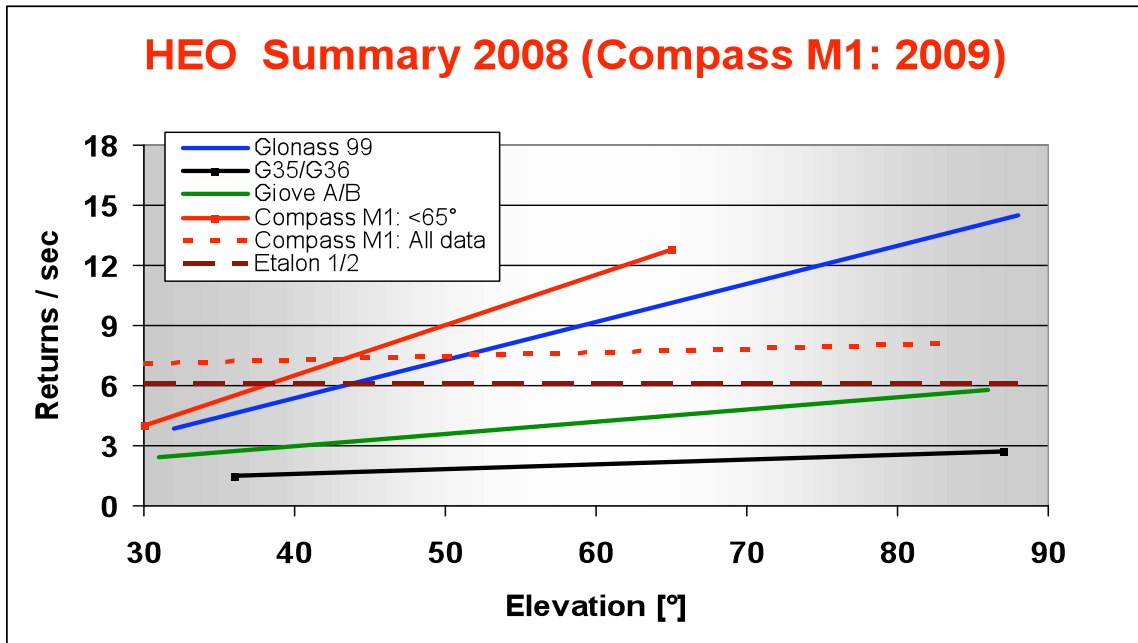
Figure 4. GNSS return signal test at Graz station (provided by Georg Kirchner)
