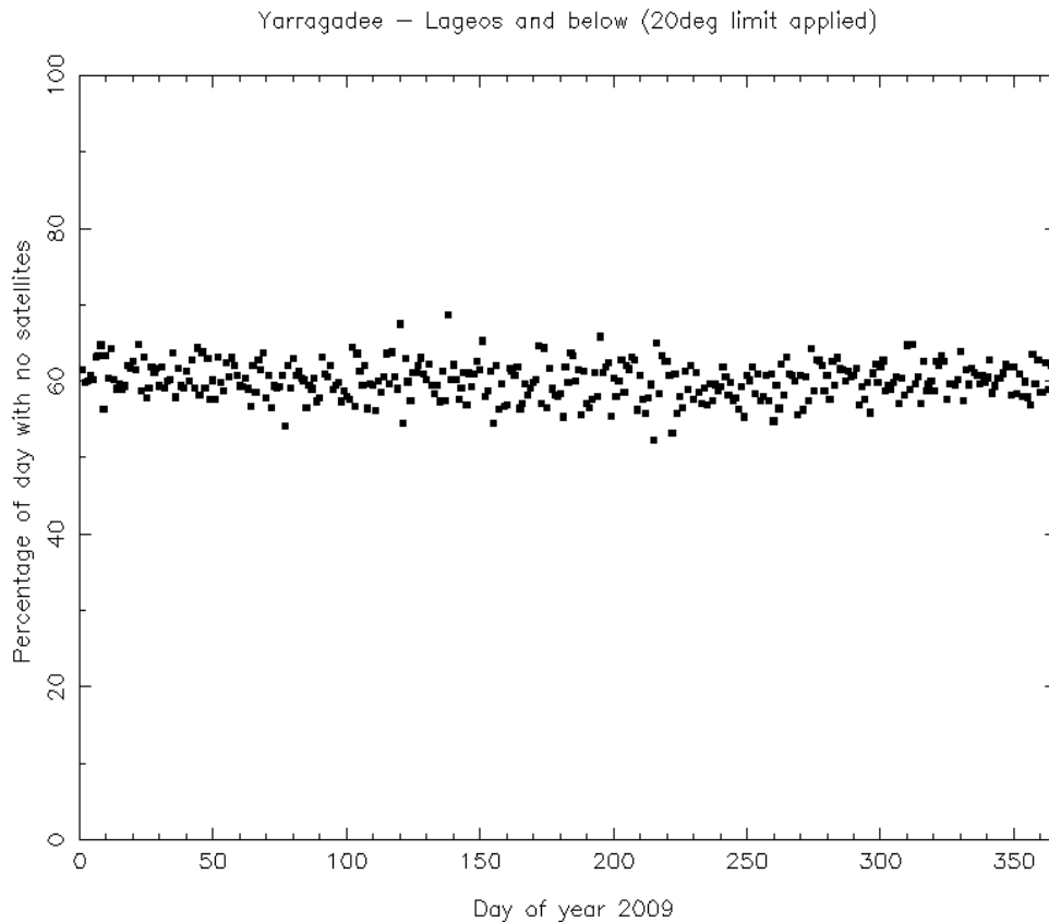
Figure 3 (b) Percentage of time per day when no LEO-> LAGEOS satellites are available.
