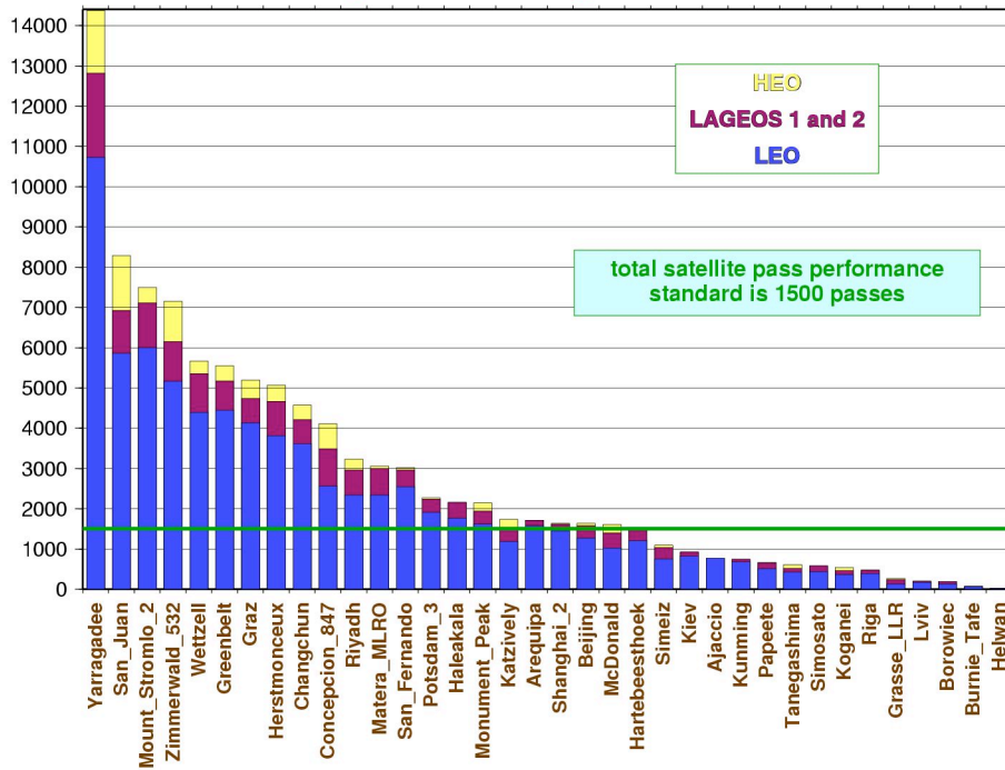
Figure 4 Tracking record in pass numbers for each station during the past year. (ILRS web)
