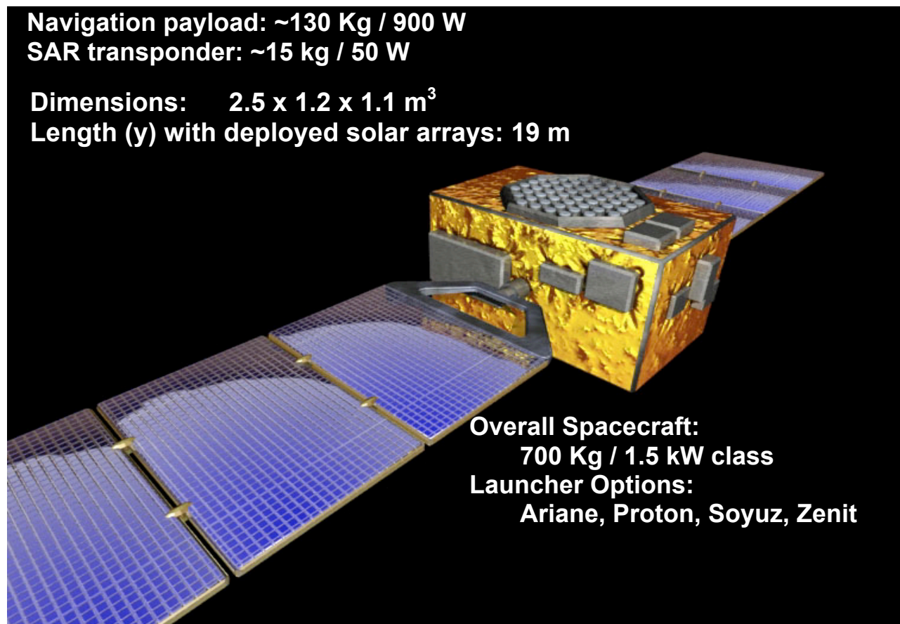
Figure 2: Artist Impression of a Galileo Satellite
