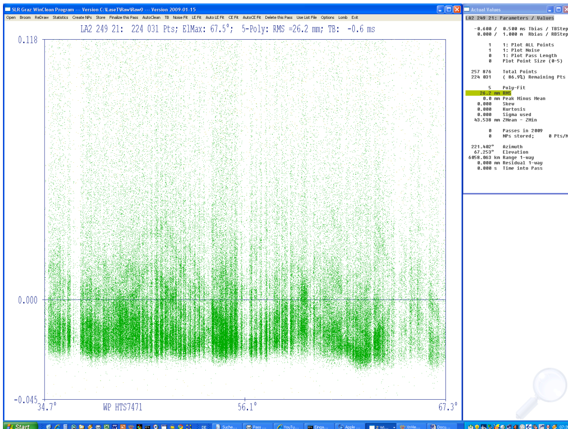
Figure 1b 2 KHz returns from Graz Station with a 35 ps pulse width on the Lageos 2 Satellite (provided by Georg Kirchner)
