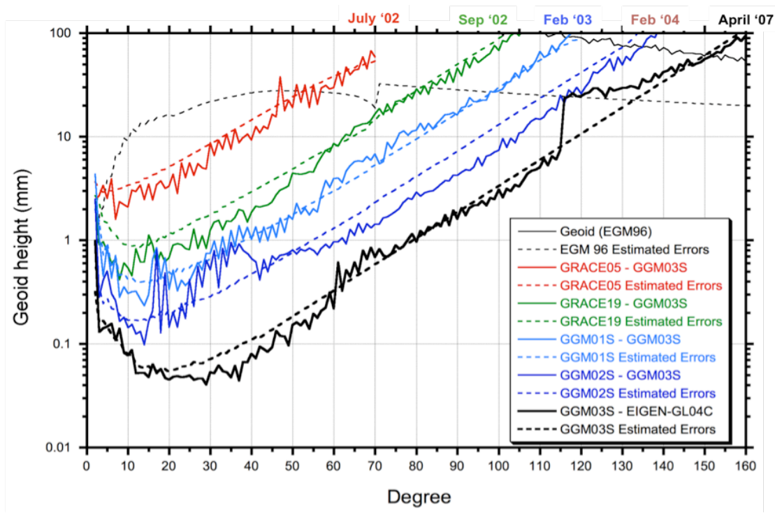
Figure 1. Geoid height error spectrum for GRACE-derived gravitational field models.
