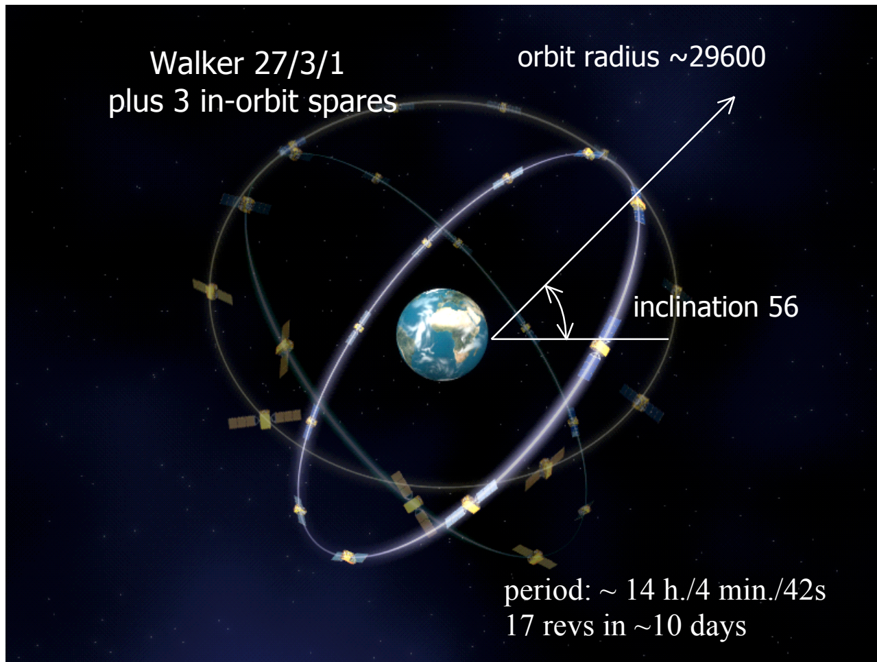
Figure 1: Artist Impression of the Galileo Orbit Constellation
