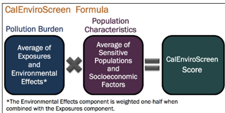
Figure 8-2: CalEnviroScreen Formula
