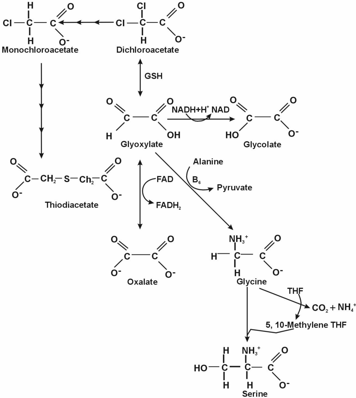
Figure 3-1. Metabolism of DCA
