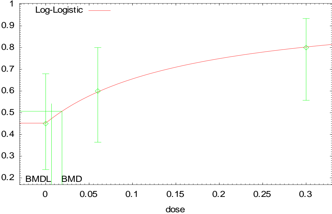
Log-Logistic Model with 0.95 Confidence Level
