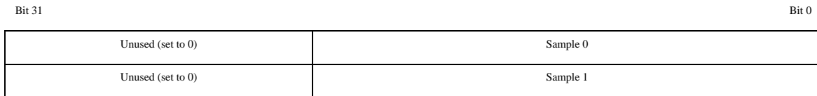
Figure 8: Real 20 bits/sample data-word format
