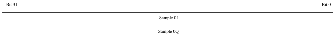
Figure 15: Complex 32 bits/sample-component data-word format
