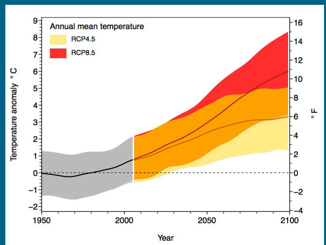
Caption: Projected annual temperature simulations for both high emissions scenario (RCP 8.5) and lower emissions scenario (RCP 4.5) for the Northwest United States to the year 2100. (Figure source: David E. Rupp; data source: Rupp et al. 2016, adapted.)
