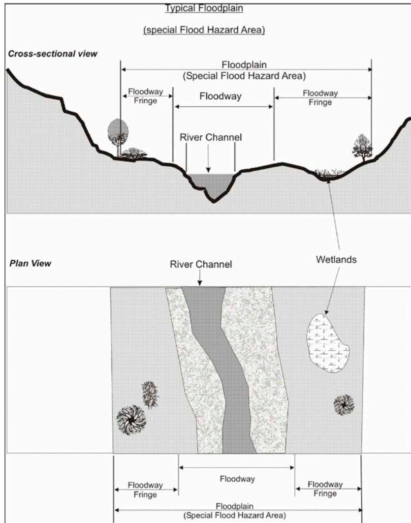
FIGURE 14: FLOODWAY SCHEMATIC
