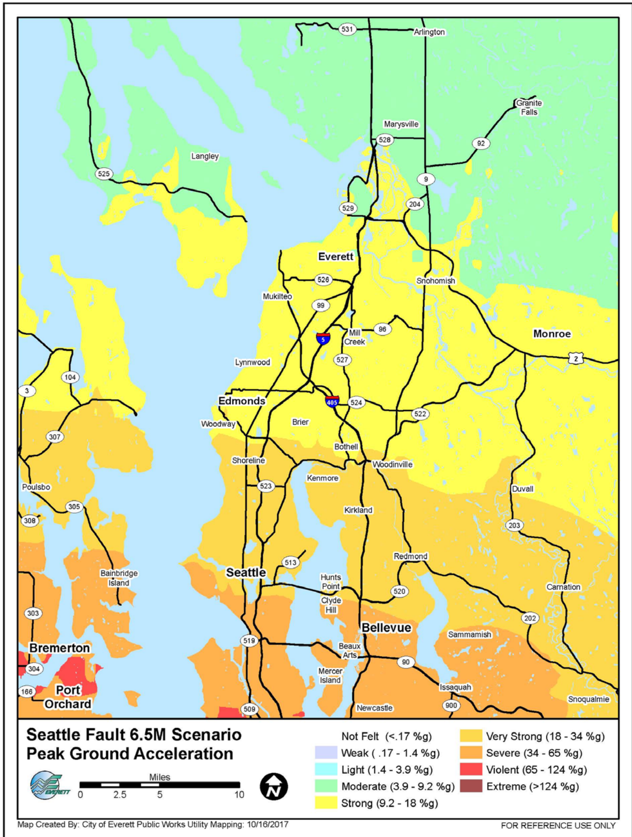
FIGURE 12: SEATTLE FAULT 6.5 SCENARIO PEAK GROUND ACCELERATION
