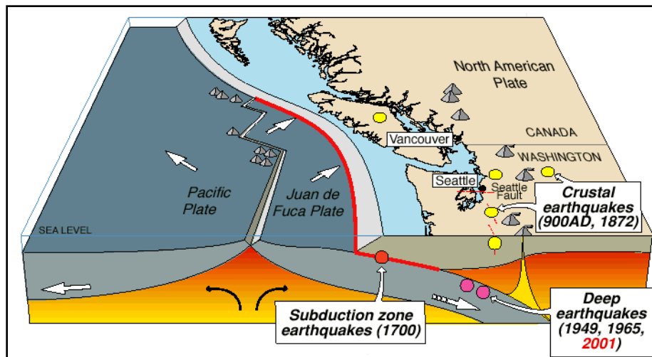
FIGURE 3: EARTHQUAKE TYPES IN WESTERN WASHINGTON
