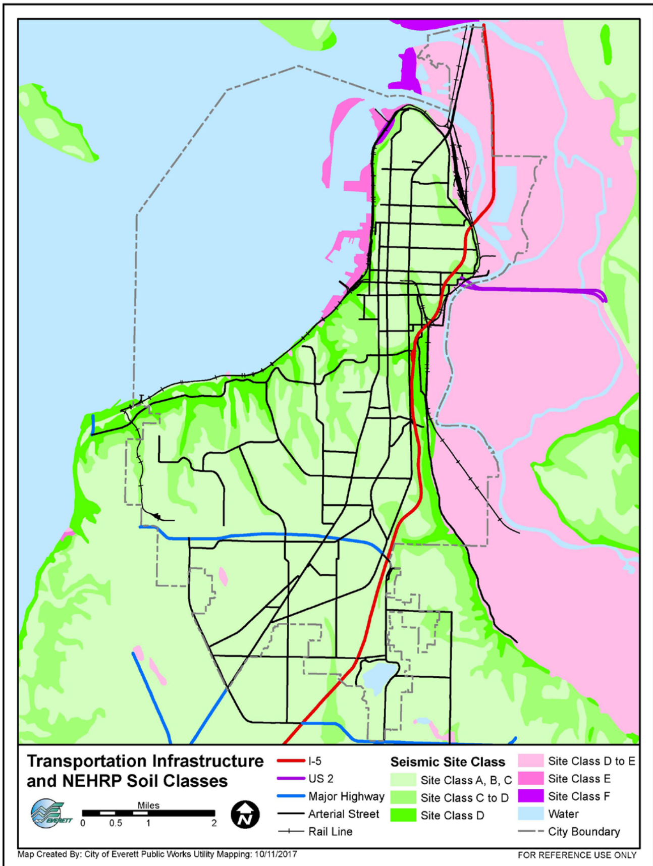
FIGURE 10: NEHRP SOILS IN EVERETT AND EXPOSED TRANSPORTATION INFRASTRUCTURE
