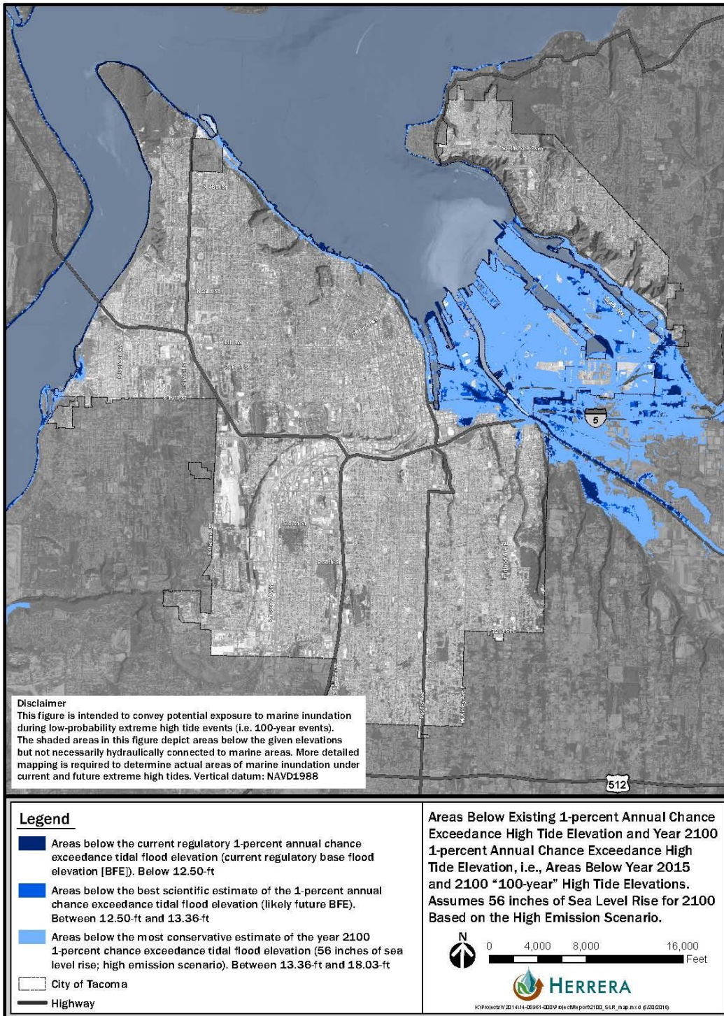
Figure 4. Potential flooding area during extreme high tides in 2100 using the high emissions scenario.
