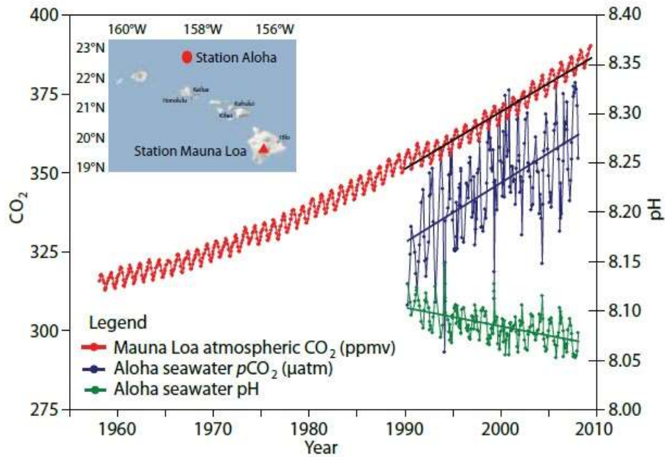
Figure 8. Time series of atmospheric CO 2 at Mauna Loa (in parts per million volume, ppmv; red), surface ocean pCO 2 (µatm; blue) and surface ocean pH (green) at Ocean Station ALOHA in the subtropical north Pacific Ocean. Note that the increase in oceanic CO 2 over the past 17 years is consistent with the atmospheric increase within the statistical limits of the measurements. Figure and caption source: Doney et al. 2009 [42]. As of the time of this writing (March 2017), CO 2 at Mauna Loa is now over 400 ppm (www.co2.earth/daily-co2).
