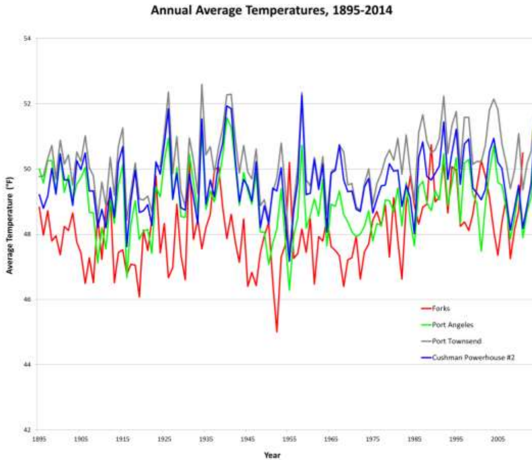
Figure 3. Average annual temperatures at weather stations on the Olympic Peninsula. Data recorded from 1895 to 2014. Data source: Office of the Washington State Climatologist, www.climate.washington.edu .
