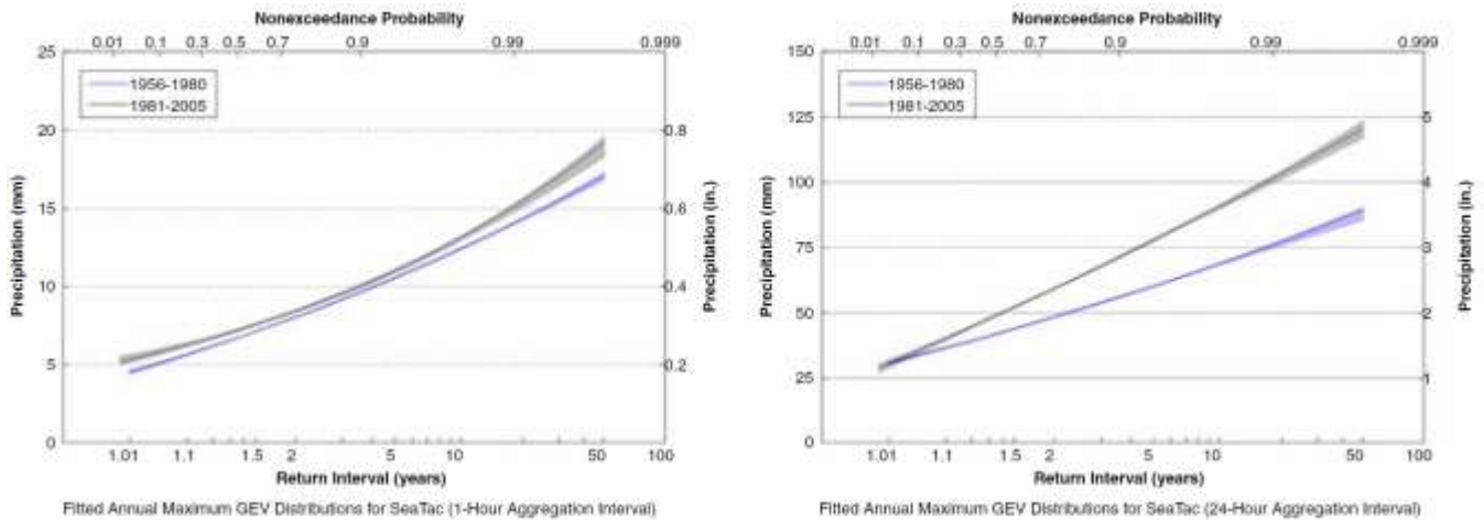
Figure 2. Changes in fitted 1-hour (left) and 24-hour (right) annual maximum precipitation distributions for Sea-Tac Airport from 1956–1980 (purple line) to 1981–2005 (gray line). GEV stands for Generalized Extreme Value. Uncertainty bounds are indicated by the shaded areas. Both figures show an increase in the 1-hour and 24-hour rain events, although none of the changes was found to be statistically significant at the 95% confidence interval (the 24-hour distributions at Sea-Tac were statistically significant at the 90% interval). Figures and caption adapted from Rosenberg et al. 2010, Figure 2 [10].
