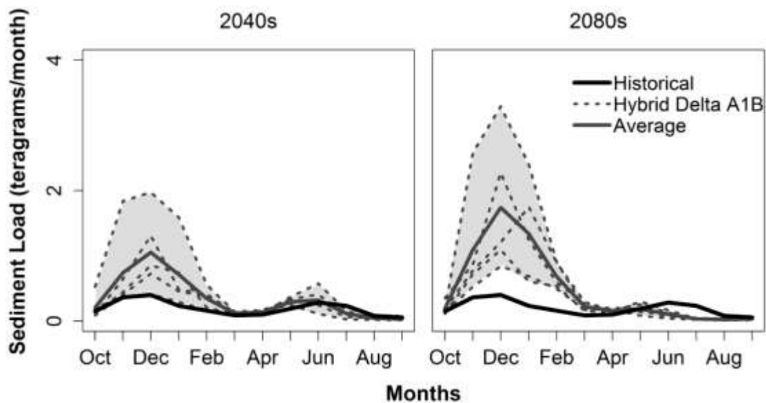
Figure 18. Simulated monthly average sediment loading for the Skagit River near Mount Vernon for the 2040s (left) and 2080s (right). Figure source: Lee et al. 2016 [65].
