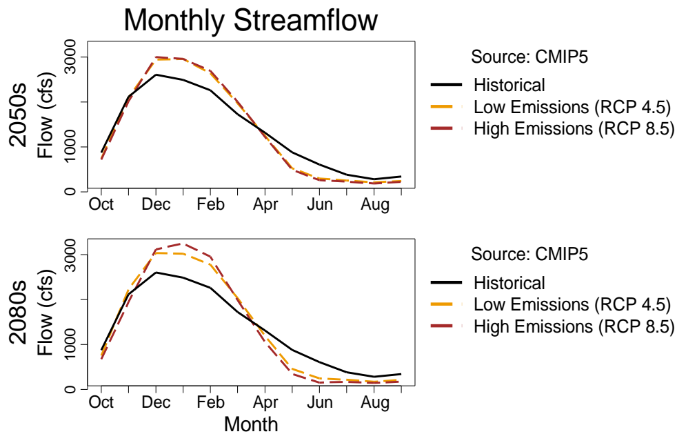
Figure 16. Monthly graph of streamflow for the Skokomish River. Estimates of the monthly average flow are based on the water year, starting in October and ending in September. Changes are shown for two time periods: the 2050s (top) and the 2080s (bottom). Figure source: Climate Impacts Group.
