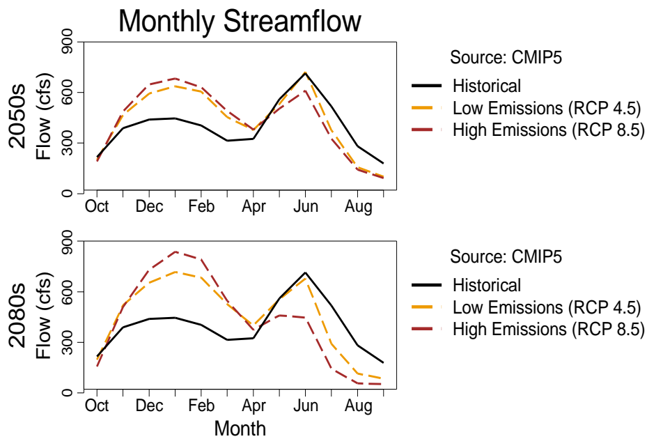
Figure 15. Monthly graph of streamflow for the Dungeness River. Estimates of the monthly average flow are based on the water year, starting in October and ending in September. Changes are shown for two time periods: the 2050s (top) and the 2080s (bottom), for both a low (RCP 4.5, yellow line) and a high (RCP 8.5, red line) emissions scenario. All changes are relative to average historical flows (black). Figure source: Climate Impacts Group.
