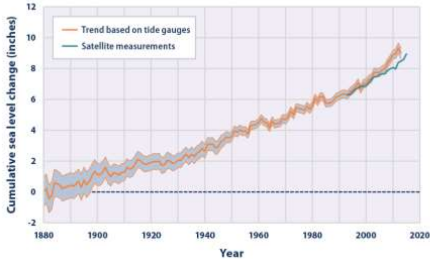
Figure 5. Observed change in global sea level, 1880–2015. The figure shows the change in average absolute sea level change, which refers to the height of the ocean surface regardless of whether nearby land is rising or falling. Since 1880, global sea level has risen over 8 inches. The shaded band shows the likely range of values, based on the number of measurements collected and the precision of the methods used. Figure source: U.S. Environmental Protection Agency, based on data from CSIRO 2015 and NOAA 2016 [30, 31, 32].
