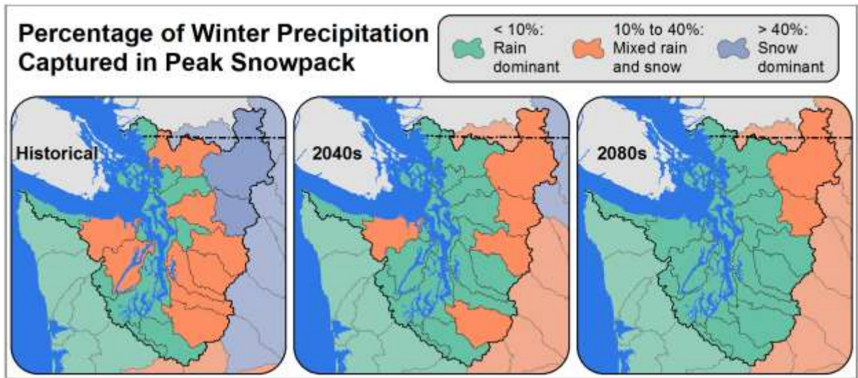
Figure 17. Current and future watershed classifications, based on the proportion of winter precipitation stored in peak annual snowpack. Map compares average historical conditions (1970–1999) and average projected future conditions for 10 global models, 2 time periods: the 2040s (2030–2059) and the 2080s (2070–2099) and a moderate greenhouse gas scenario (A1B). By the end of the 21 st century, Puget Sound will no longer have any snow-dominant watersheds, and only a few remaining that can be classified as mixed rain-and-snow. Data source: Hamlet et al., 2013 [60].
