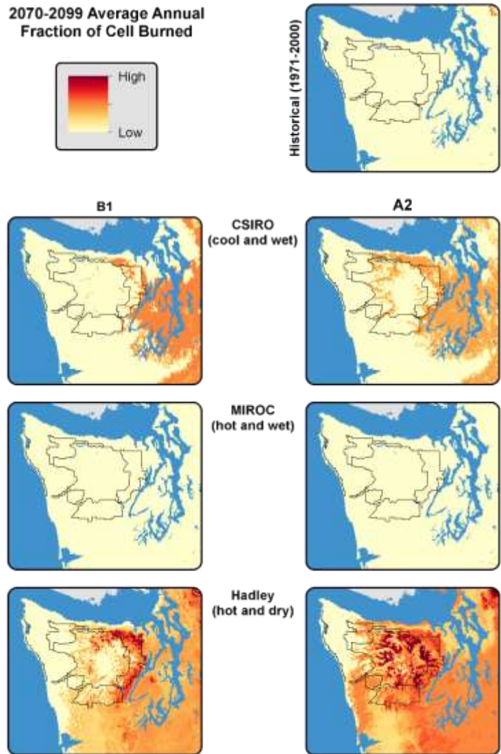
Figure 19 (at right). Projected average annual fraction of cell burned on the Olympic Peninsula for the 2070–2099 time period compared to modeled historical fire activity. This output is derived by averaging the area of a cell that is burned over the period of interest. Numbers are not shown in the legend because they are not intuitive. However, darker colors indicate more fire. Projections are from the MC1 model for three global climate models (GCMs) (rows) and two Intergovernmental Panel on Climate Change carbon dioxide emissions scenarios (columns). The B1 emissions scenario is characterized by relatively low future emissions, and the A2 scenario is characterized by relatively high future emissions. Olympic National Park and Olympic National Forest are outlined in black. CSIRO = Commonwealth Scientific and Industrial Research Organization; MIROC = Model for Interdisciplinary Research on Climate. (Data from R. Neilson and the MAPSS Team, USDA Forest Service and Oregon State University, Corvallis, Oregon.) Figure and caption source: Halofsky et al. 2011 [90].
