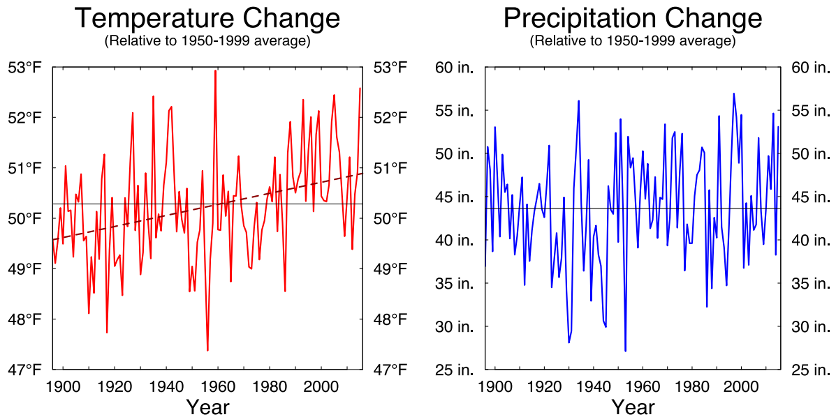
Figure 1. Temperature is rising in the Puget Sound lowlands, but there is no long-term trend in annual precipitation. Average annual air temperature (left, red, in °F) and total annual precipitation (right, blue, in inches) for the Puget Sound Lowlands climate division, shown relative to the average for 1950-1999 (black horizontal line in both graphs, corresponding to 50.3°F for annual average temperature and 43.6 inches for annual total precipitation). The dashed line in the temperature plot is the fitted trend, indicating a warming of +1.3°F (range: +0.7°F to +1.9°F) from 1895 to 2014. The trend for precipitation is not statistically significant and therefore is not shown. Figure source: Climate Impacts Group, Data source: Vose et al. 2014 [3].
