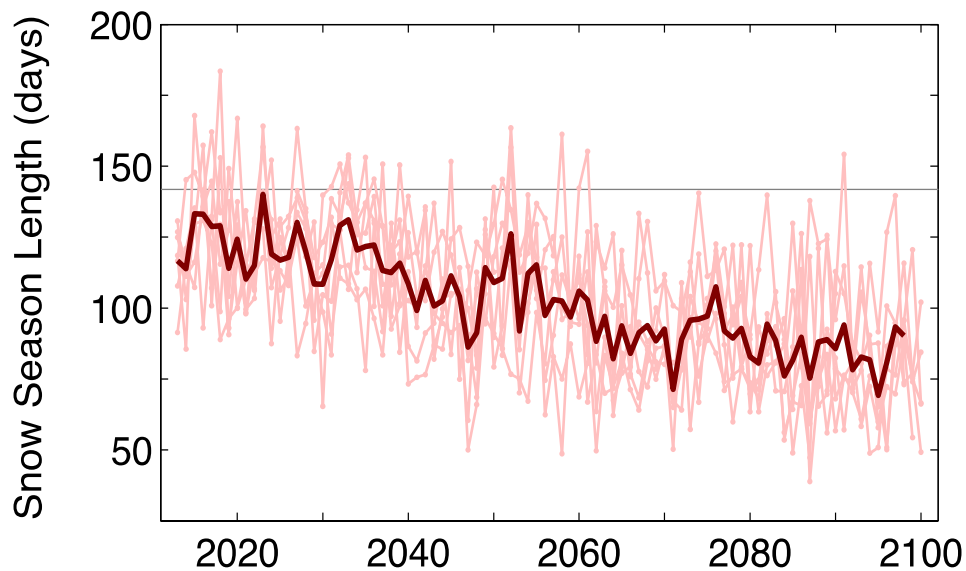
Figure 14. Shorter snow season with warming; large year-to-year variability. Projected length of the snow season, in days, for middle elevations (4,000 to 5,000 feet) for the Cascade Mountains in Oregon and Washington. The plot shows projected snow season length from seven individual climate models (thick pink lines) and the average among all models (thick red line) for a medium greenhouse gas scenario (A1B). For comparison, the average snow season length for 1950-1999 was 142 days (shown as the gray horizontal line). Although the length of the snow season is clearly expected to decrease significantly over this century, individual years with substantially longer or shorter snow seasons than the general declining trend are also expected to occur. 20 Data source: Hamlet et al. 2013 [60].
