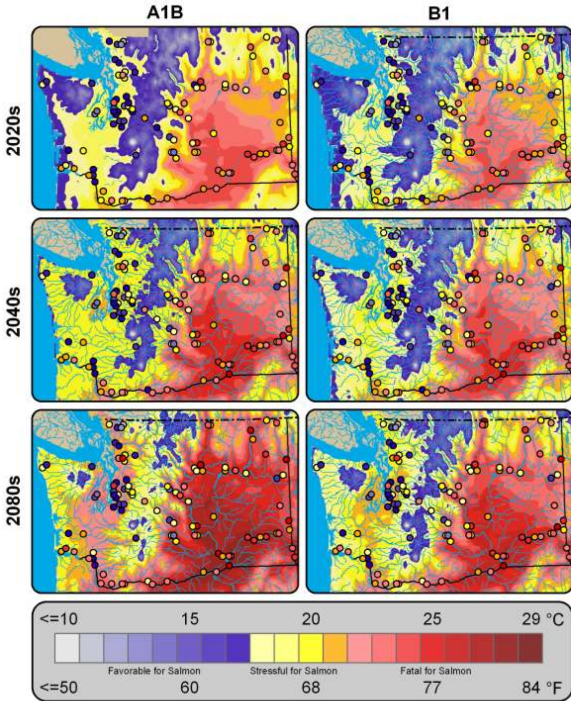
Figure 29. August mean surface air temperature (colored patches) and maximum stream temperature (dots) in Washington State. Source: University of Washington Climate Impacts Group.
