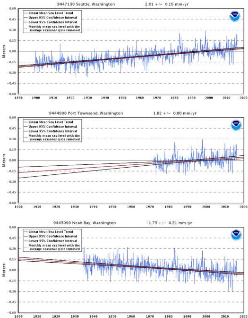
Figure 6. Monthly mean sea level trends for the Seattle (top), Port Townsend (middle), and Neah Bay (bottom) tide gauges. Each plot shows the linear trend (red line), the 95% confidence interval (black lines), and the monthly mean value. The mean sea level trend for Seattle (1899–2015) is +2.01 millimeters per year with a 95% confidence interval of \pm 0.15 mm/year (equivalent to a change of 0.66 feet in 100 years). The mean sea level trend for Port Townsend (1972–2015) is +1.82 mm/year with a 95% confidence interval of \pm 0.80 mm/year (equivalent to a change of 0.60 feet in 100 years). The mean sea level trend for Neah Bay (1934–2015) is -1.73 mm/year with a 95% confidence interval of \pm 0.31 mm/year (equivalent to a change of -0.57 feet in 100 years). Trends exclude the regular seasonal fluctuations due to coastal ocean temperatures, salinities, winds, atmospheric pressures, and ocean currents. Figure and trends source: NOAA Tides and Currents, https://tidesandcurrents.noaa.gov/sltrends/sltrends.html .
