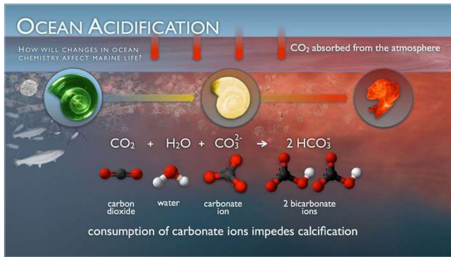
Figure 7. Ocean acidification occurs when carbon dioxide, which is being released at increasingly higher levels as a result of human activities, is absorbed by the ocean. When mixed with seawater, carbon dioxide chemically changes into carbonic acid. Carbonic acid lowers the ocean’s pH level, nudging it toward acidity. Carbonic acid also increases the water’s hydrogen ion concentration, ultimately limiting the availability of carbonate ions (a key component of calcium carbonate) for building and maintaining hard body parts, such as shells. Figure source: NOAA PMEL.
