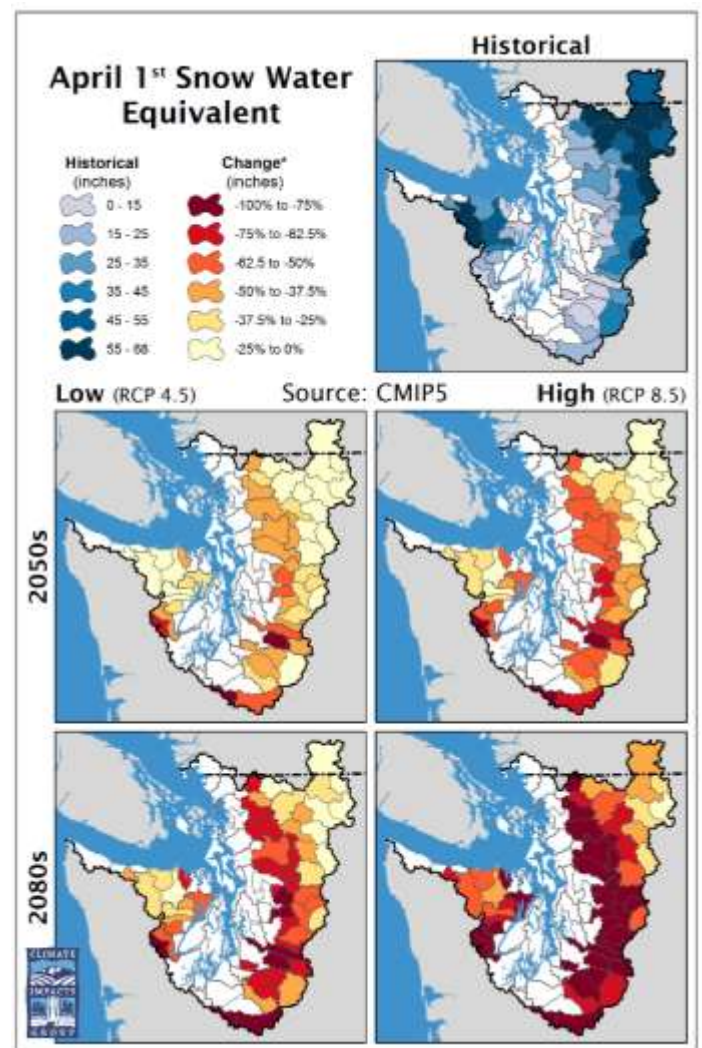
Figure 13 (at right) Projected changes in April 1 st Snow Water Equivalent (SWE) for the HUC-10 scale. Maps show the historical and projected April 1 st SWE, a measure of the total amount of water contained in the snowpack. The figure compares watershed averages for historical conditions (1970–1999, in inches) and the projected change (in percent) for 10 global models. Two time periods are considered: the 2050s (2040–2069) and the 2080s (2070–2099), based on a low (RCP 4.5) and a high (RCP 8.5) greenhouse gas scenario. Results are only shown for watersheds with an average historical April 1 st SWE of at least 0.4 inch. White to dark blue shading on the historical map indicates areas which received highest levels of April 1 st SWE in Puget Sound. Projected decreases in SWE are depicted by the yellow to red shading. Figure created by Robert Norheim, Climate Impacts Group, based on CMIP5 projections used in the IPCC 2013 report [27]. Data source: Mote et al. 2015 [45].
