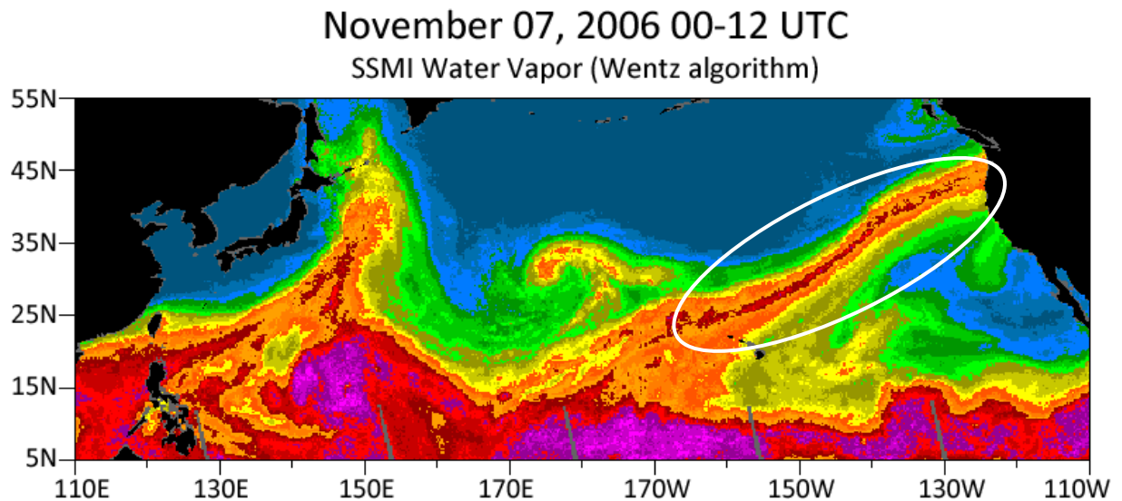
Figure 12. Satellite view of the Pacific region showing an atmospheric river (circled in white) originating in the tropical Pacific Ocean on November 7, 2006. Brighter colors indicate areas where the atmosphere is holding more moisture. Figure source: NOAA.
