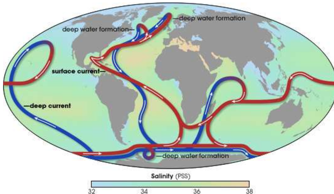
Figure 22. Thermohaline circulation, the global conveyor belt of ocean currents that influence the Earth's climate [123].
