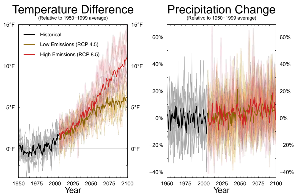
Figure 9. All scenarios project warming in the Puget Sound region for the 21 st century; projected changes in annual precipitation are small compared to year-to-year variability. The graphs show average yearly air temperature and precipitation for the Puget Sound region, relative to the average for 1950–1999 (horizontal gray line, corresponding to an annual average temperature of 44°F and an annual total precipitation of 78 inches). The black line shows the average simulated air temperature or precipitation for 1950–2005, based on the individual model results indicated by the thin gray lines. The thick colored lines show the average among model projections for two emissions scenarios (low: RCP 4.5, and high: RCP 8.5; see Section 1), while the thin colored lines show individual model projections for each scenario. Figure source: Climate Impacts Group, using downscaled climate projections developed by Abatzoglou and Brown (2011) [27, 45].
