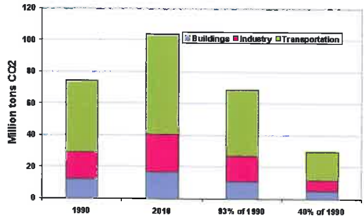
Projected Carbon Emissions to 2010, Washington State Source: James D. Kerstetter, "Greenhouse Gas Emissions in Washington State: Sources and Trends," Washington State University Cooperative Extension Energy Program for Washington State Community, Trade and Economic Development, Energy Policy Group, 1999 http://www.cted.wa.gov/energy/archive/papers/wa-ghg09.htm
