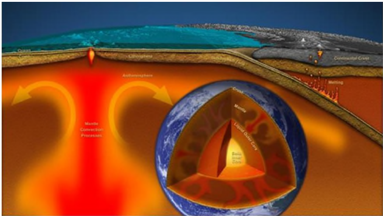
Figure 5. The Subduction Process 11 (Image provided courtesy of the NEPTUNE Project, specializing on studies of the northeast Pacific Ocean off the Washington and Oregon coasts)
