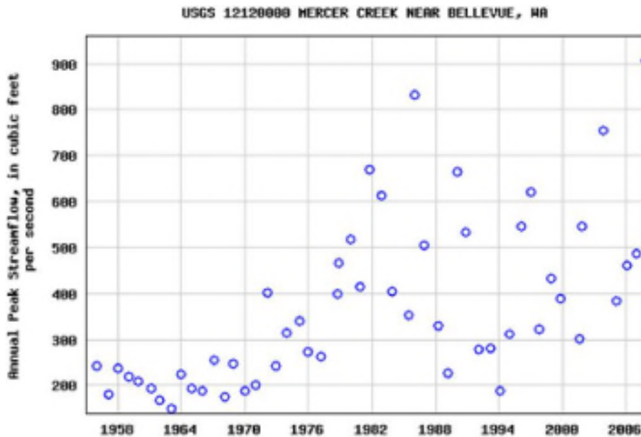
Figure 5. USGS Fact Sheet 229-96 "100 Year Flood" https://pubs.usgs.gov/fs/FS-229-96/pdf/FS_229-96.pdf
