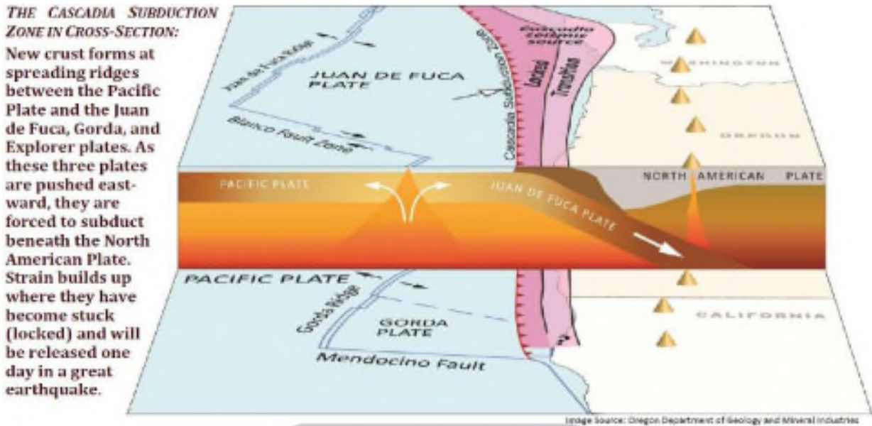
Figure 4. Cascadia Earthquake Sources 10
