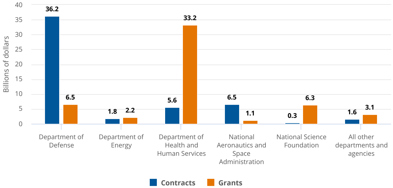
Federal obligations for extramural R&D, by agency and type of agreement: FY 2022
