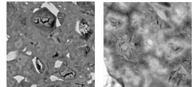
Ettringite cores forming into aged cement pastes. Right picture is a 2 years old paste subjected to sulfate attack. One clearly sees the ettringite cores forming within the C-S-H.
