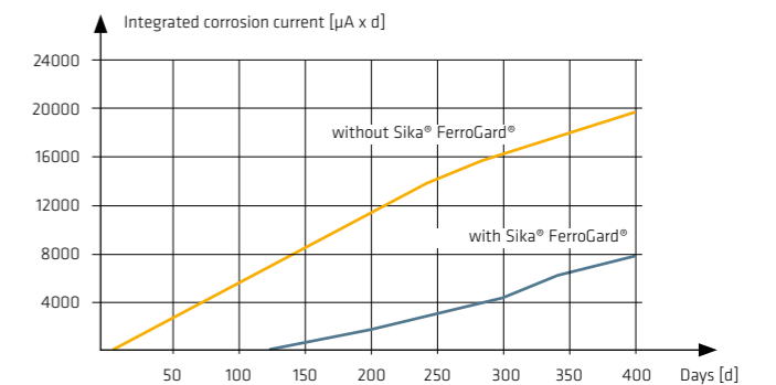
The Sika Research Department in Zurich tested the anticorrosive effect of Sika® FerroGard® on cracked concrete beams. The specimens were produced in accordance with ASTM G 109 and were cyclically treated with road salts. Periodic measurement of the corrosion current confirms the protective effect of Sika® FerroGard®.
