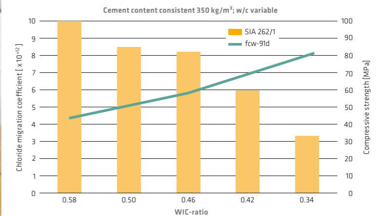
Figure 6: Concrete tests according to SIA 262/1 Annex B (similar to NT BUILD 492)
