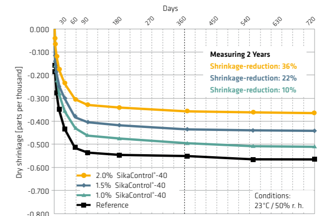
Shrinkage behavior of concrete containing shrinkage-reducing admixtures, measured 2 years to complete abatement of shrinkage due to drying.
