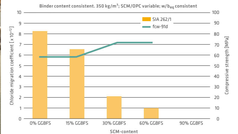
Figure 7: Concrete tests according to SIA 262/1 Annex B (similar to NT BUILD 492)
