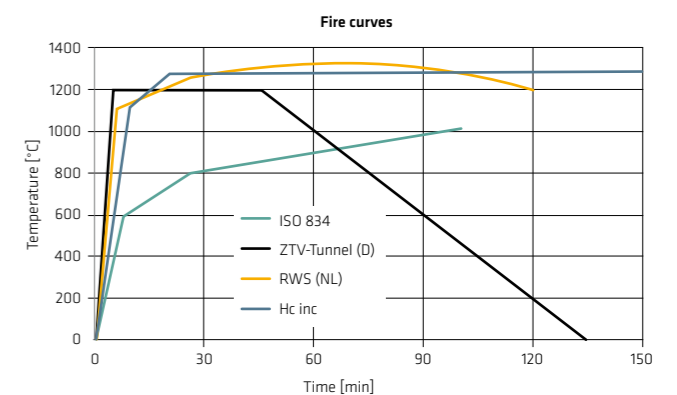
These fire exposure rating curves all simulate the temperature profile of a tunnel fire. The example of the RWS curve defines the maximum exposure which can be expected in the worst case scenario: Defined as a fire of a tank truck with a load capacity of 50m 3 which is 90% full of liquid hydrocarbon fuel (petrol).
