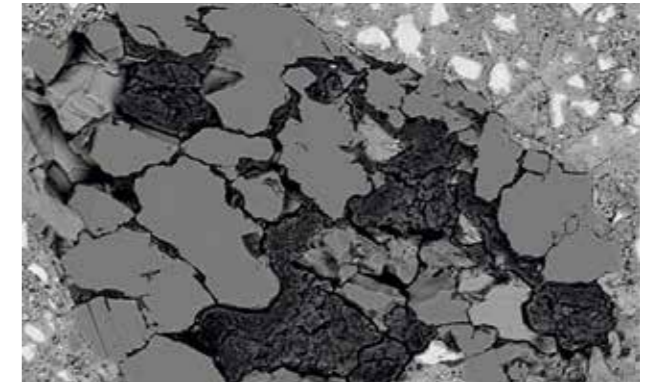
Amorphous silica spots within the aggregate have reacted with alkali ions and formed a gel that expanded upon ingress of water. The aggregate has subsequently swelled and cracked while the amorphous region (black cracked masses) expanded.
