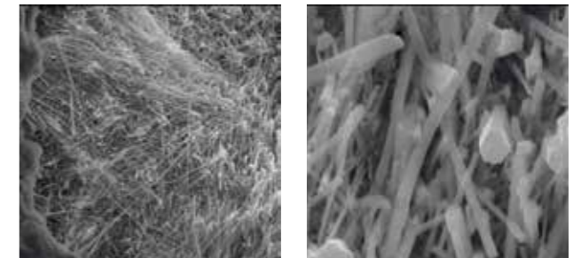
Classic form of sulfate attack associated with ettringite or gypsum formation. Flurry of ettringite rods grown in mature cement pastes subjected to external sulfate solutions.
