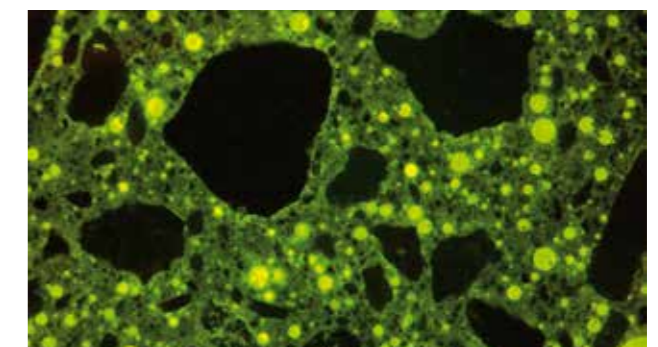
Artificially introduced air voids, caused by an air entrainer, generate space for expansion in the concrete structure to allow for the roughly 10% increase in volume when water freezes to become ice. In test BE II according to D-R 400, the test prisms are subject to alternating loads between +20°C and -20°C, the change in length is measured and judged between three ranges of durability (low / middle / high). Calculation according to ASTM C666.
