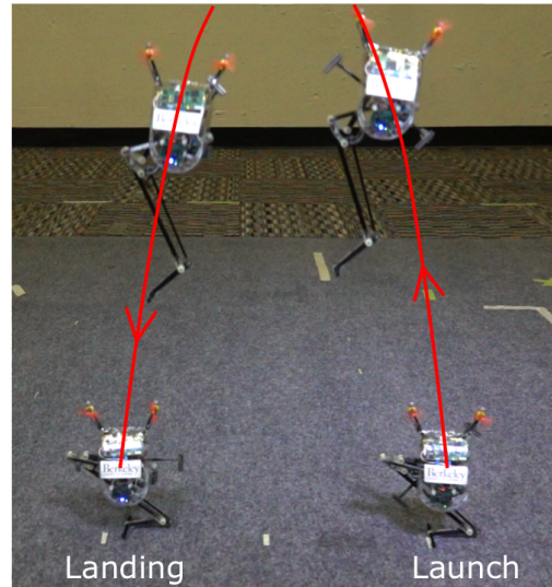
Fig. 1: Salto-1P leaps and lands.
