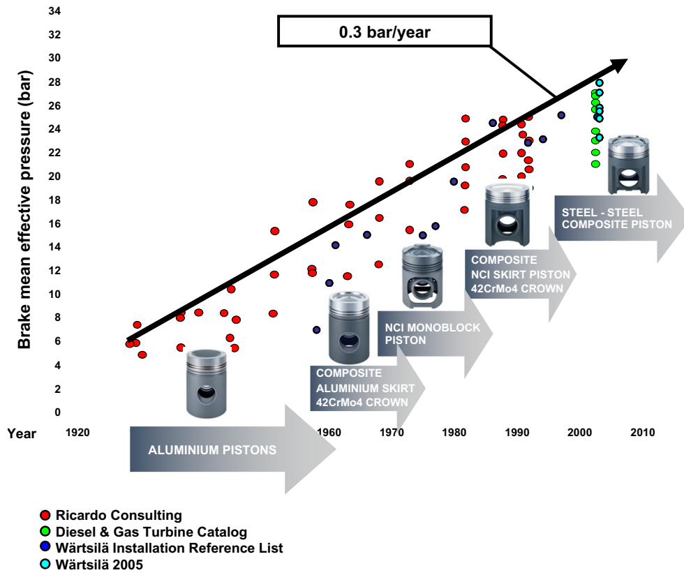
Figure 15: Moore's Law for Pistons: The Quality Trend of Diesel Engines and Piston Materials.
