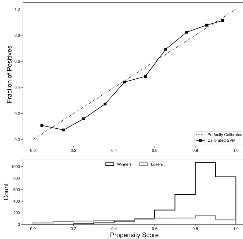
Figure 4: The Text Propensity Score Calibration Plot.
