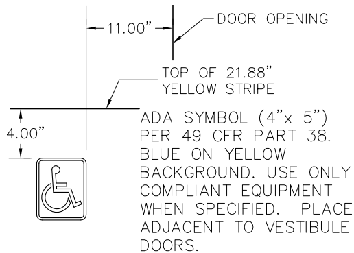
DETAIL C NO SCALE
