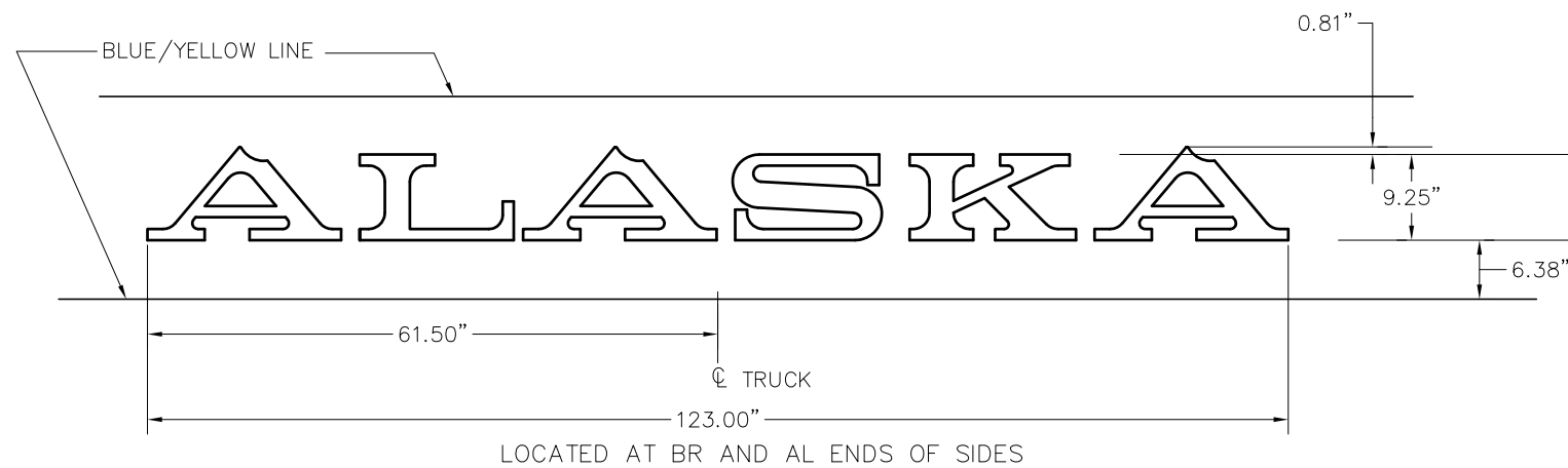
DETAIL B NO SCALE
