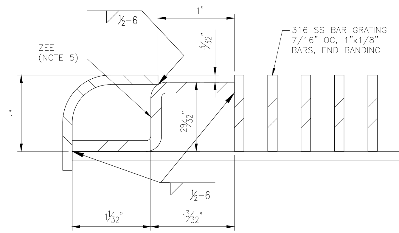
NOSING WELD DETAIL SCALE: NTS
