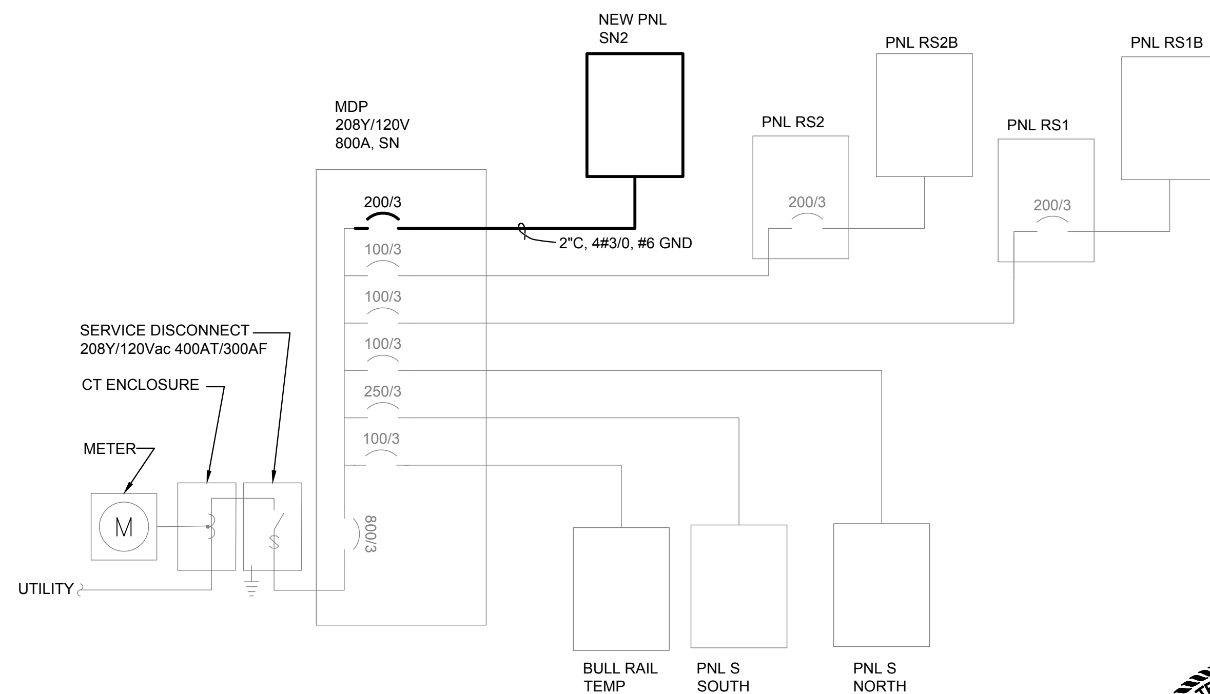
POWER ONE-LINE DIAGRAM E-1 NTS
