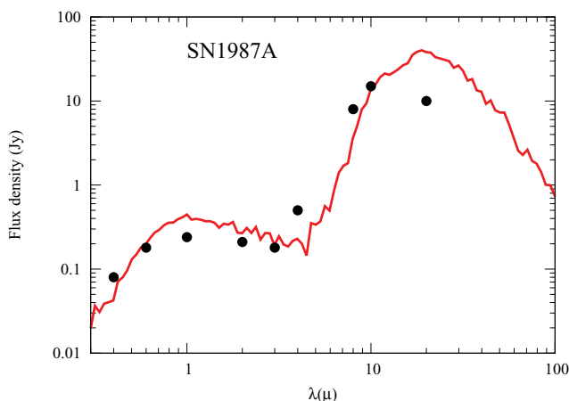
Figure 1. IR flux emitted by our modelled dust composition and mass for a 19 M ⊙ progenitor at day 615 post-explosion. The IR flux data of SN1987A at 615 days are shown.
