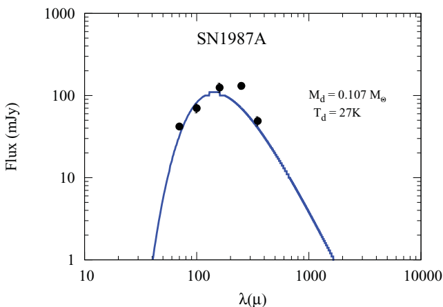
Figure 2. Submm flux emitted by our modelled dust composition and mass for a 19 M ⊙ progenitor. The dust temperature is 27 K. The submm dust flux data from Herschel are also shown.
