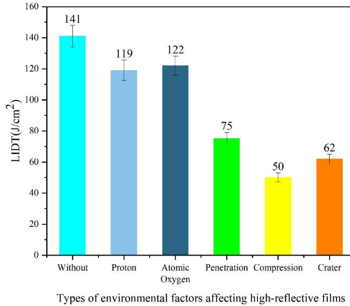
Fig. 4. A comparison of LIDTs for high-reflection films under the action of single space environmental factors. ('Without' presents without any space environmental factors)
