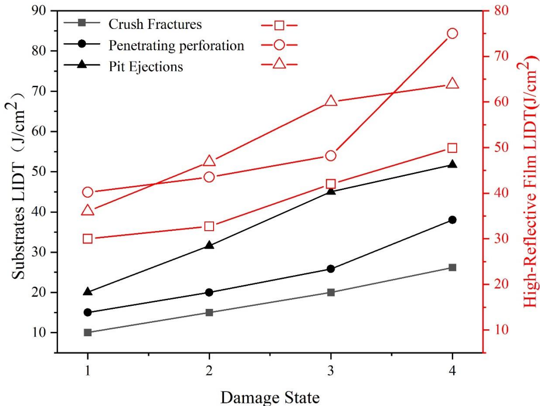
Fig. 3. LIDT results for different states in 30 \mu\text{m} substrates and high-reflection films. (1: Initial damage morphology; 2: Damage to the membrane around the hole; 3: Bright spots appearing around the hole; 4: Extensive damage centered around the hole.)
