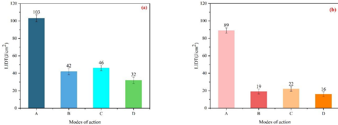
Fig. 7. A comparison of LIDT values for simulated fragment compressions in (a) high-reflectance films and (b) substrates. A: Protons & Atomic Oxygen; B: Protons & Penetration; C: Atomic Oxygen & Penetration; D: Protons & Atomic Oxygen & Penetration.
