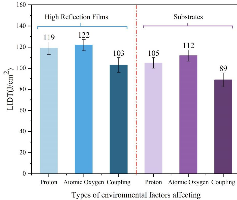
Fig. 6. A comparison of LIDT values produced by the coupled effect of atomic oxygen and protons.
