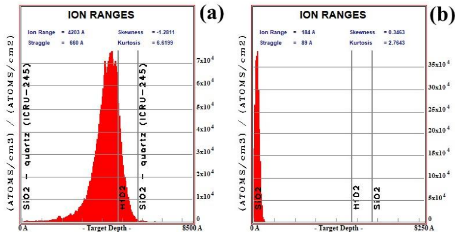
Fig. 9. SRIM simulations of proton concentrations and atomic oxygen distributions within the membrane layer. (a) Protons; (b) Atomic oxygen.
