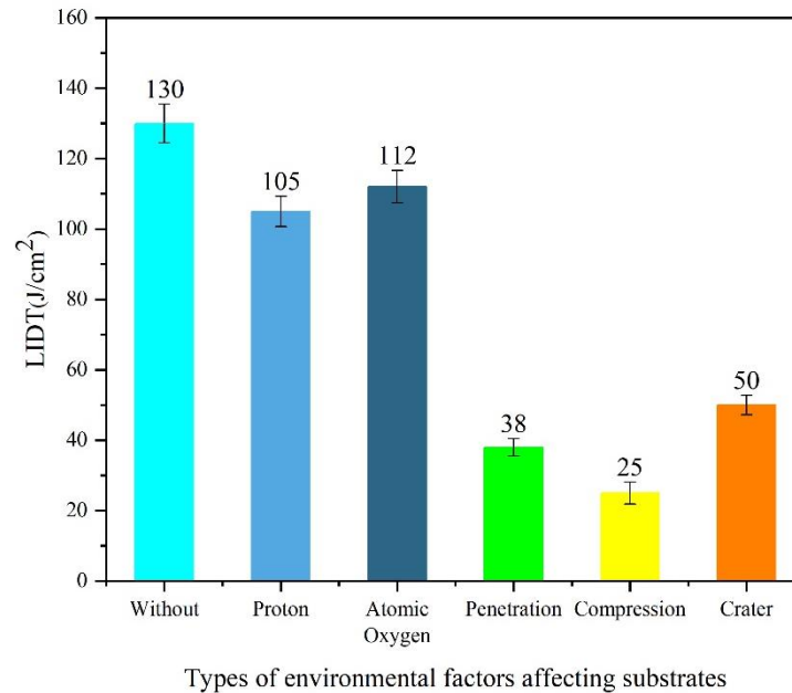
Fig. 5. A comparison of LIDTs for substrates under the action of single space environmental factors. ('Without' presents without any space environmental factors)
