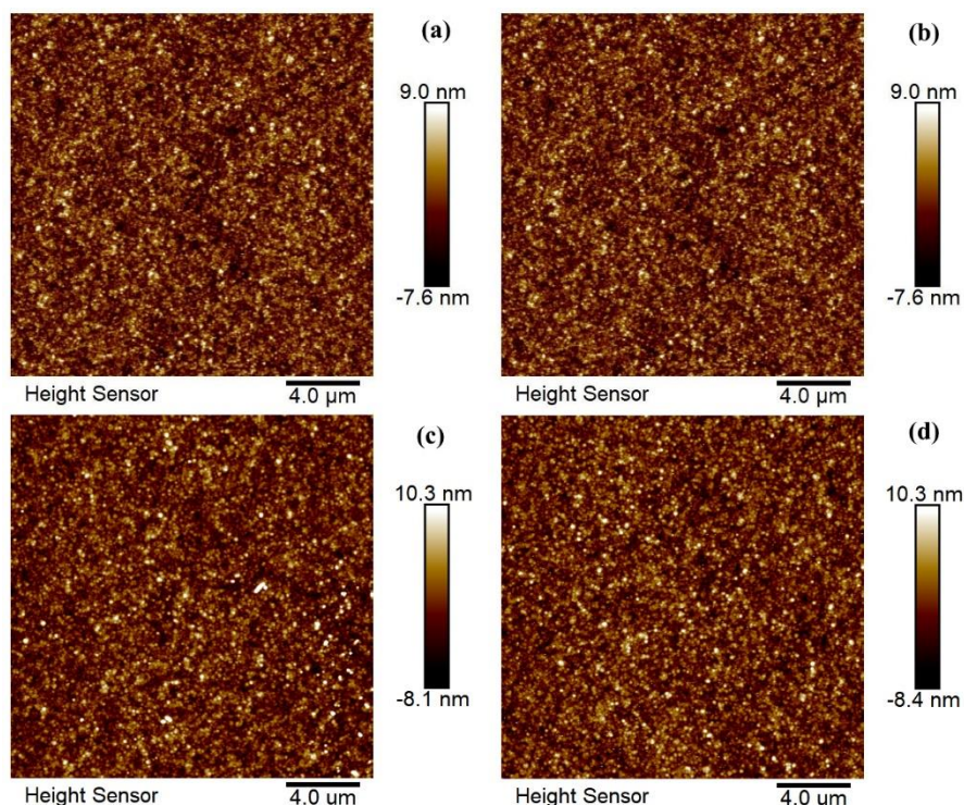
Fig. 8. Surface morphology images of three-band high-reflectance thin films before and after proton and atomic oxygen irradiation. (a) Before proton irradiation; (b) After proton irradiation; (c) Before atomic oxygen irradiation; (d) After atomic oxygen irradiation
