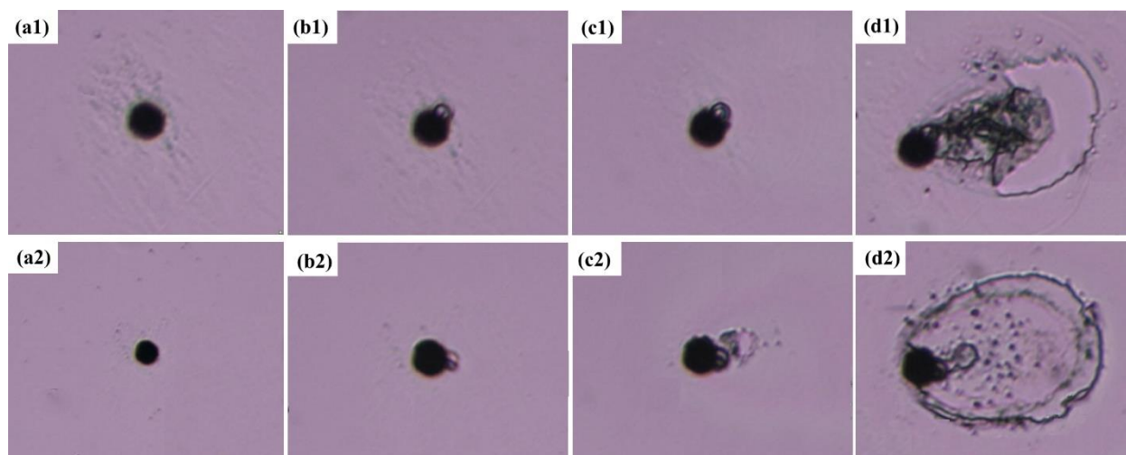
Fig. 2. Damage condition of high-reflectance thin film (1 series) and substrate (2 series) samples (a) Initial damage morphology; (b) Damage to the membrane around the hole; (c) Bright spots appearing around the hole; (d) Extensive damage centered around the hole.
