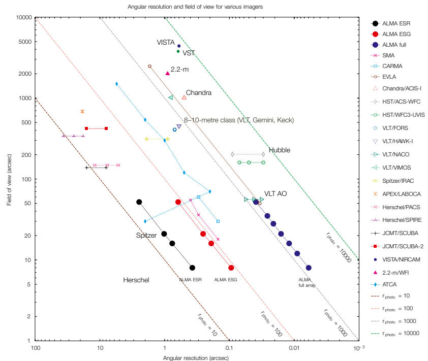
Figure 6. Effective angular resolution plotted against the field of view for a selection of different imagers.
