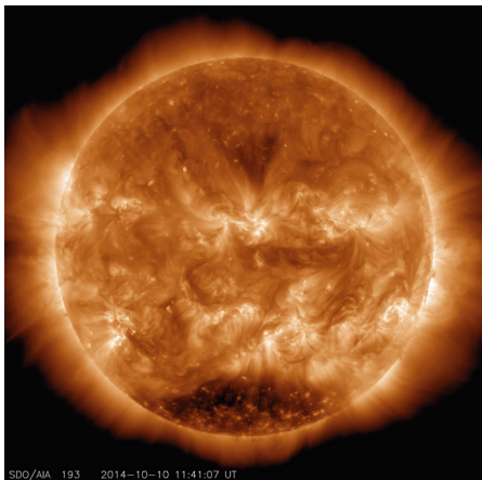
Figure 1. The Sun in the extreme ultraviolet, imaged by NASA's Solar Dynamics Observatory on 10 October 2014. This wavelength highlights the outer atmosphere of the Sun (corona) and active solar regions, which appear bright in the image. Solar flares and coronal mass ejections would also be highlighted in this channel. Credit: Image courtesy of NASA/SDO and the AIA, EVE, and HMI science teams
