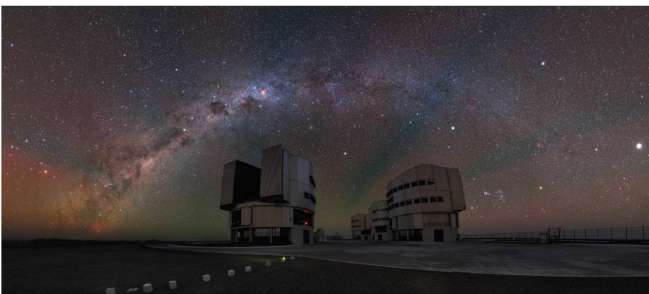
Figure 3. This Ultra HD photograph shows almost the full VLT platform with the red shades of airglow visible overhead. Credit: ESO/Y. Beletsky (LCO)
