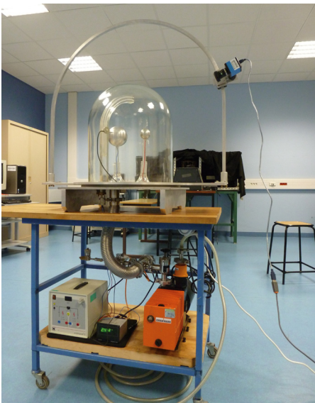
Figure 2. Planeterrella III. Credit: J. Liljensten
