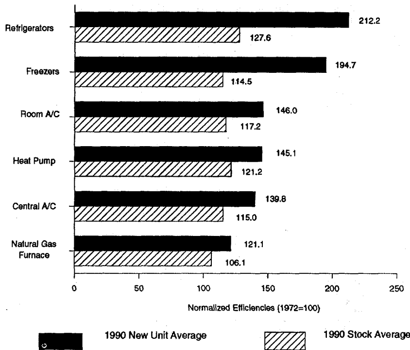
Figure 8. Comparison of 1990 Average Stock Efficiencies with 1990 New Unit Efficiencies
