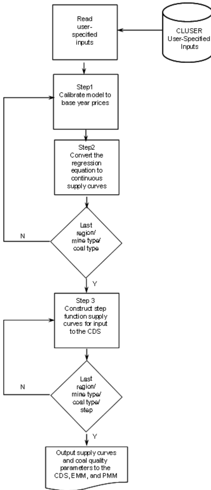
Figure 1. 5. CPS flowchart
