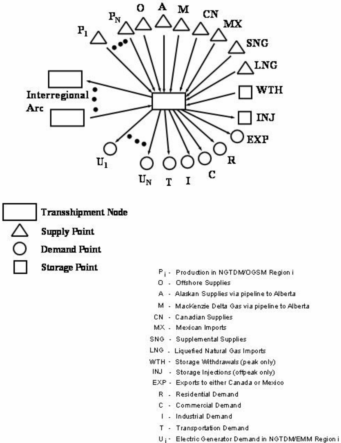
Figure 3-2. Transshipment Node
