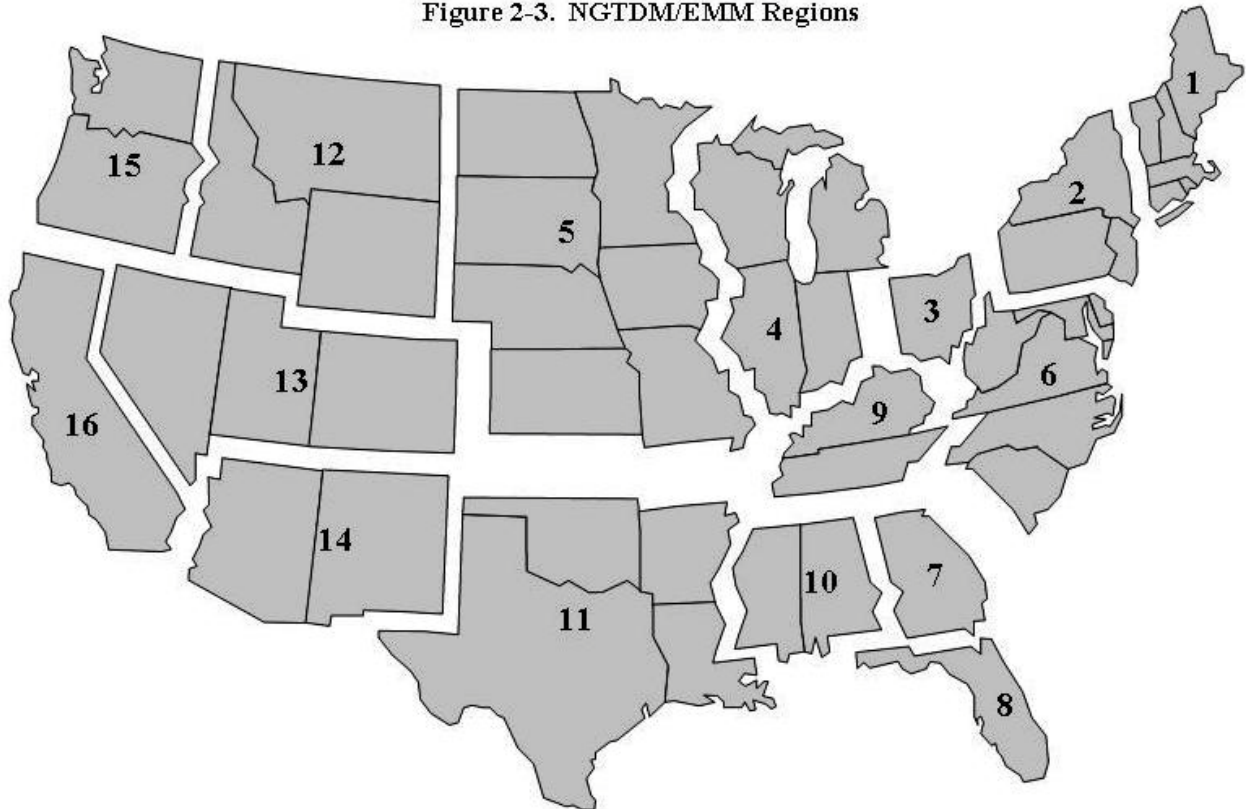
Figure 2-3. NGTDM/EMM Regions
