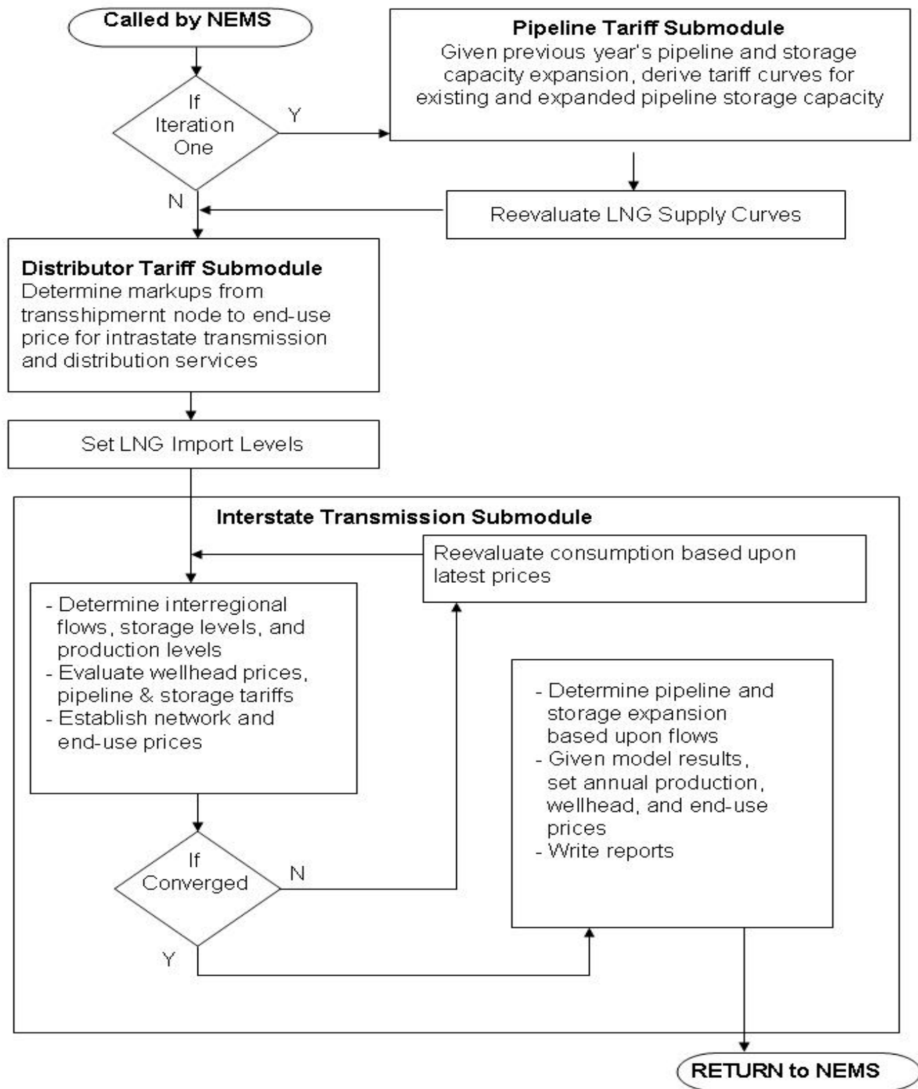
Figure 3-4. NGTDM Process Diagram
