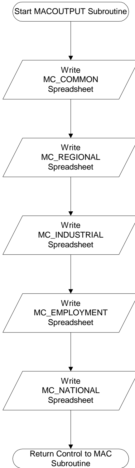
Figure 16. Subroutine MACOUTPUT
