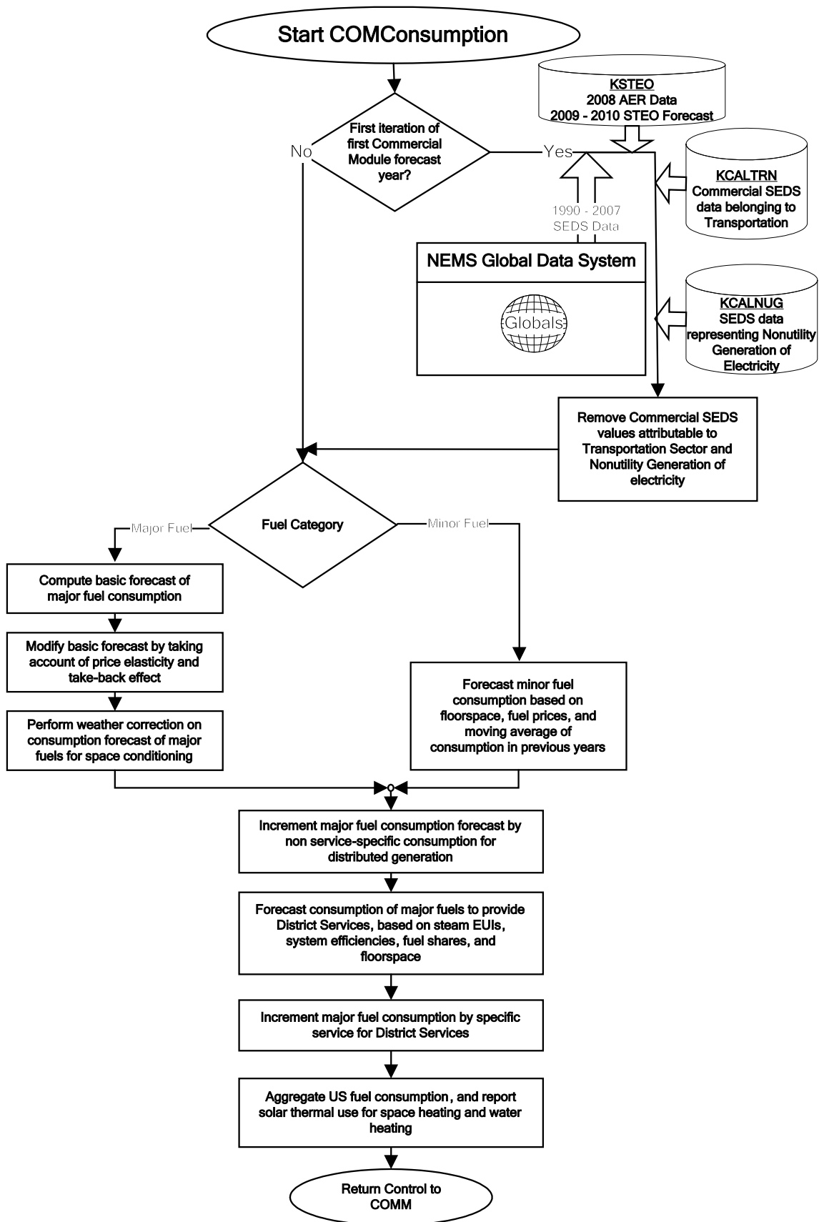
Figure 8. COMConsumption Calculation Process Flow
