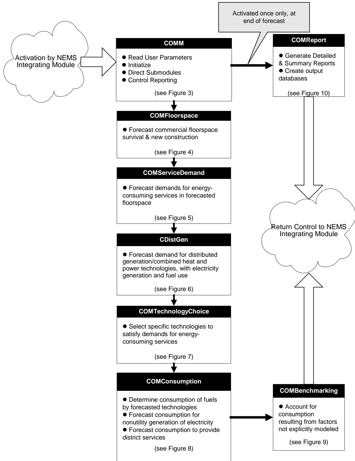
Figure 2. Commercial Module Structure & Fundamental Process Flow
