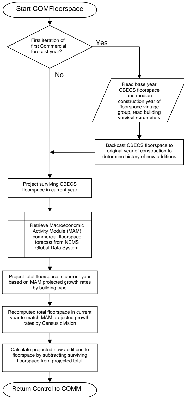
Figure 4. COMFloorspace Calculation Process Flow
