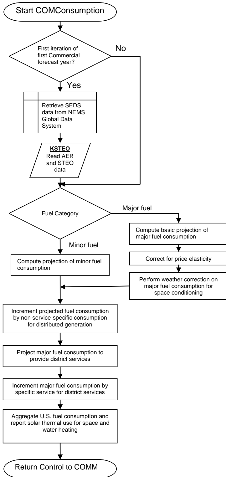
Figure 8. COMConsumption Calculation Process Flow
