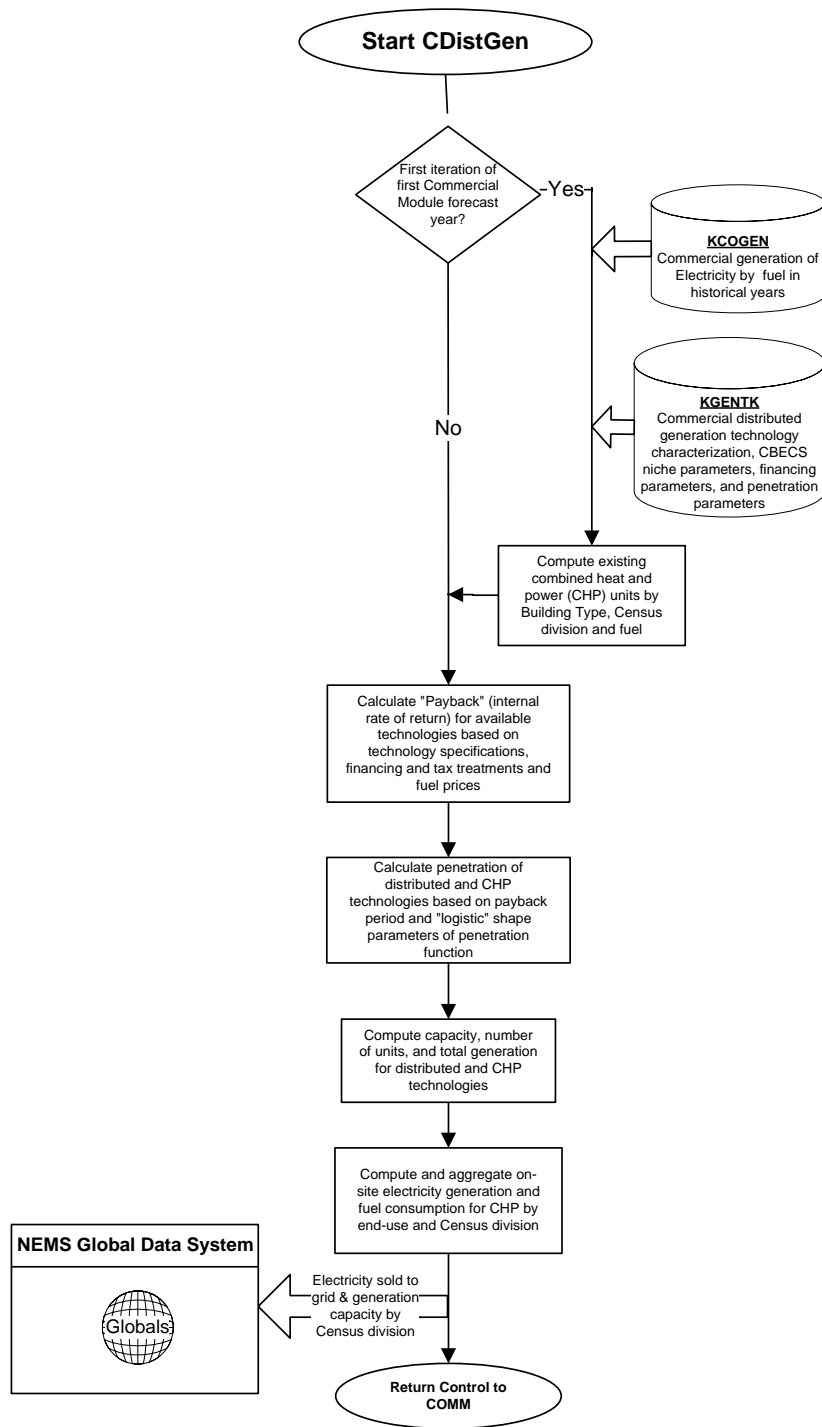
Figure 6. CDistGen Calculation Process Flow
