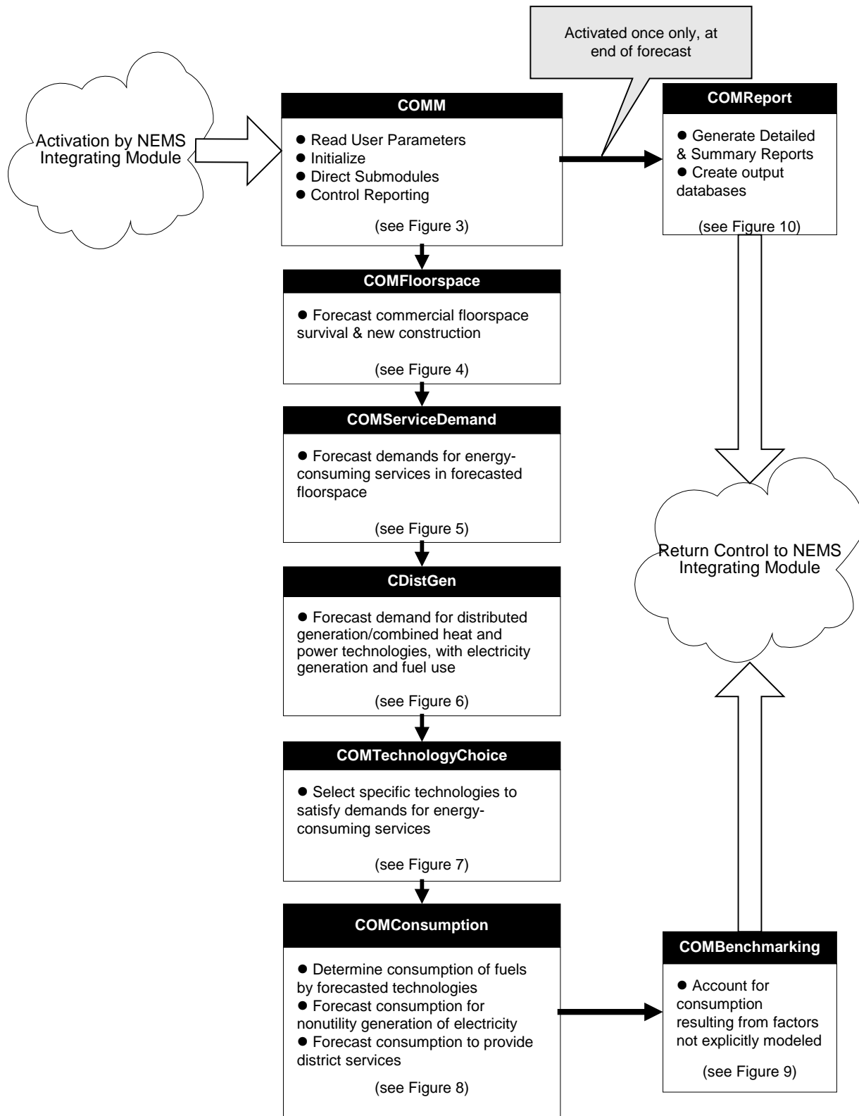
Figure 2. Commercial module structure &amp; fundamental process flow
