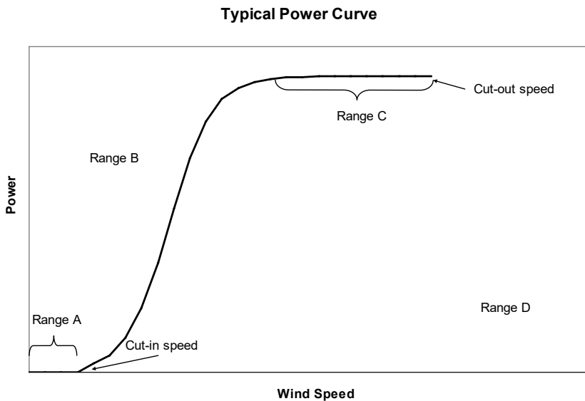
Figure 2. Power output from a typical wind turbine as a function of ambient wind speed
