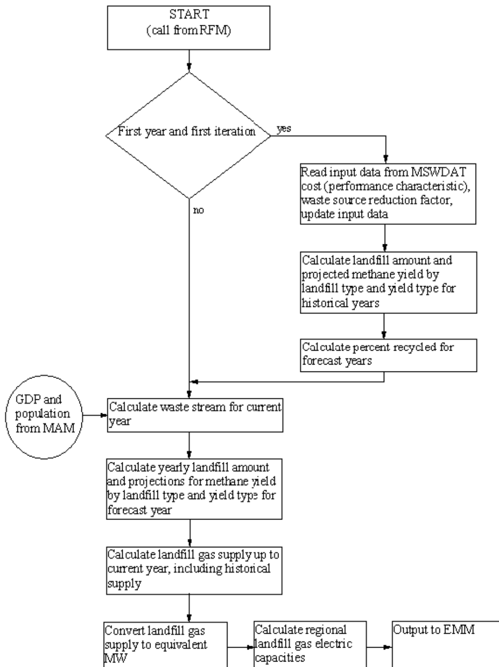
Figure 4. Landfill Gas Submodule flowchart
