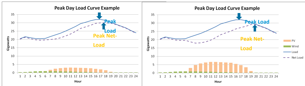
Figure 1. Potential shift in peak net-load within a day
