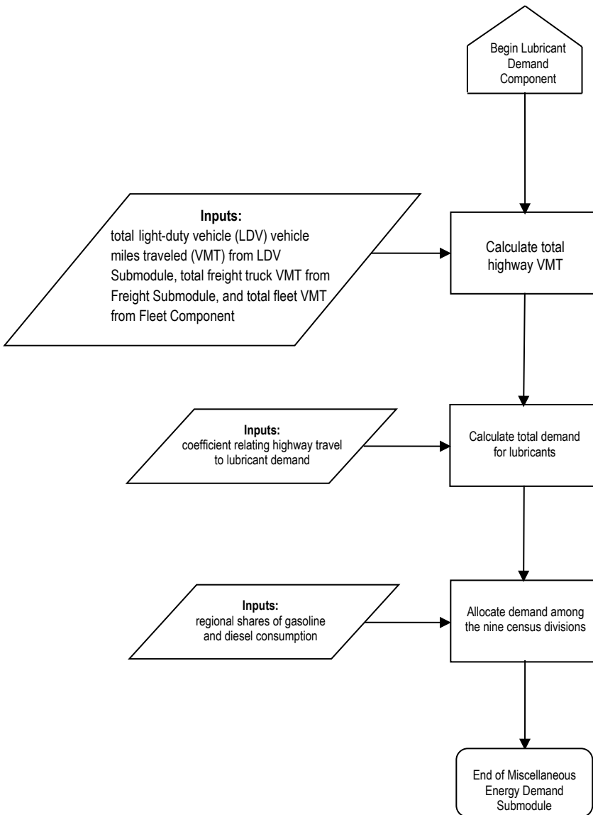
Figure 21. Lubricant Demand Component
