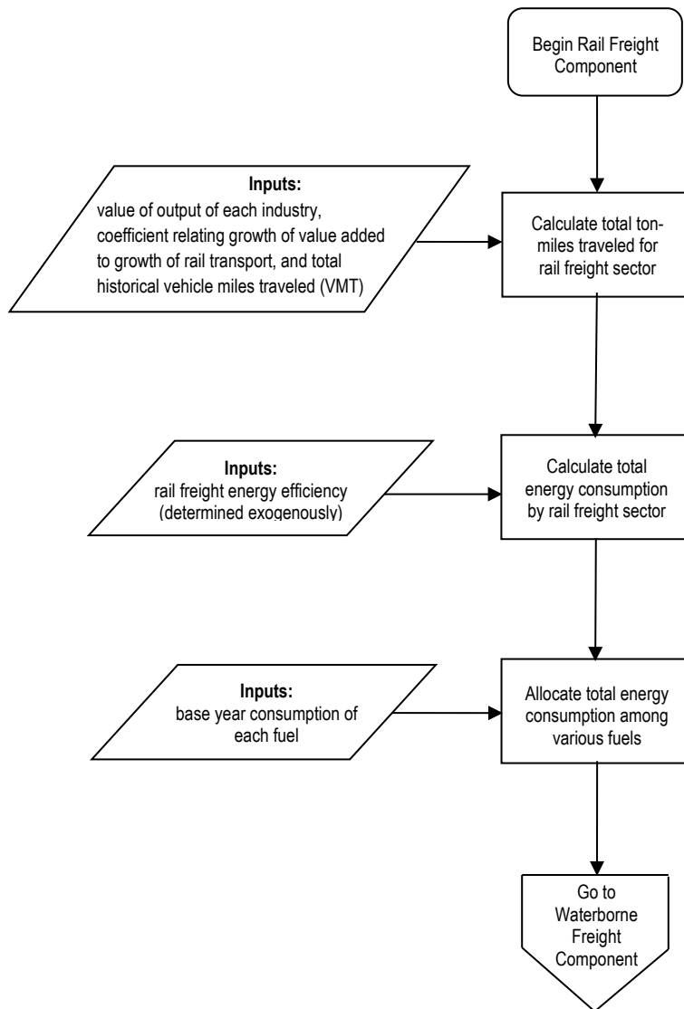
Figure 15. Rail Freight Component
