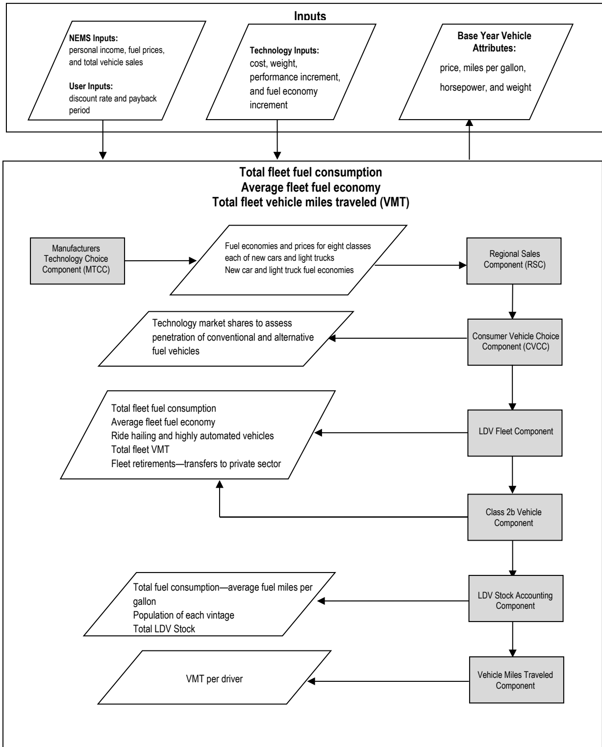
Figure 2. Structure of the Light-Duty Vehicle (LDV) Submodule
