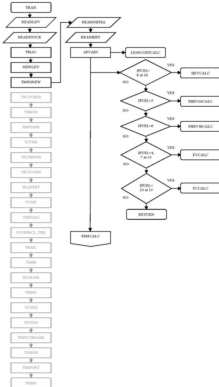
Figure 22. Flowchart of calls made by TRAN subroutine
