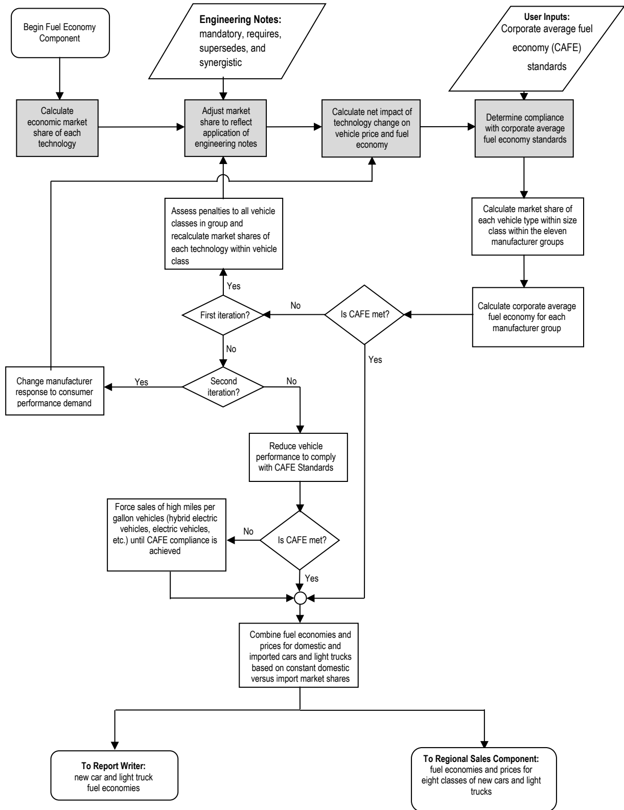
Figure 3. Manufacturers Technology Choice Component
