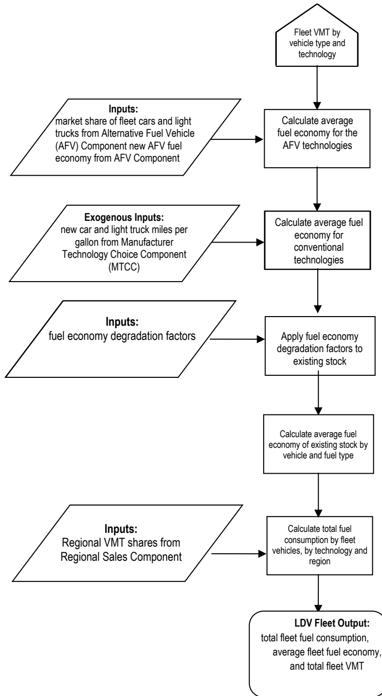
Figure 10. Determine fuel economy and consumption for light-duty vehicle (LDV) fleets
