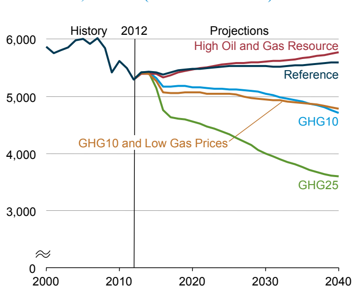
Figure ES-7. Energy-related carbon dioxide emissions in five cases, 2000-40 (million metric tons)
