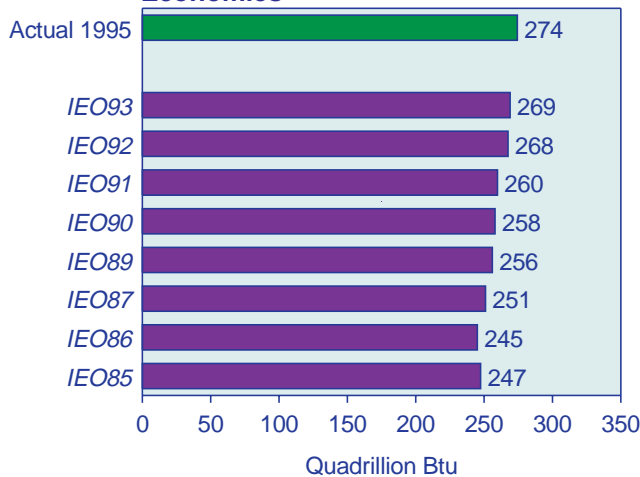
Figure F2. Comparison of IEO Forecasts with 1995 Energy Consumption in Market Economies
