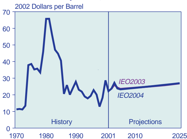
Figure 4. Comparison of 2003 and 2004 World Oil Price Projections, 1970-2025
