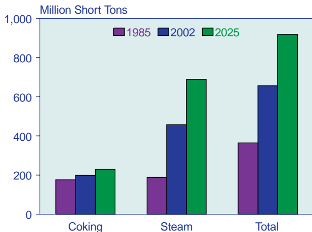
Figure 57. World Coal Trade, 1985, 2002, and 2025
