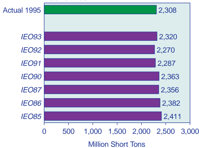
Figure F5. Comparison of IEO Forecasts with 1995 Coal Consumption in Market Economies
