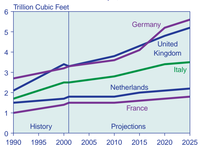
Figure 44. Natural Gas Consumption in Countries of Western Europe, 1990-2025
