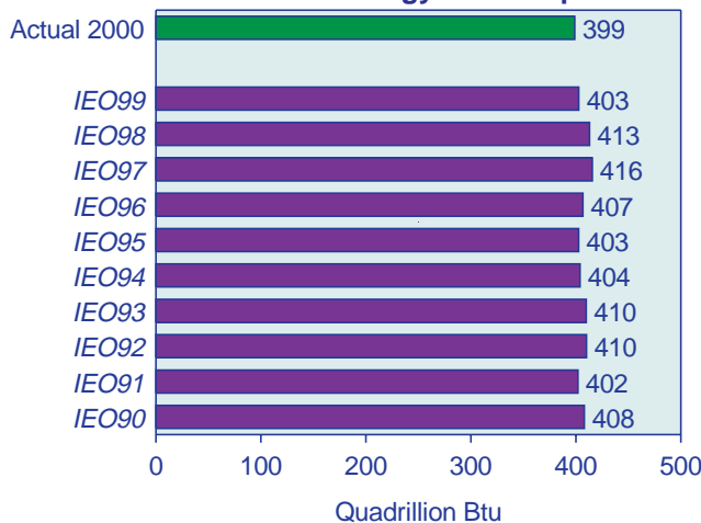
Figure F10. Comparison of IEO Forecasts with 2000 World Energy Consumption
