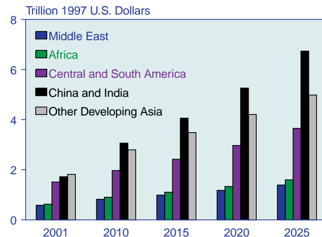
Figure 22. Developing World Gross Domestic Product by Region, 2001-2025
