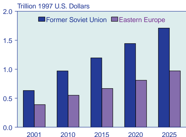
Figure 21. EE/FSU Gross Domestic Product by Region, 2001-2025
