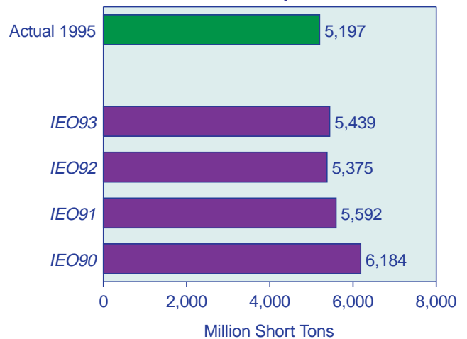
Figure F7. Comparison of IEO Forecasts with 1995 World Coal Consumption
