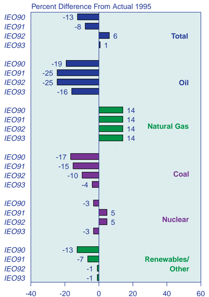
Figure F9. Comparison of IEO Forecasts with 1995 Energy Consumption in China by Fuel Type
