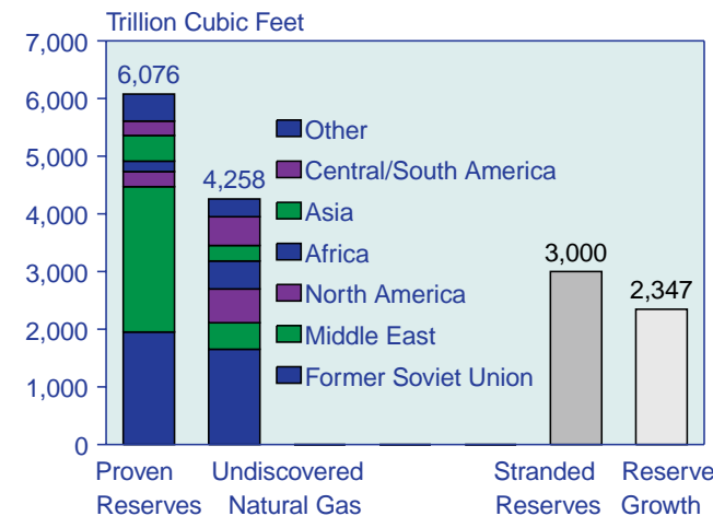
Figure 40. World Natural Gas Resources by Region as of January 1, 2004
