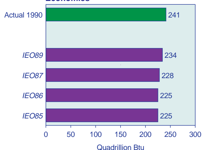
Figure F1. Comparison of IEO Forecasts with 1990 Energy Consumption in Market Economies
