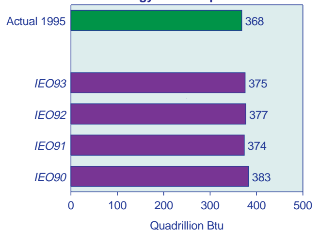
Figure F4. Comparison of IEO Forecasts with 1995 World Energy Consumption
