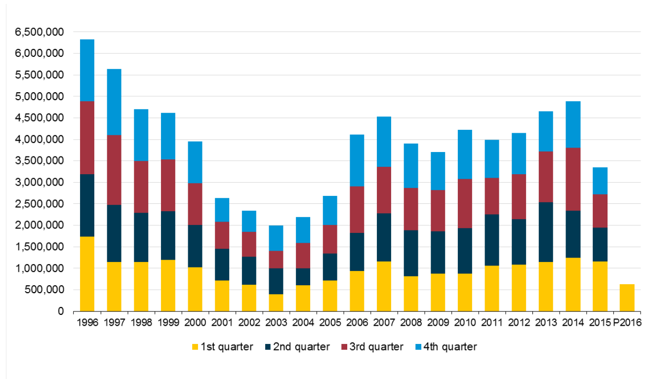
Figure 1. Uranium concentrate production in the United States, 1996 – 1st Quarter 2016
