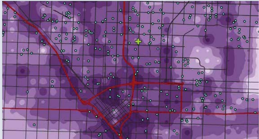
Distribution of PAHs in Fresno, California, based on extensive sampling. Darker areas reflect higher levels of PAHs. 32
